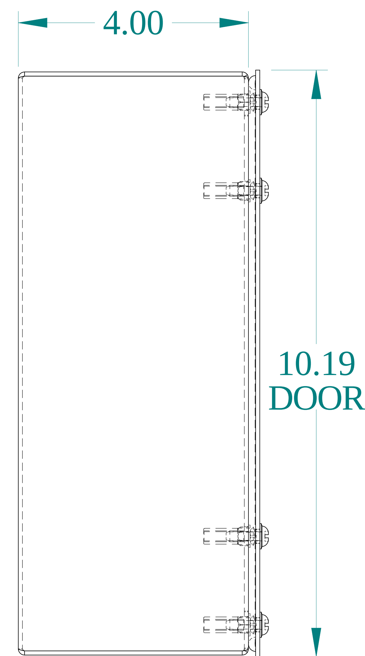
SIDE VIEW
