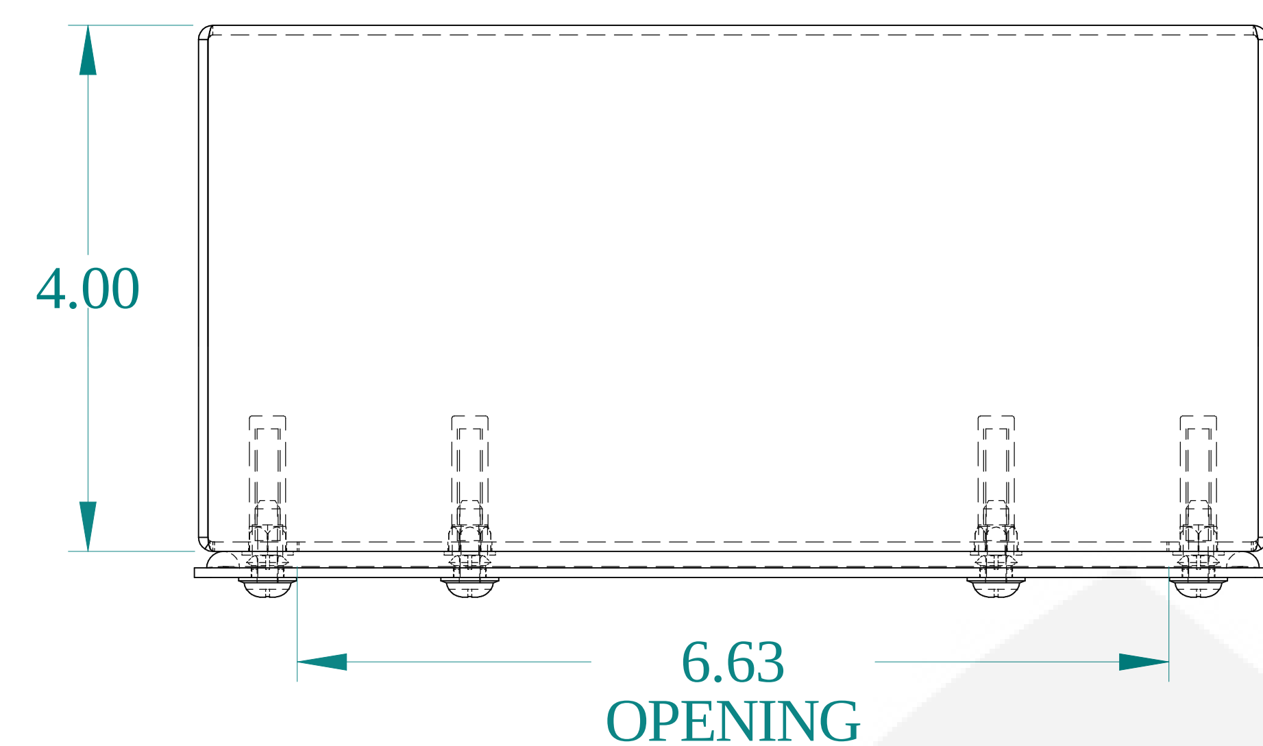
TOP VIEW
