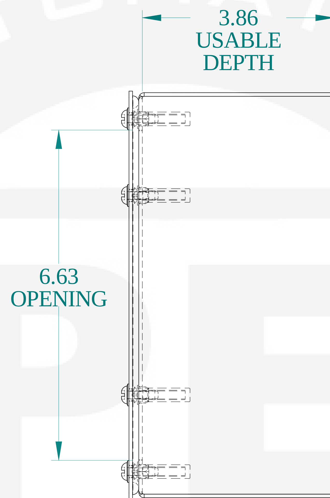
SIDE VIEW
