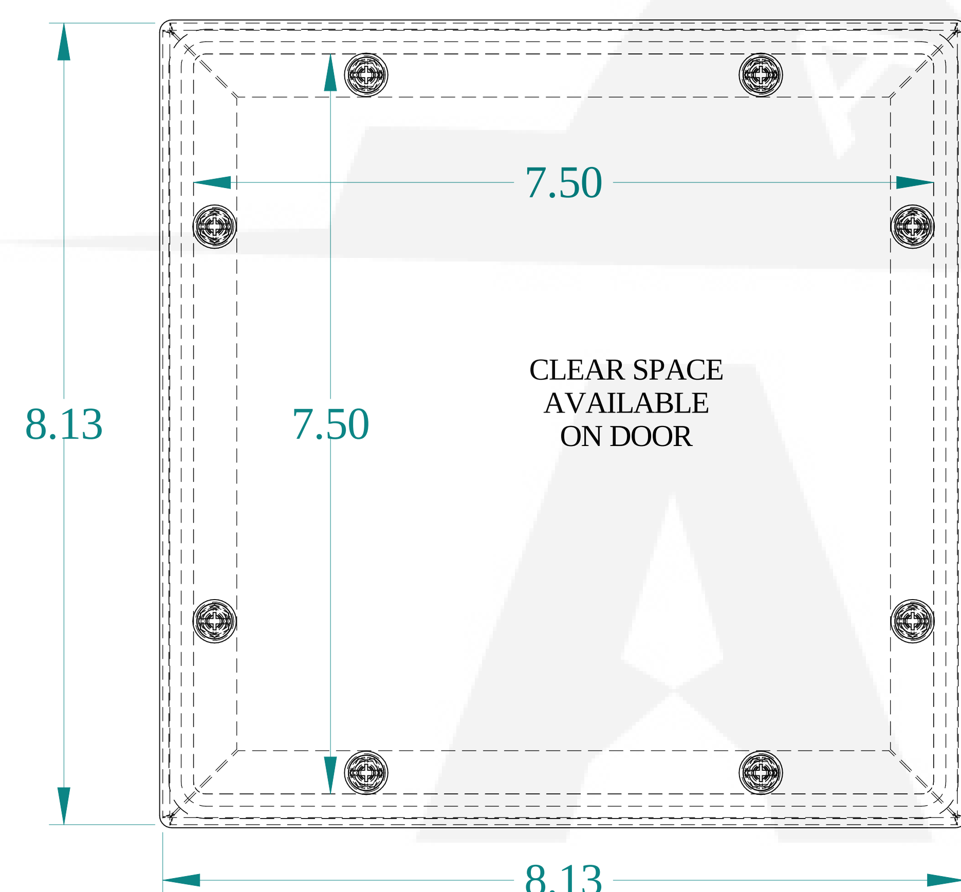
FRONT VIEW
