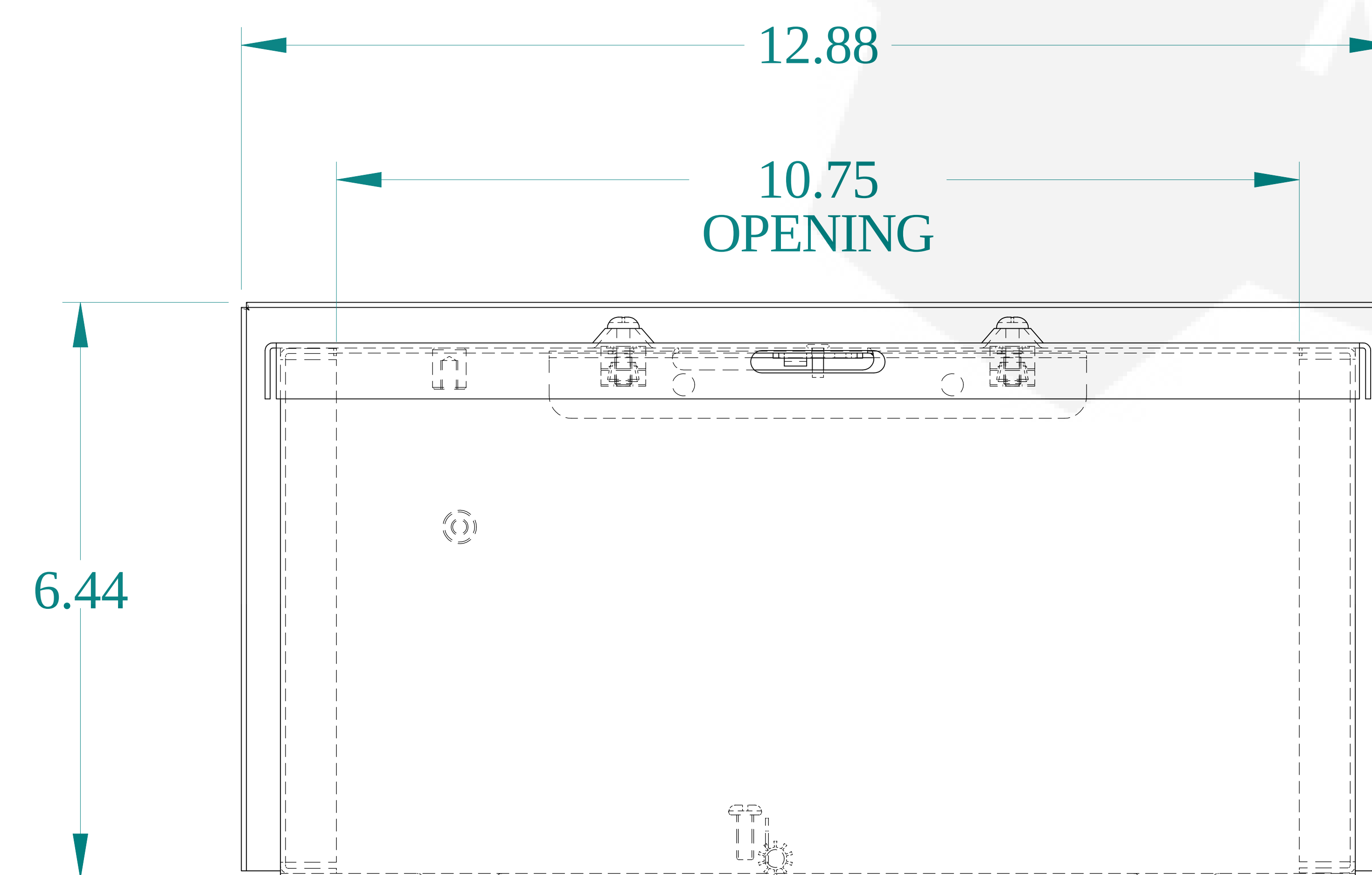
BOTTOM VIEW
