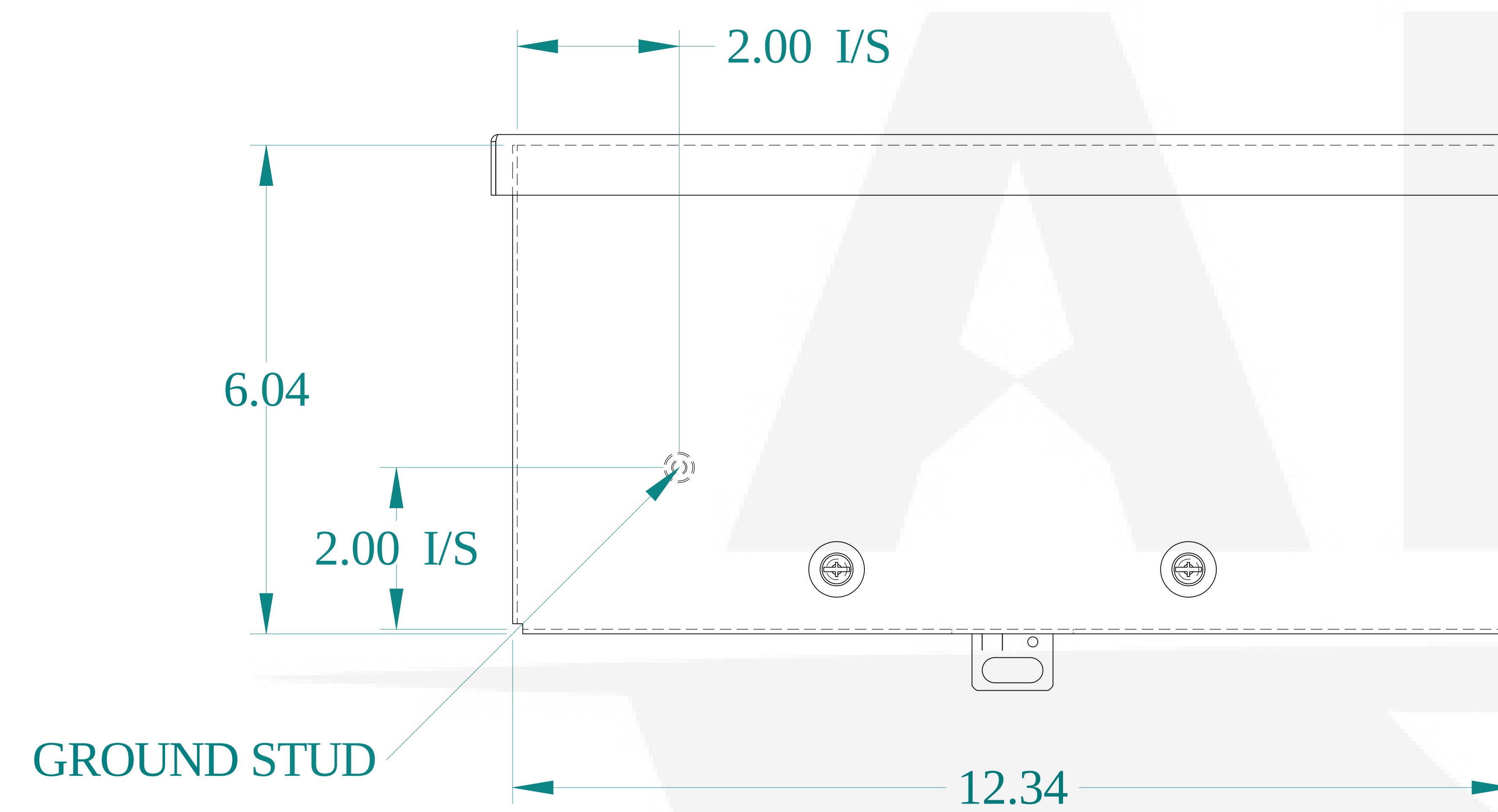
FRONT VIEW
