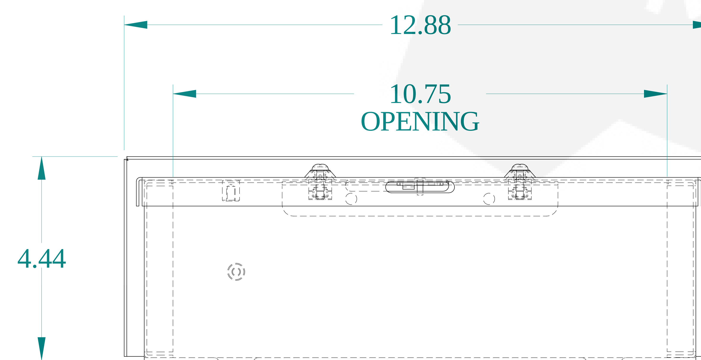
BOTTOM VIEW
