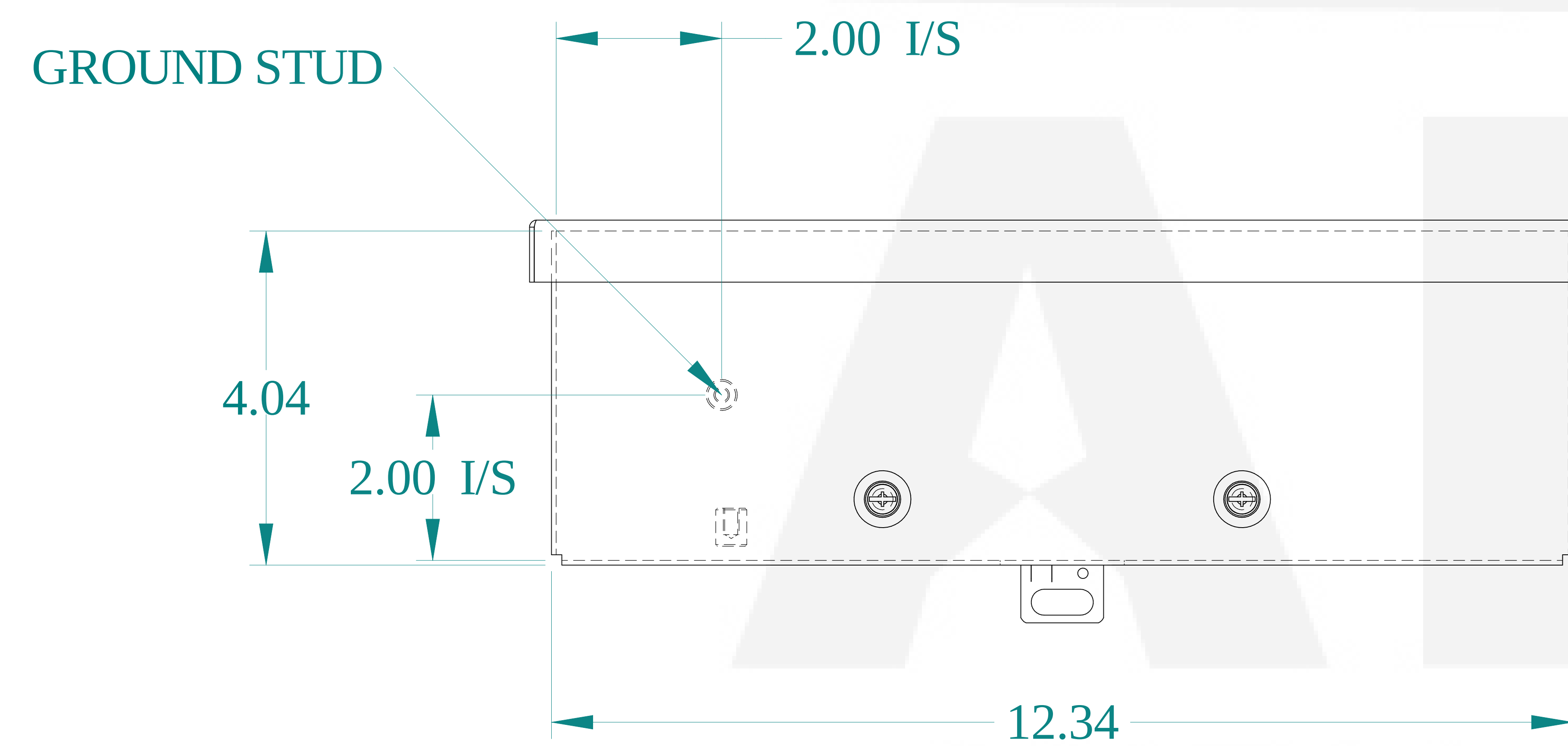
FRONT VIEW
