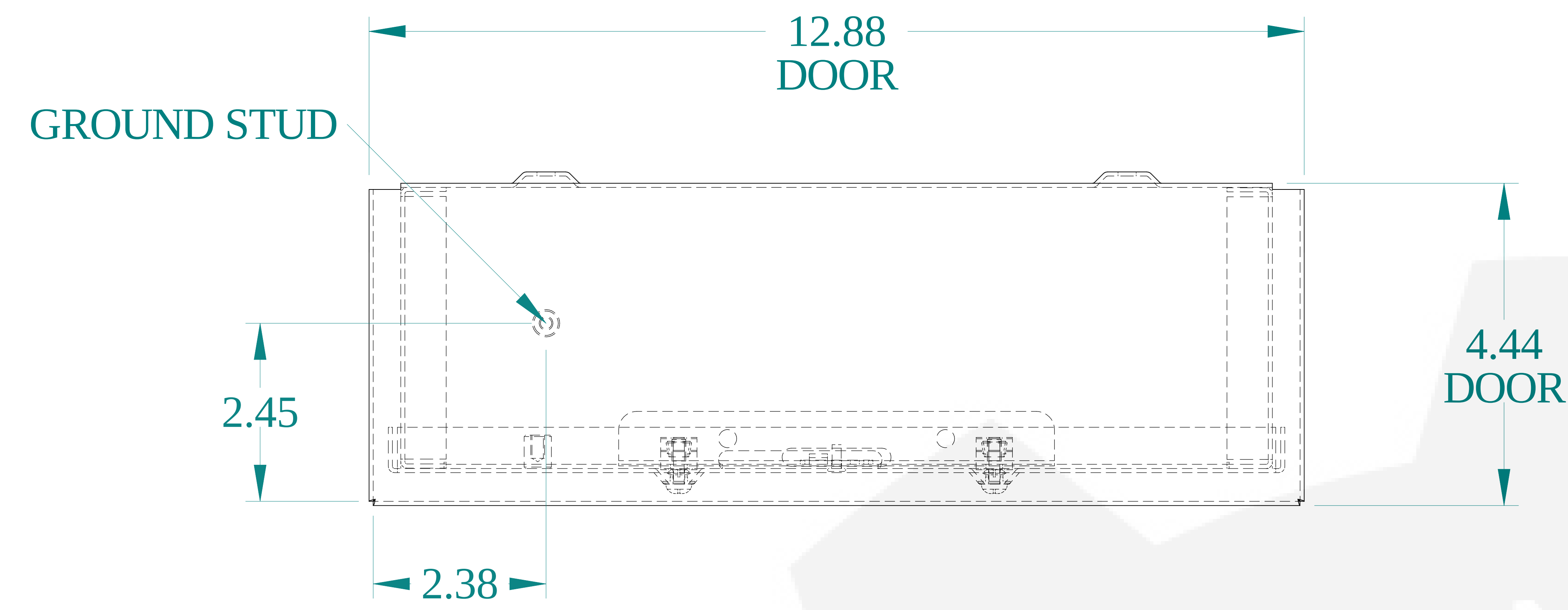
TOP VIEW
