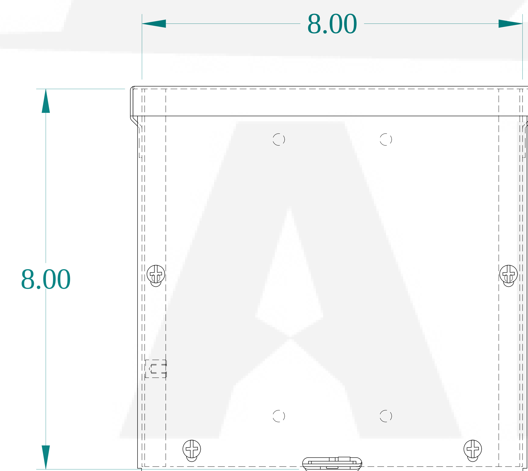
FRONT VIEW
