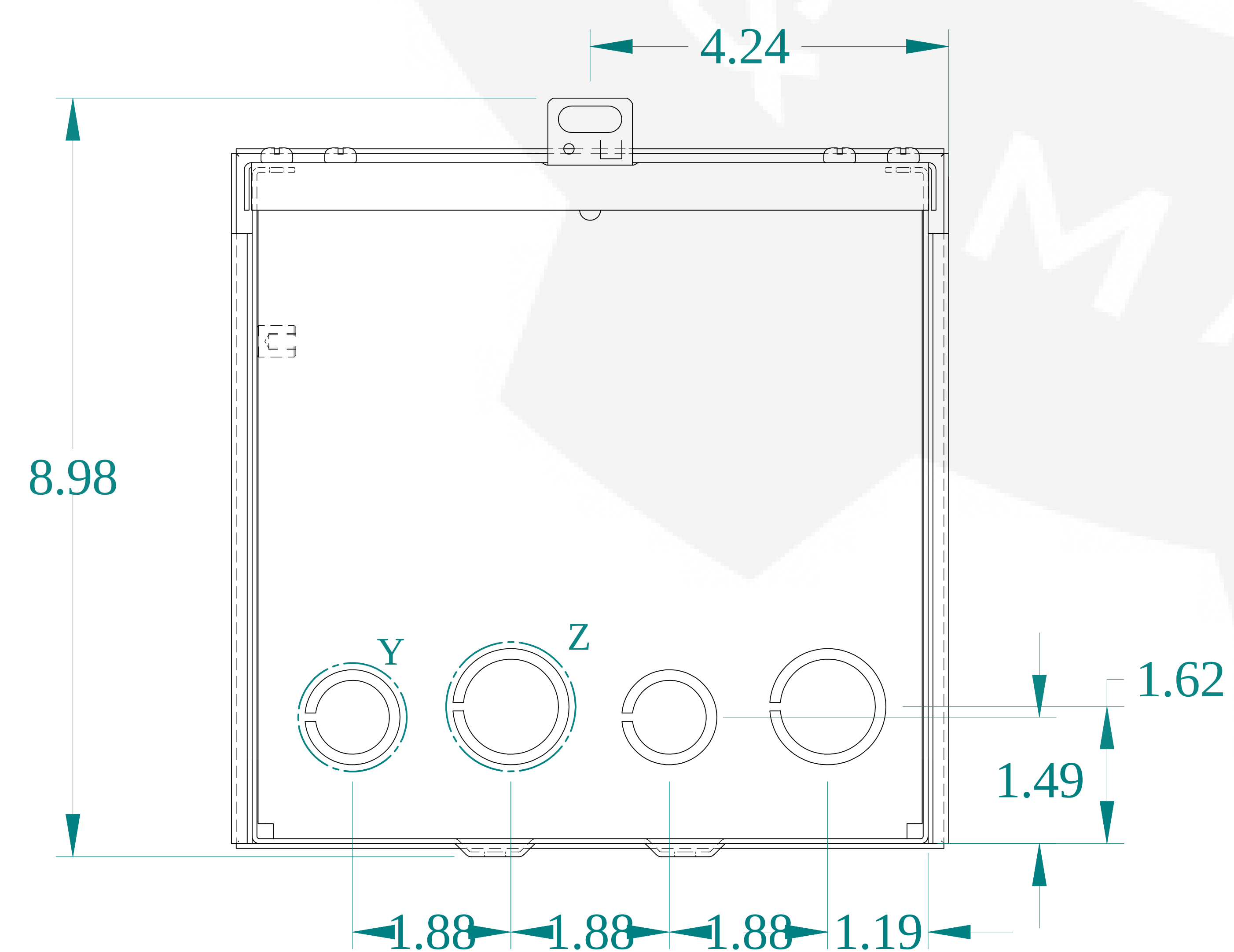
BOTTOM VIEW
