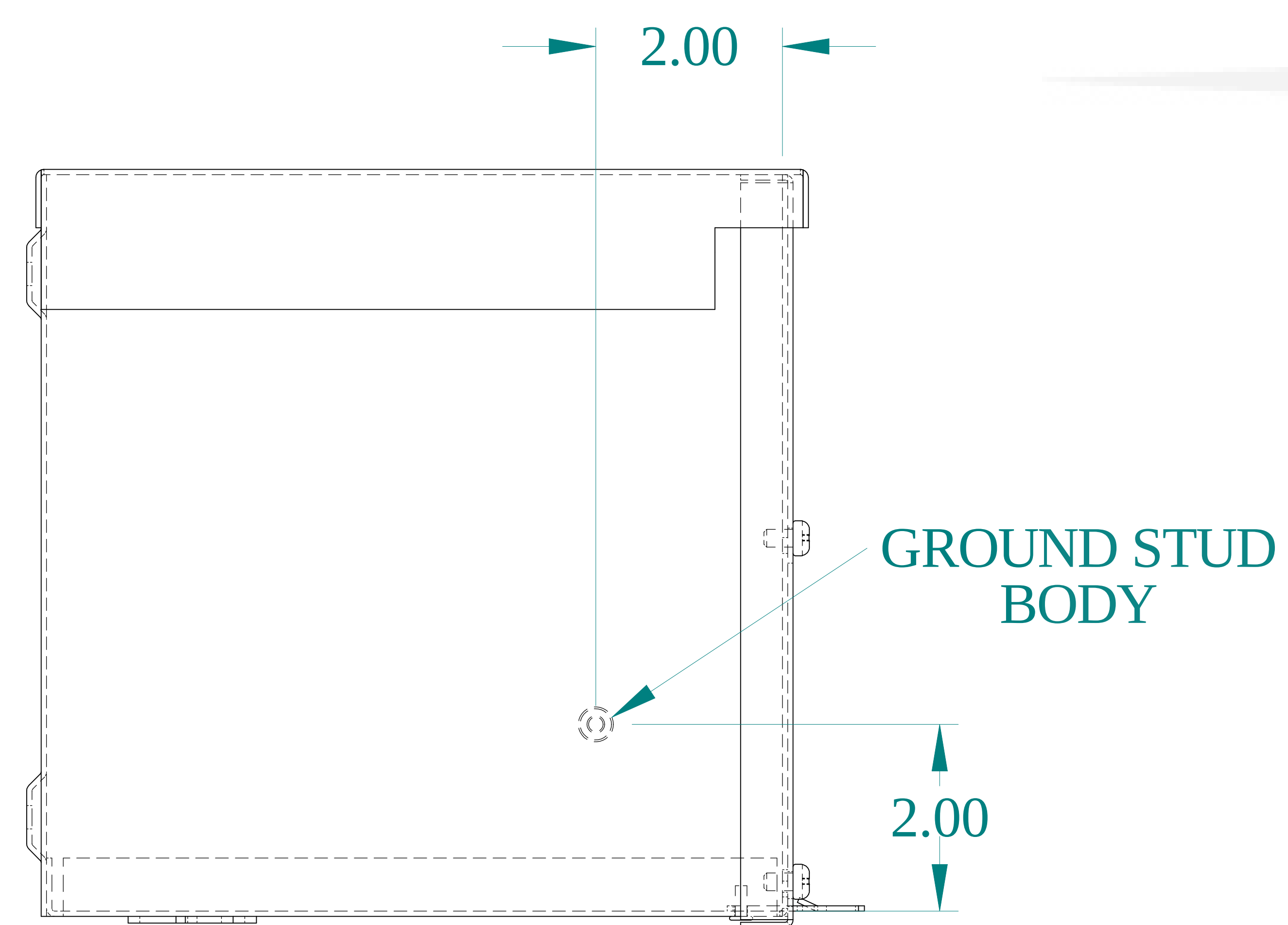
SIDE VIEW
