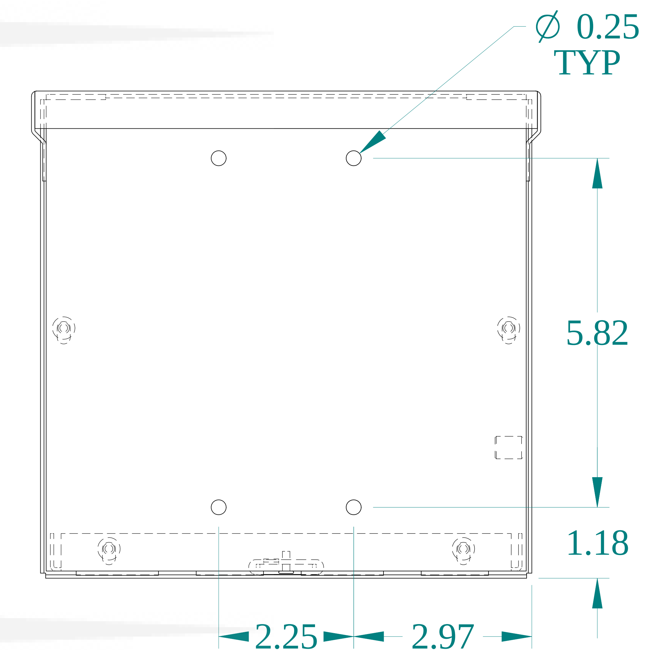
BACK VIEW
