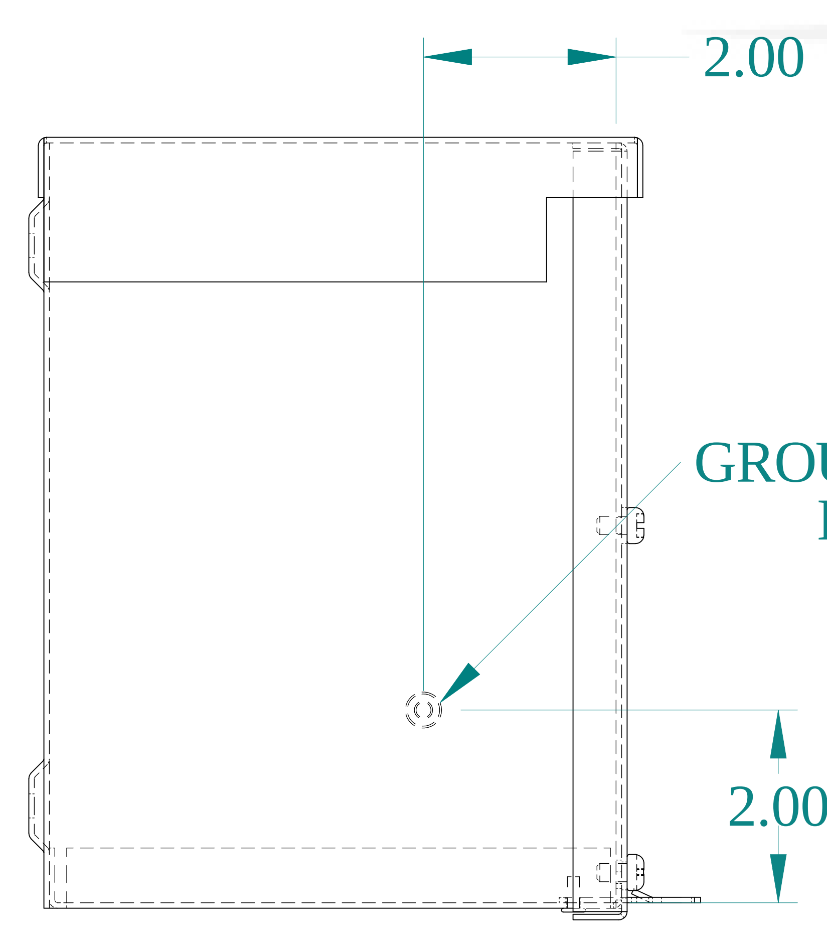
SIDE VIEW
