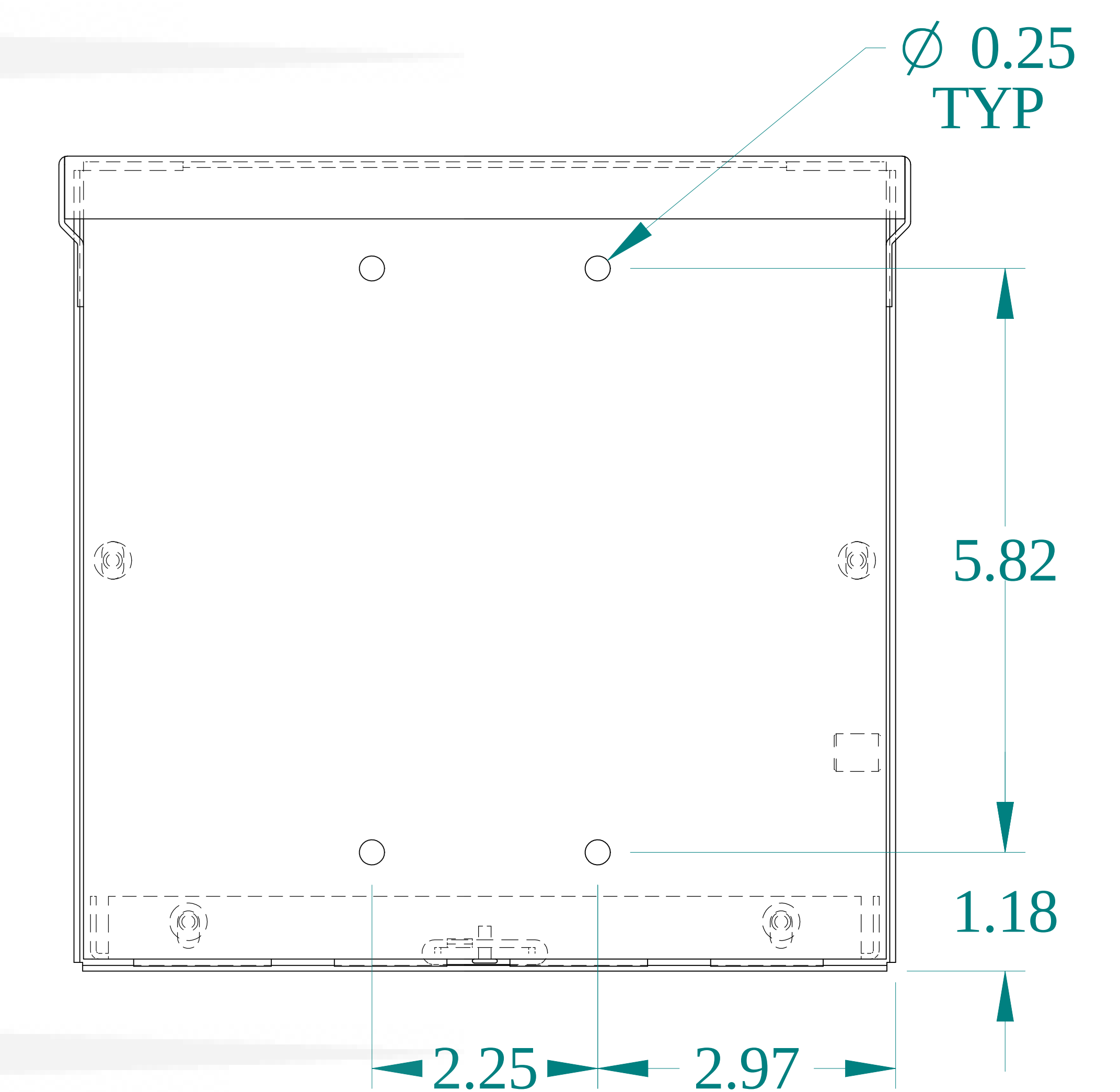
BACK VIEW
