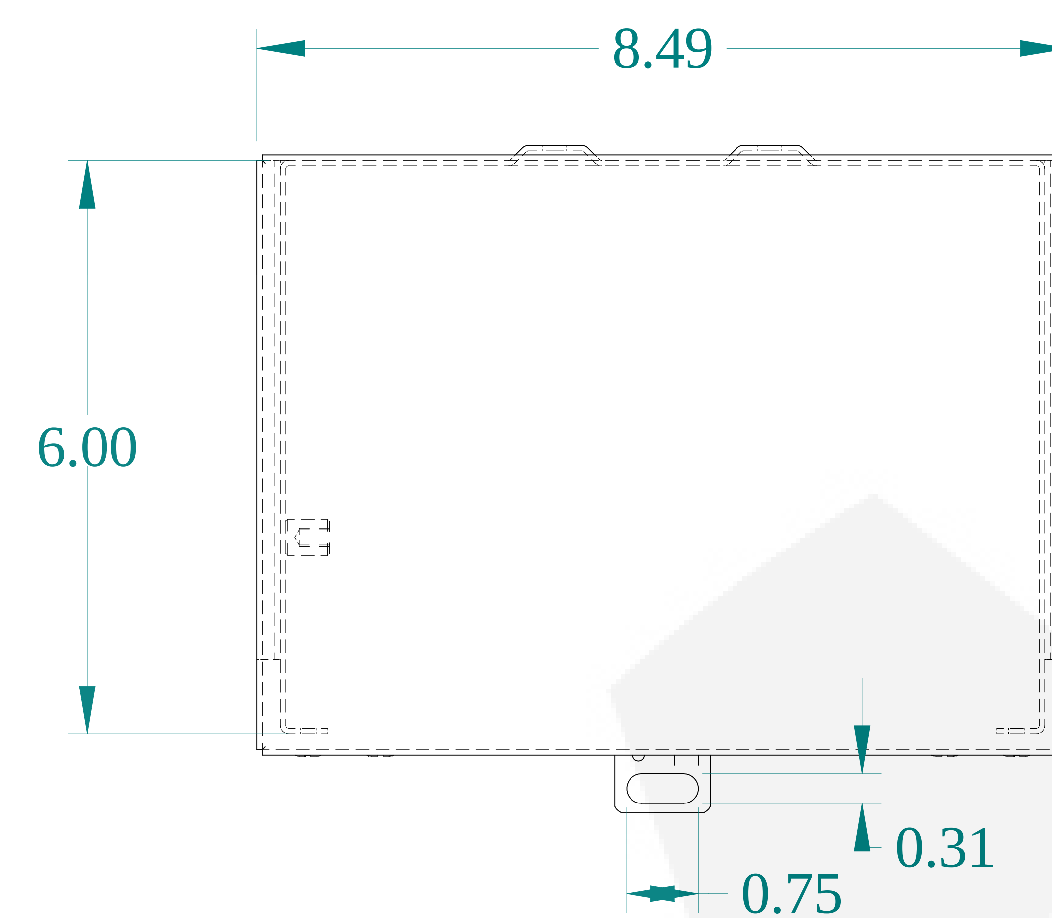
TOP VIEW
