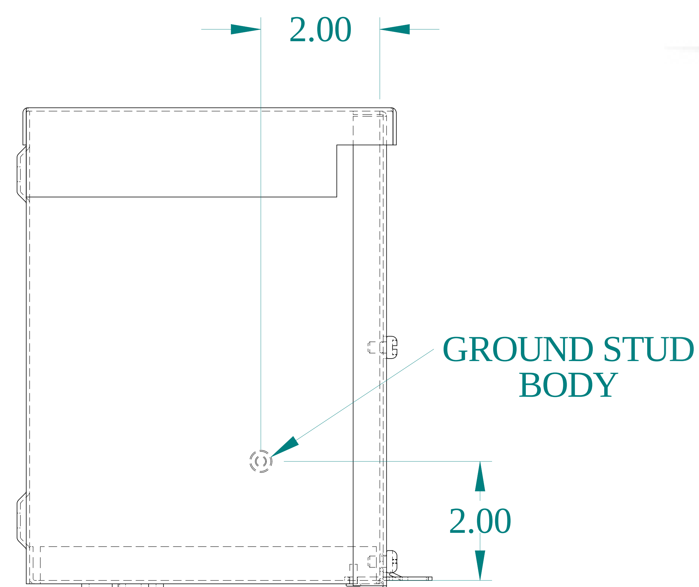
SIDE VIEW
