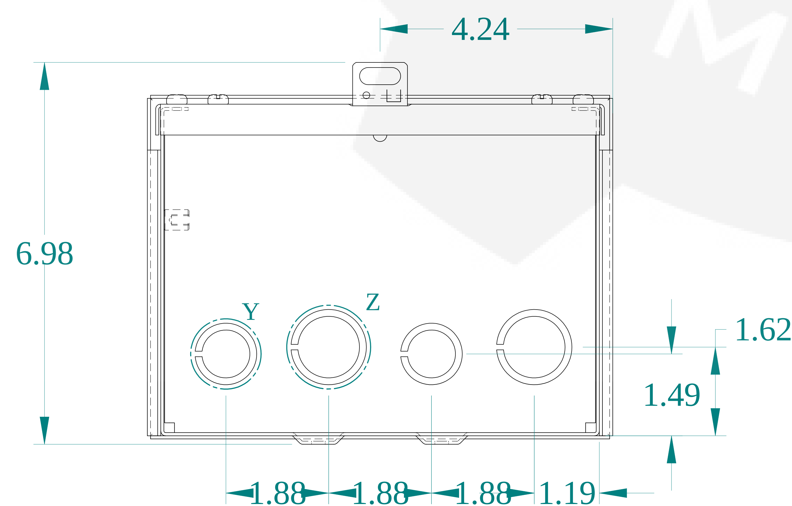
BOTTOM VIEW
