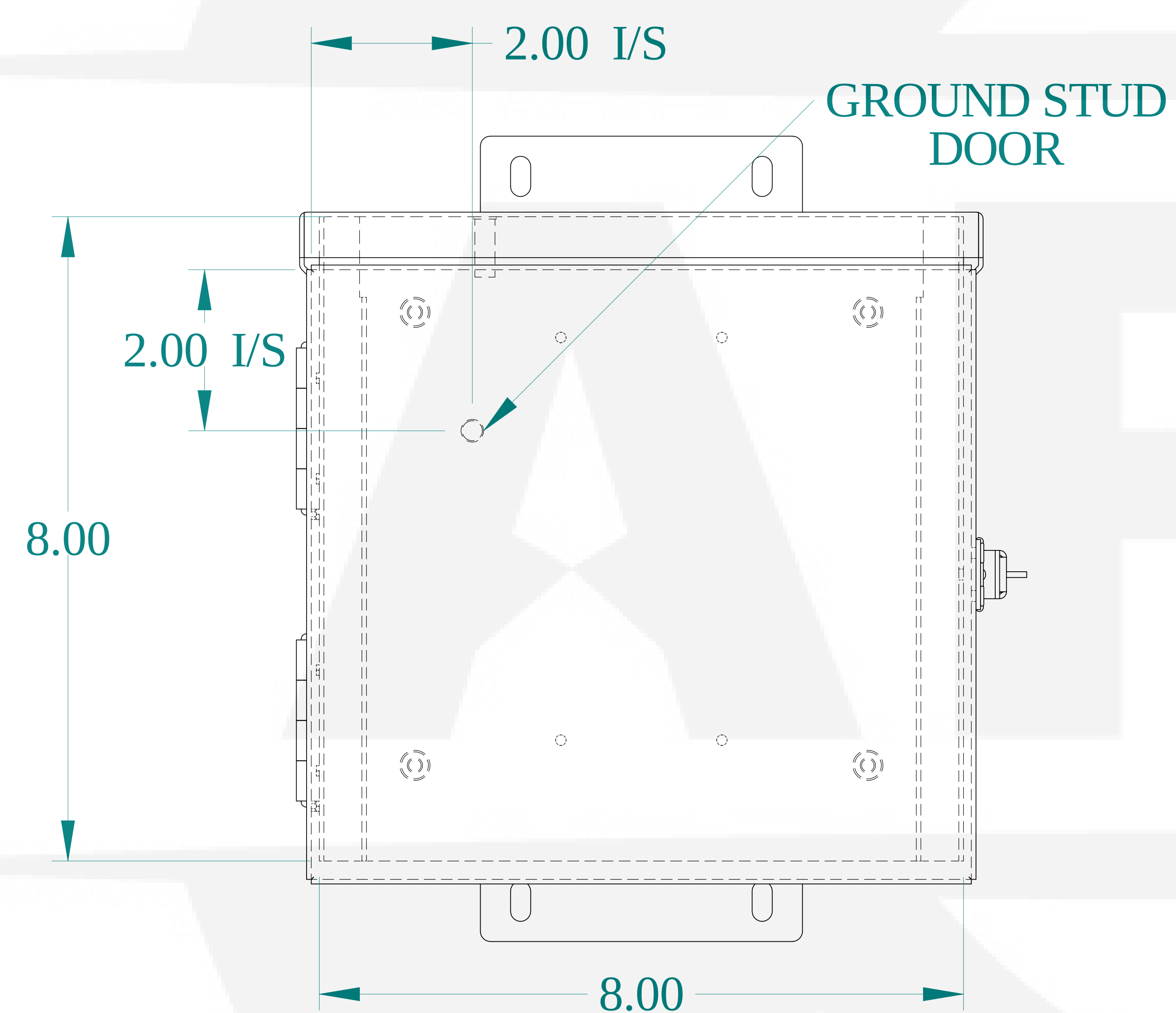
FRONT VIEW
