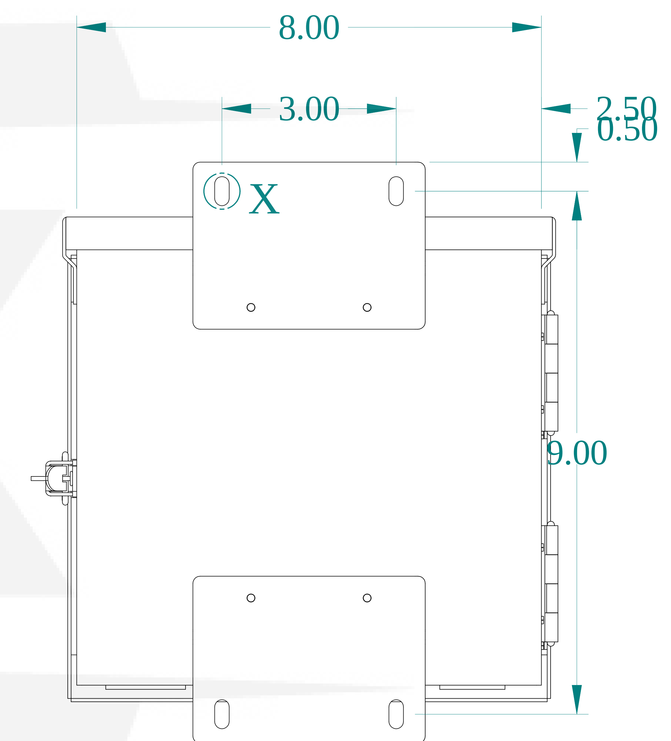
BACK VIEW
