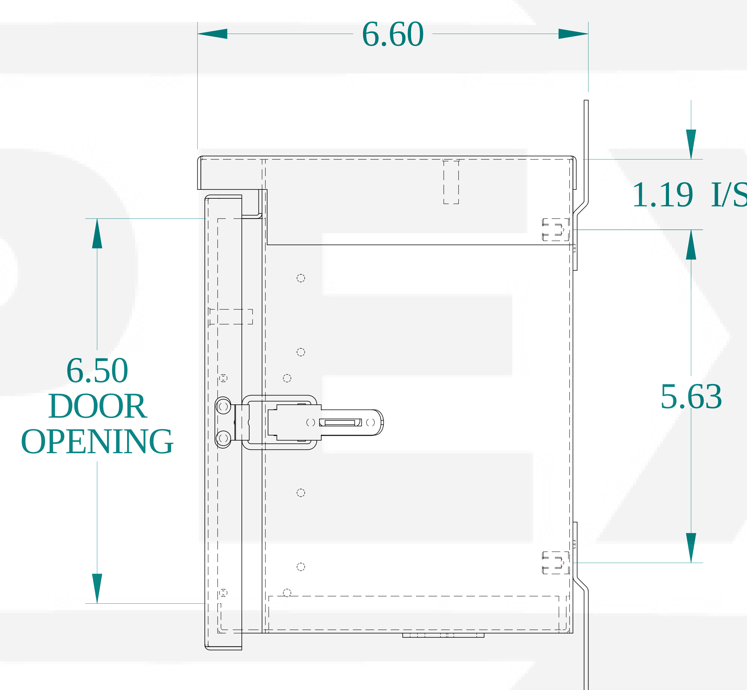
SIDE VIEW
