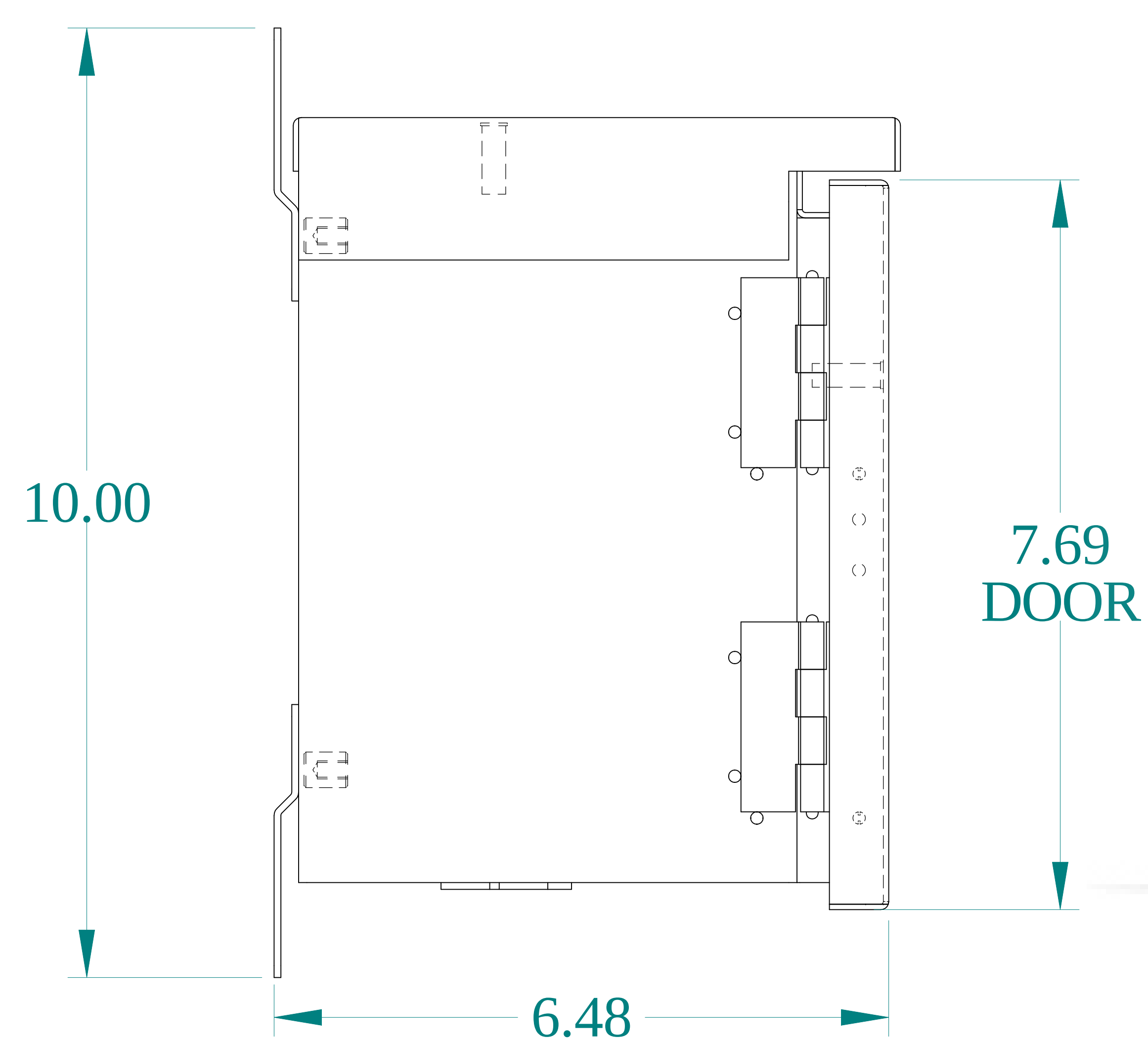
SIDE VIEW
