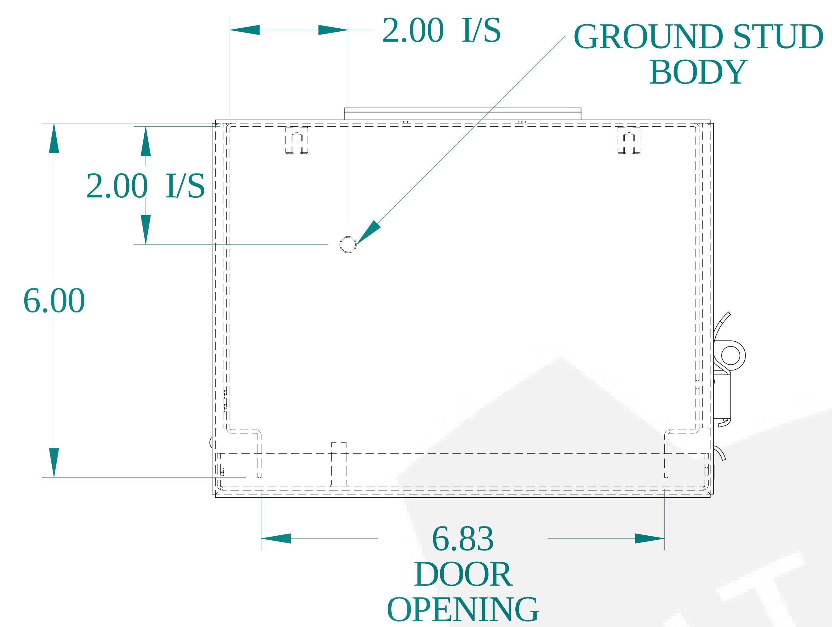
TOP VIEW
