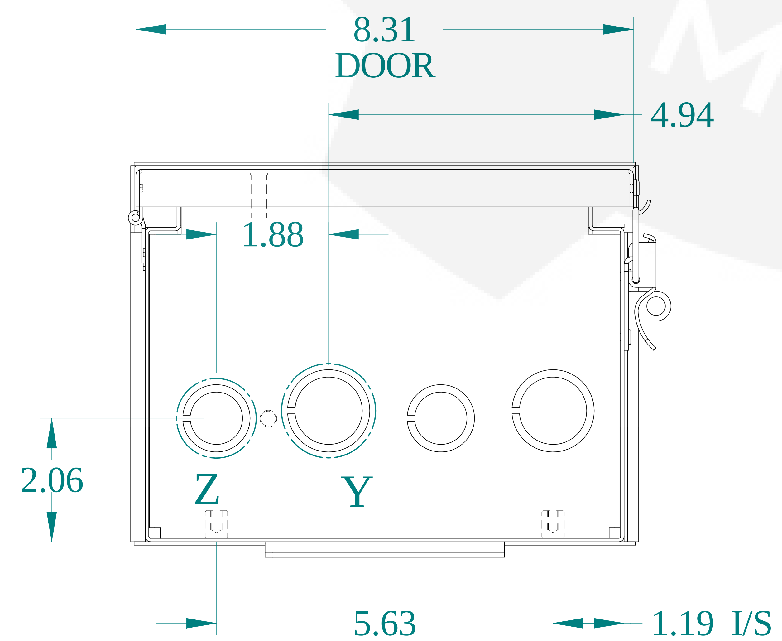
BOTTOM VIEW
