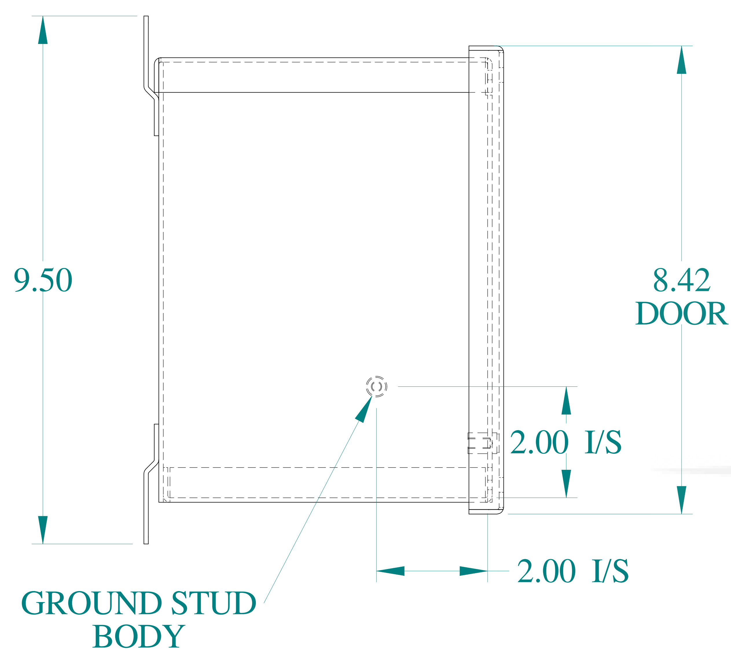
SIDE VIEW
