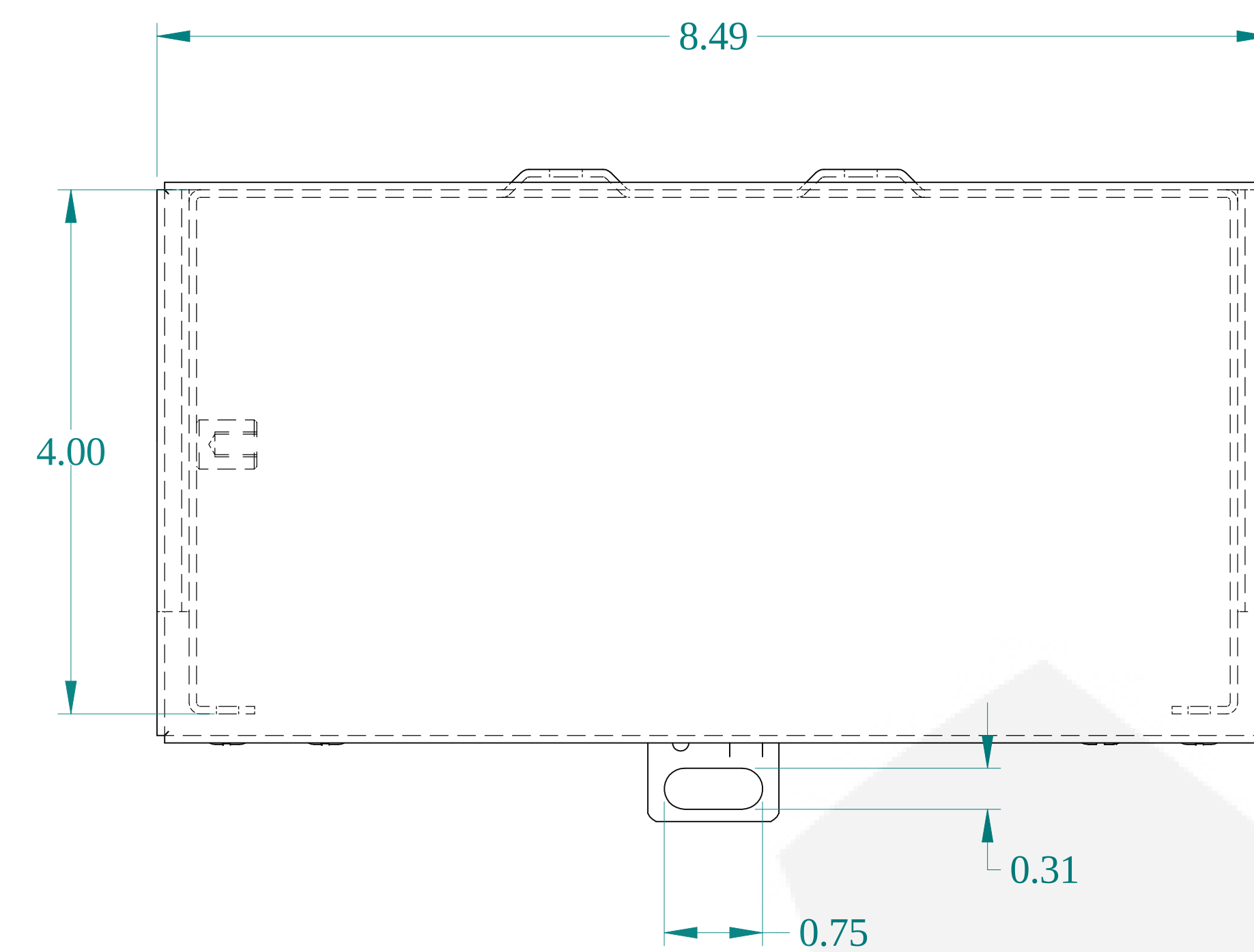
TOP VIEW
