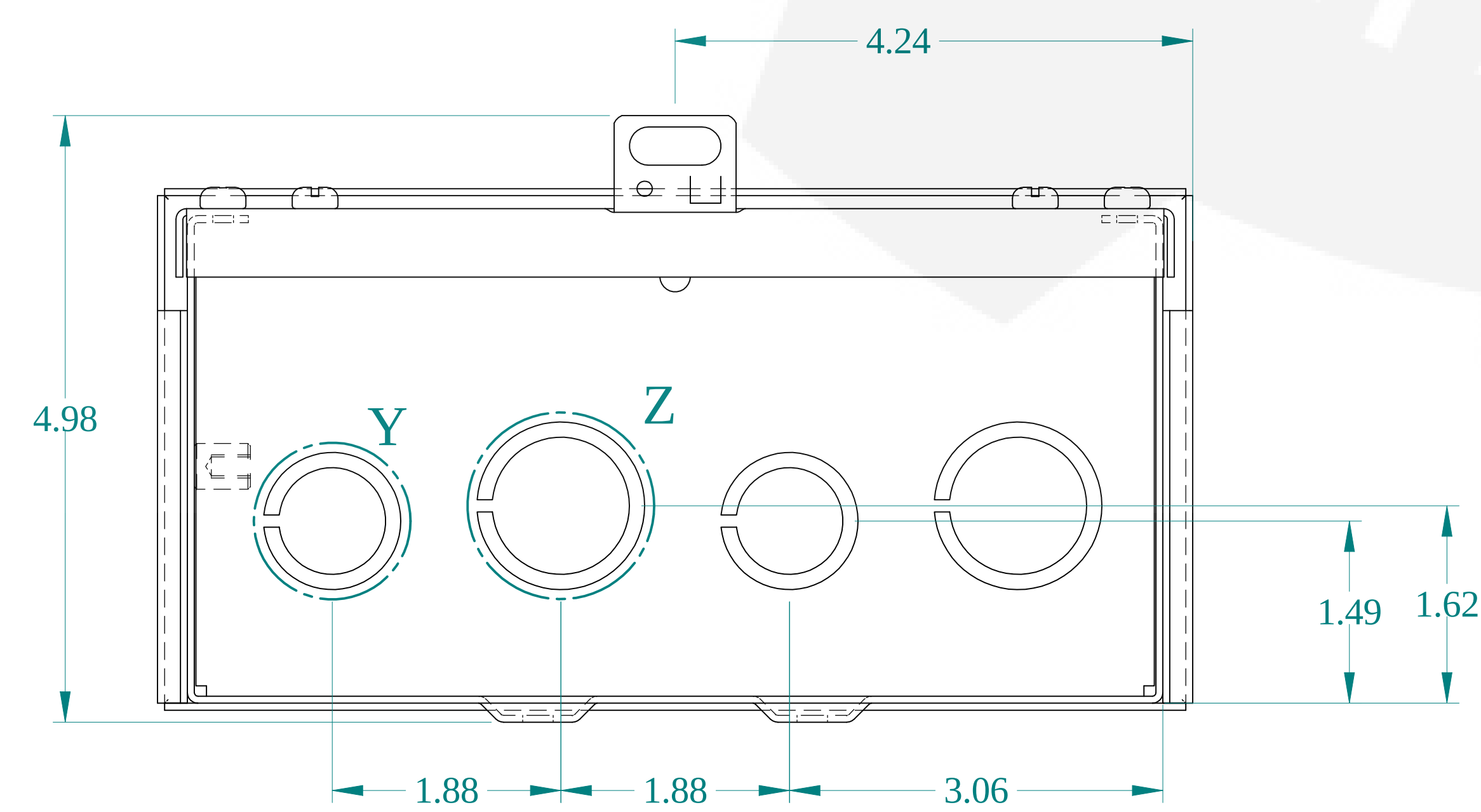
BOTTOM VIEW
