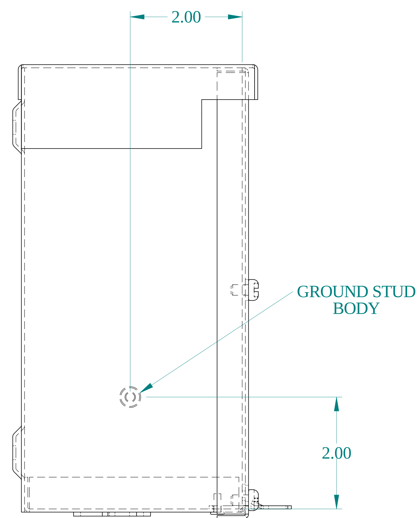
SIDE VIEW
