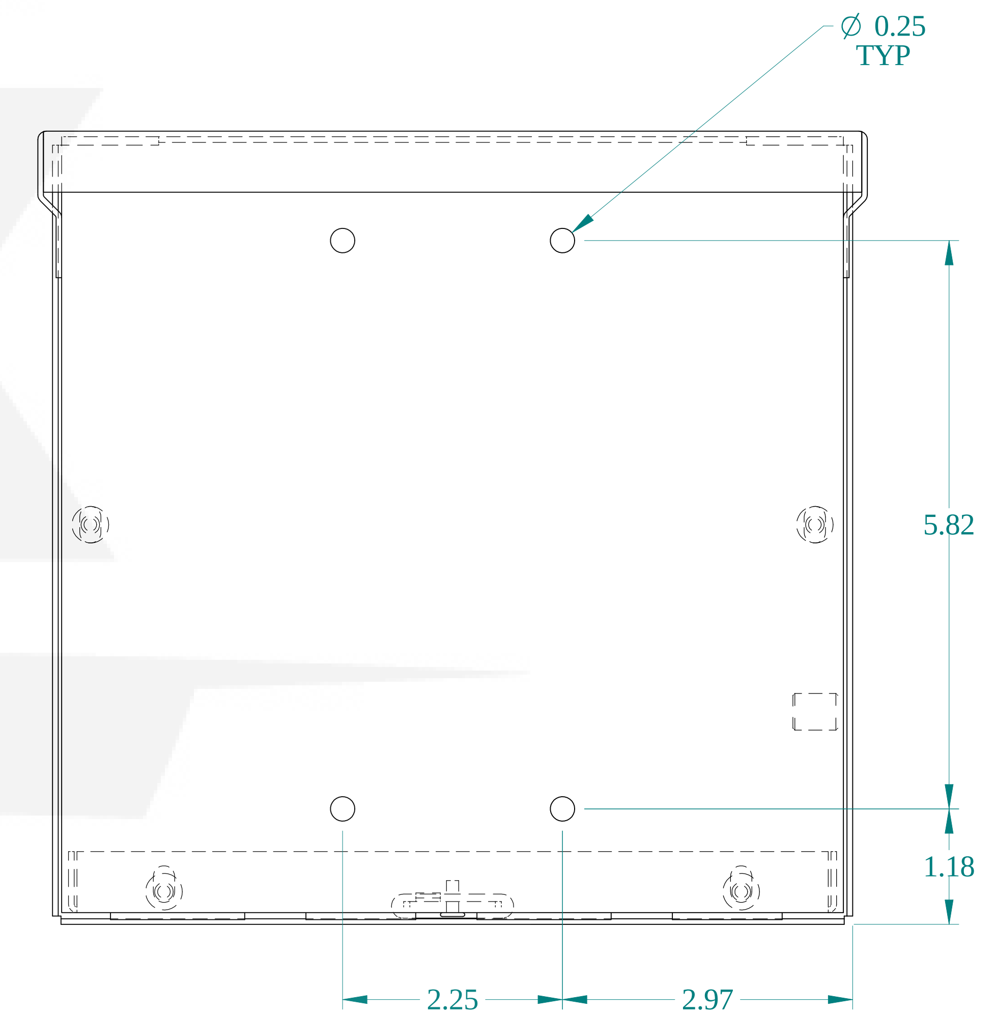
BACK VIEW
