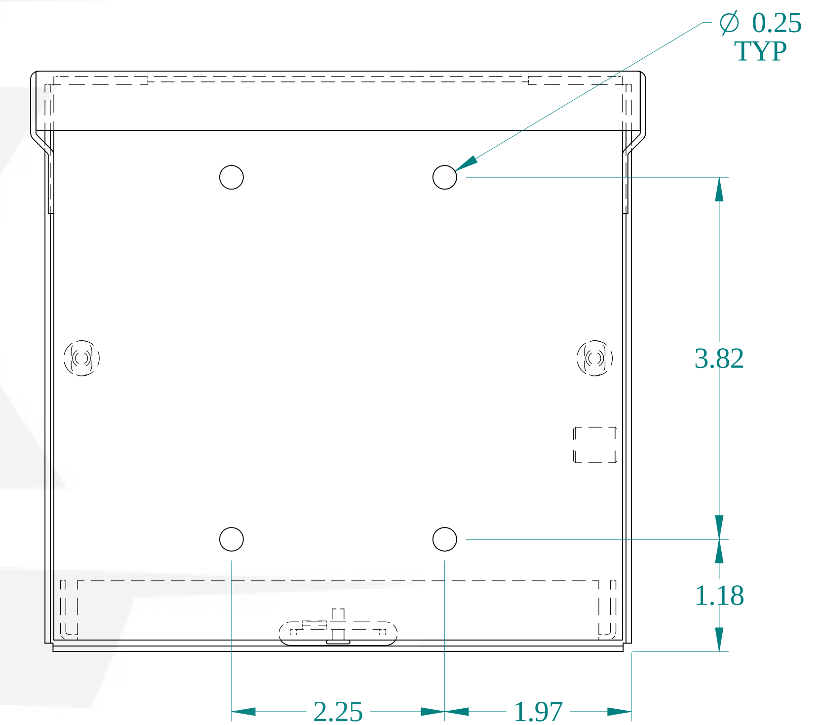
BACK VIEW
