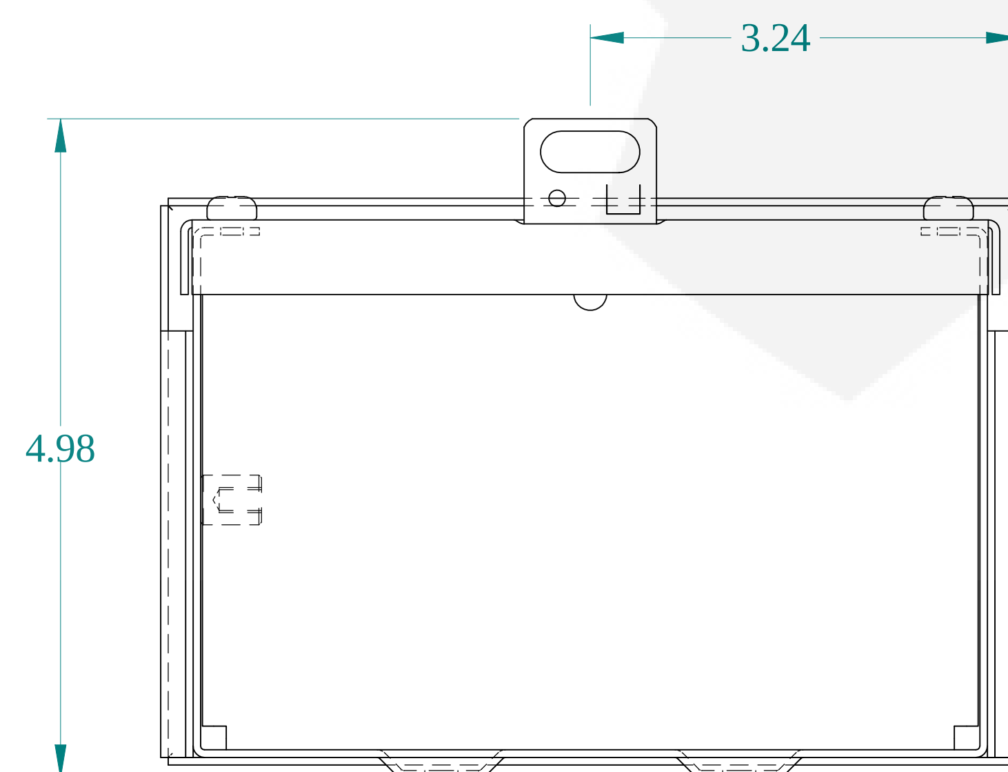
FRONT VIEW
