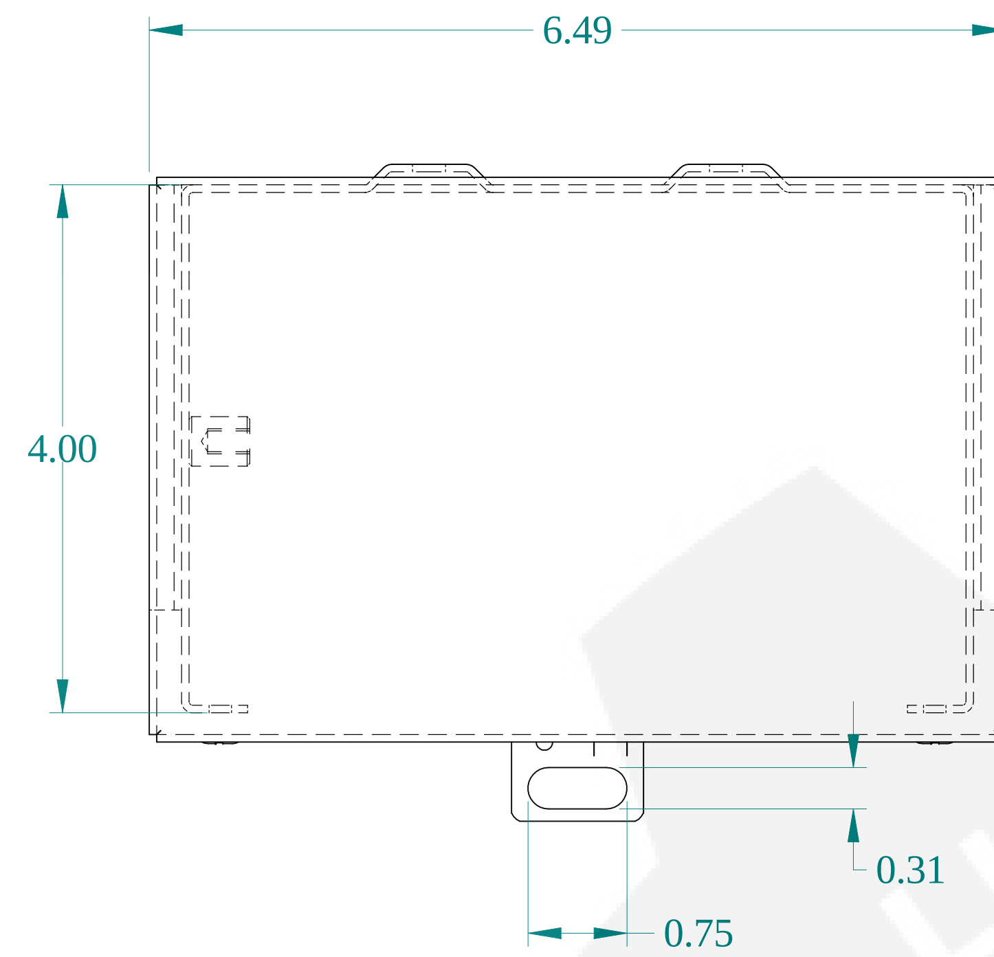
TOP VIEW
