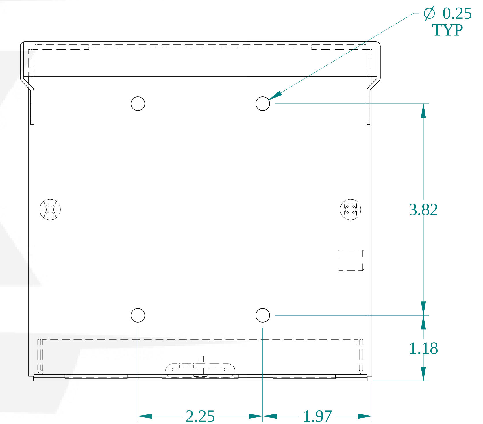
BACK VIEW
