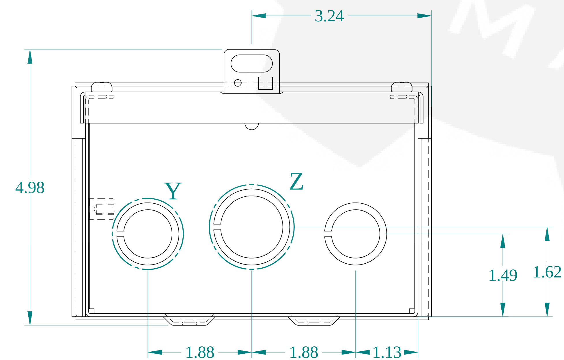
BOTTOM VIEW
