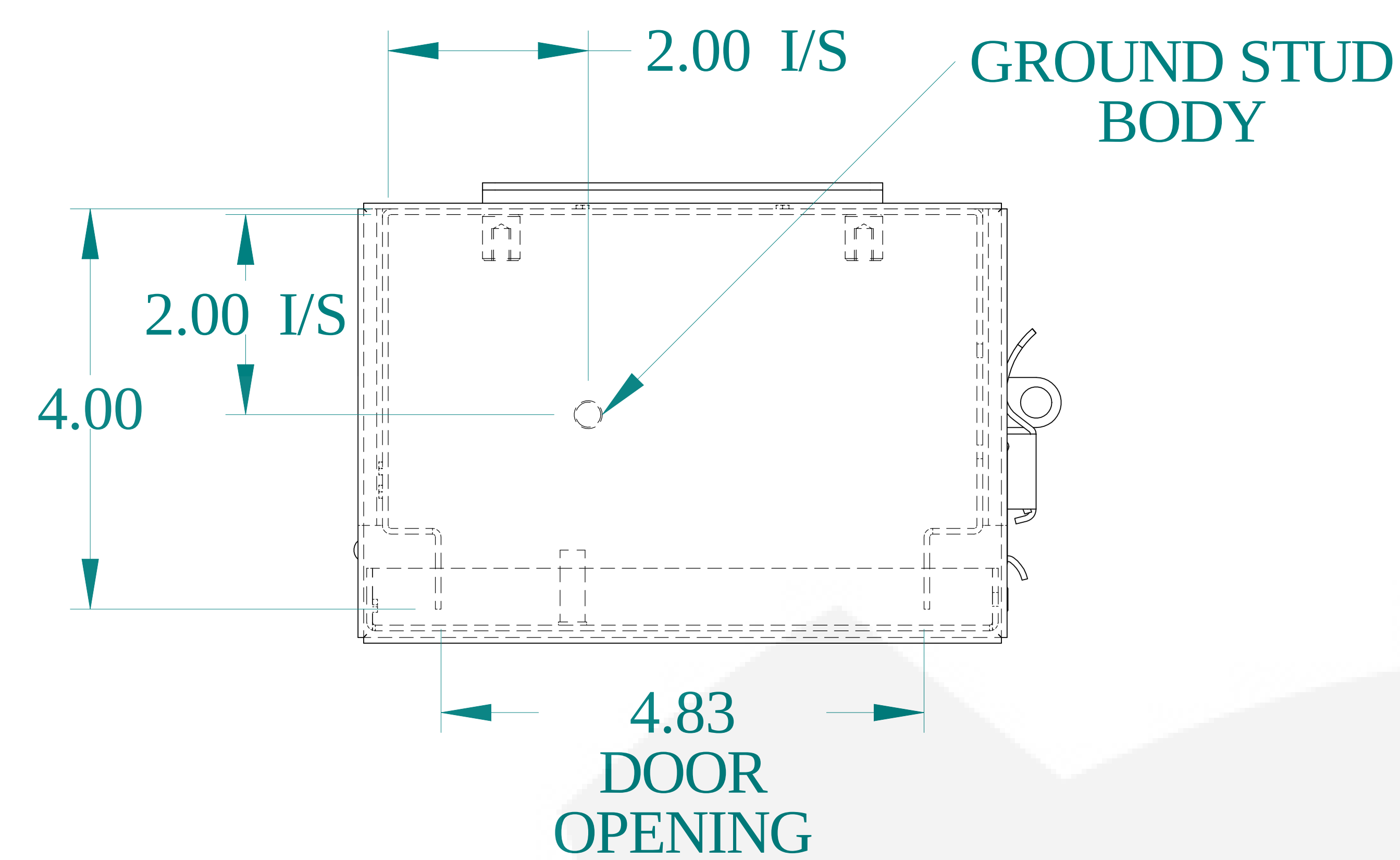
TOP VIEW
