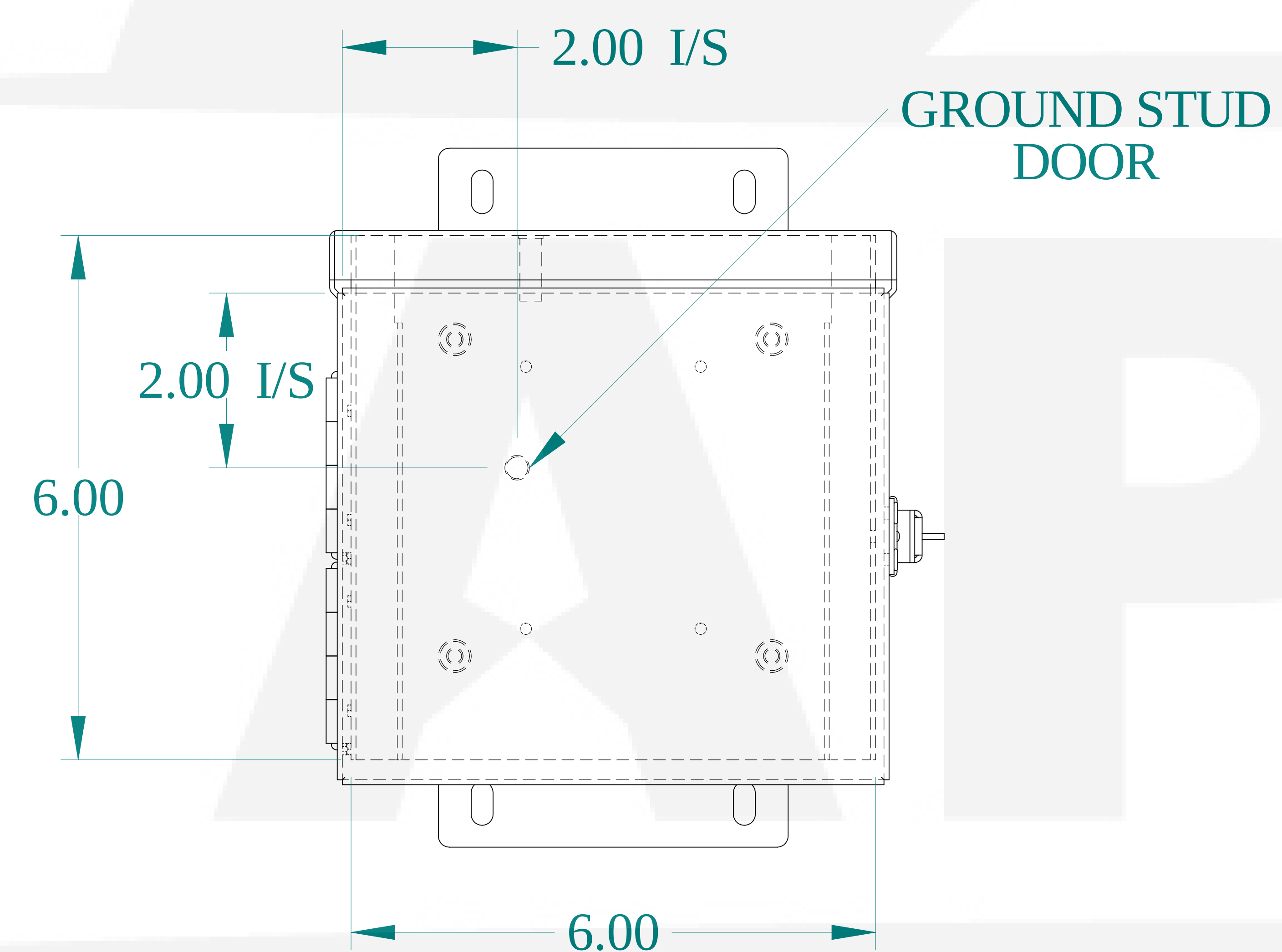
FRONT VIEW
