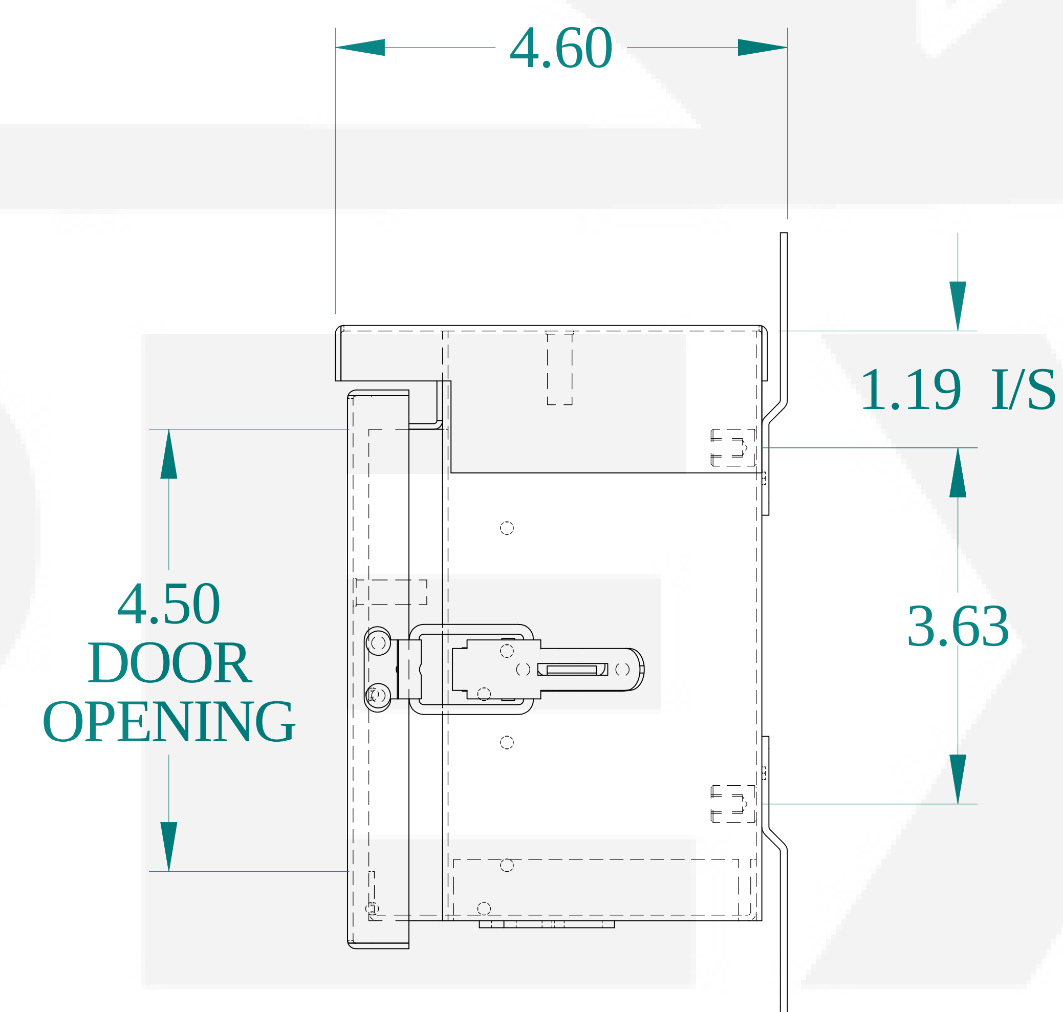
SIDE VIEW
