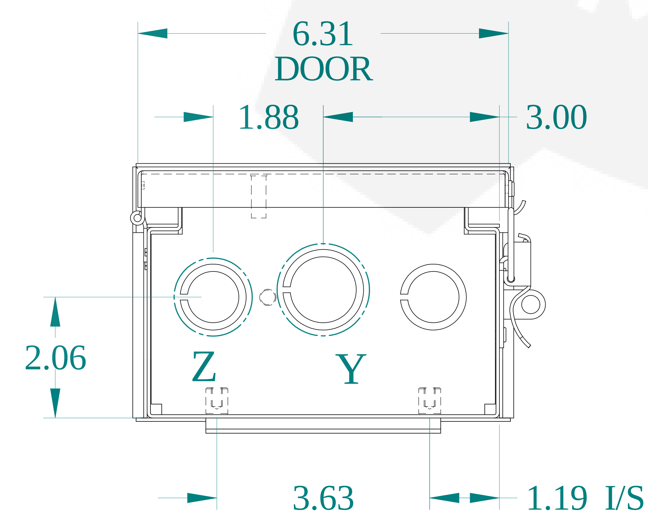
BOTTOM VIEW
