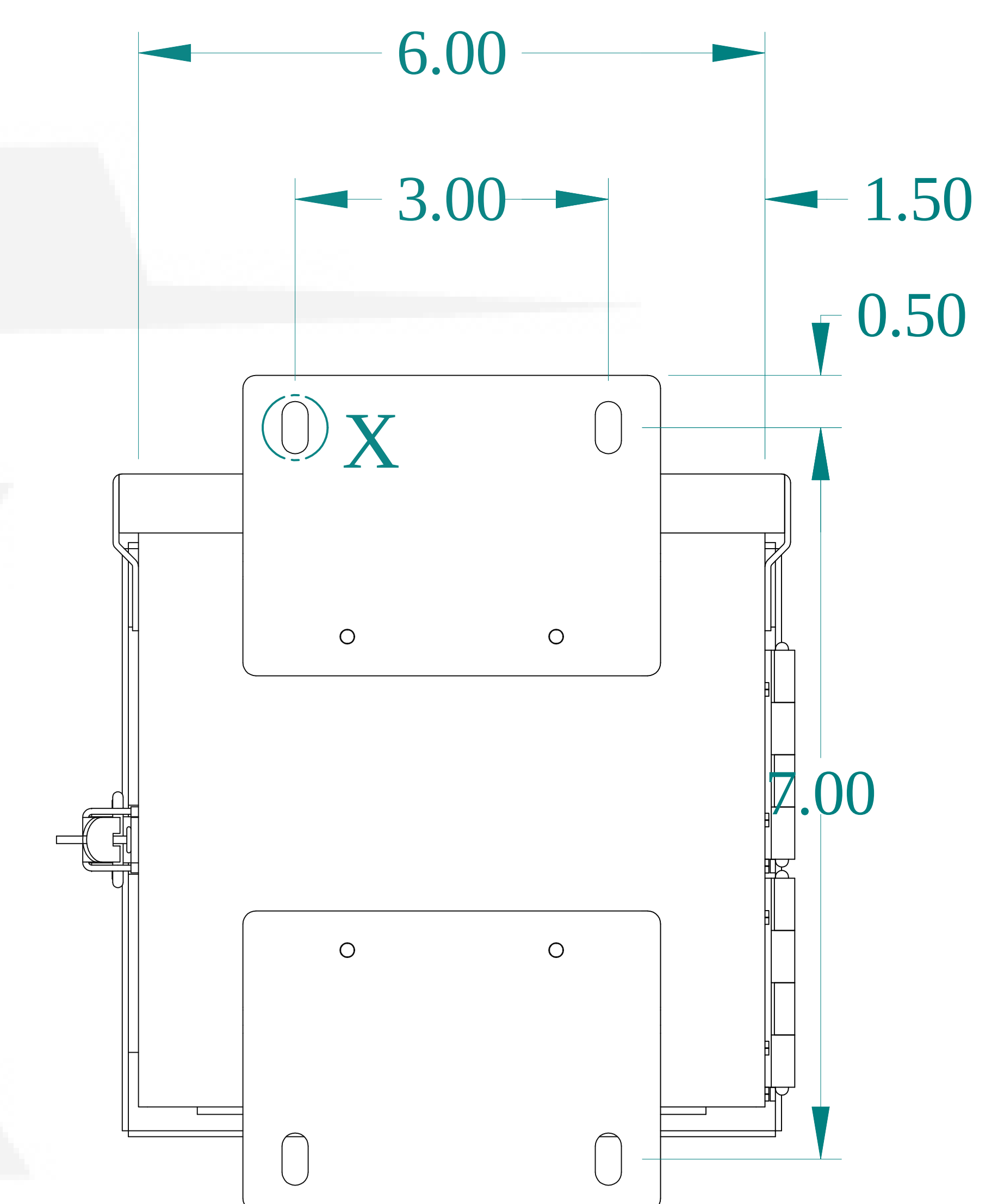
BACK VIEW
