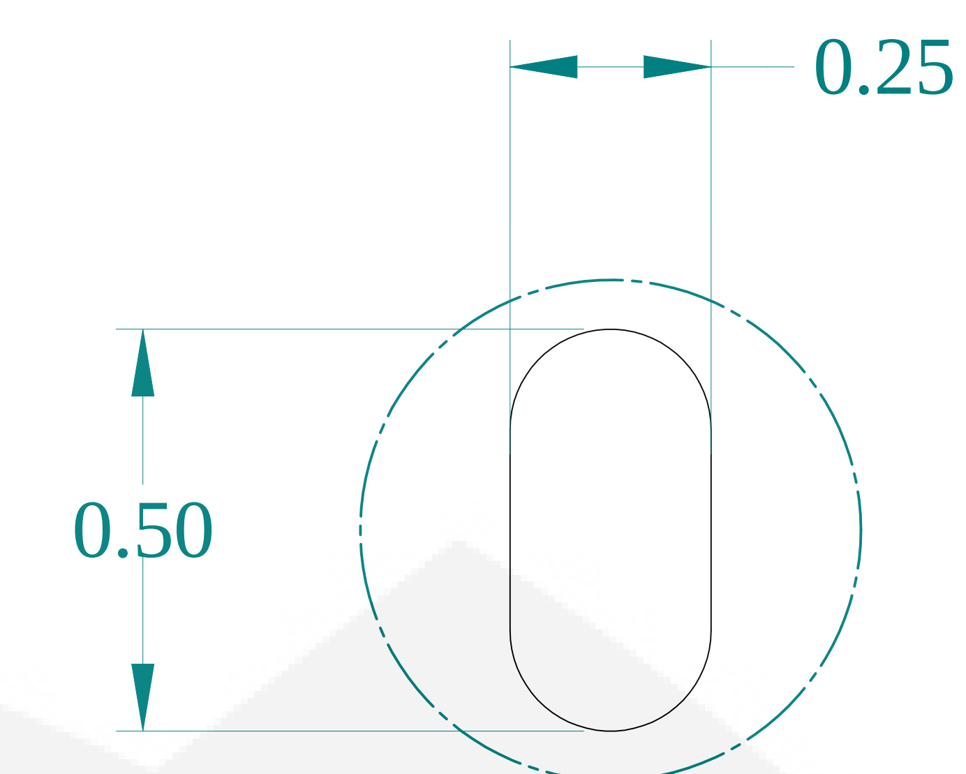
DETAIL X
