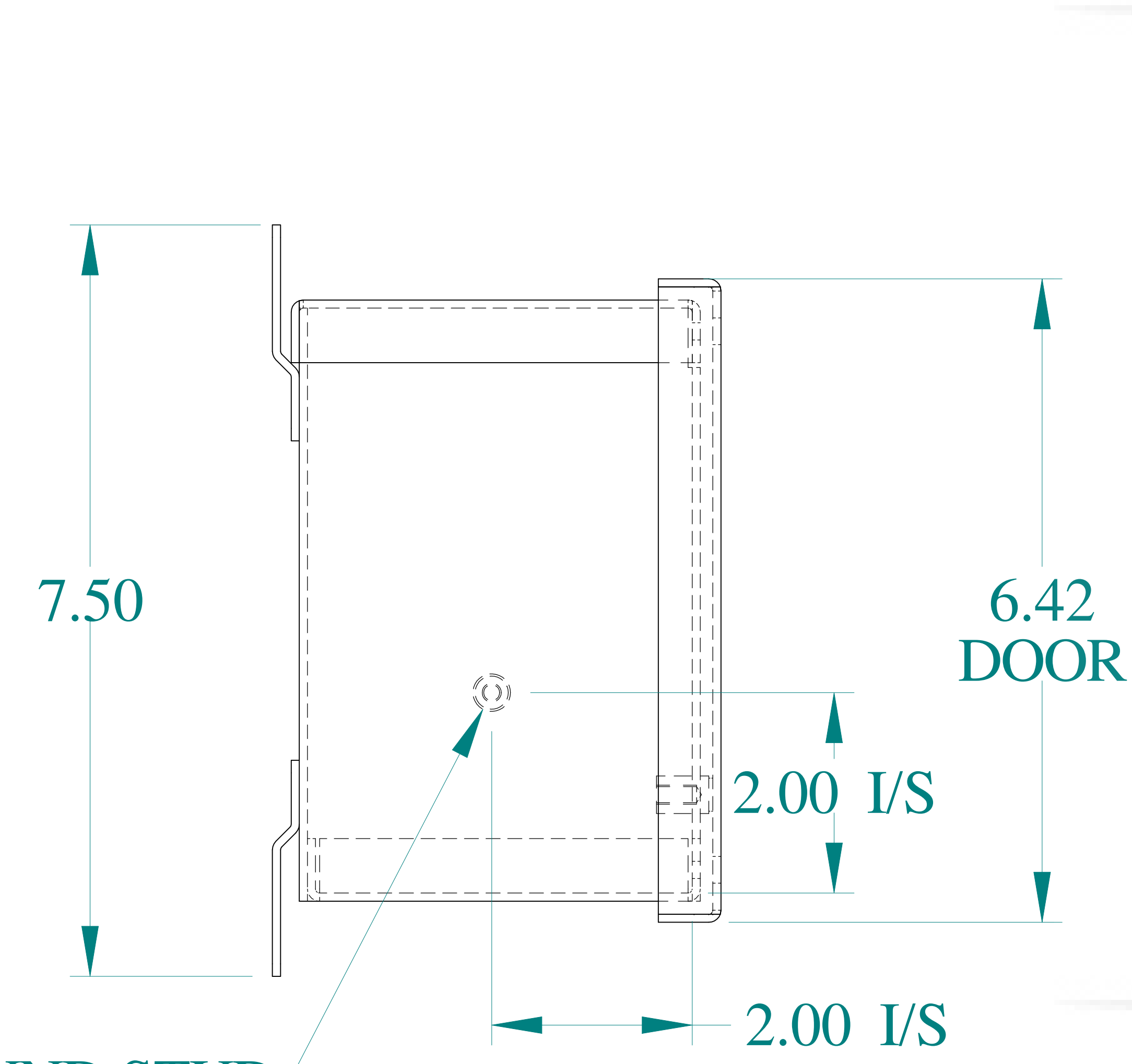
GROUND STUD BODY SIDE VIEW
