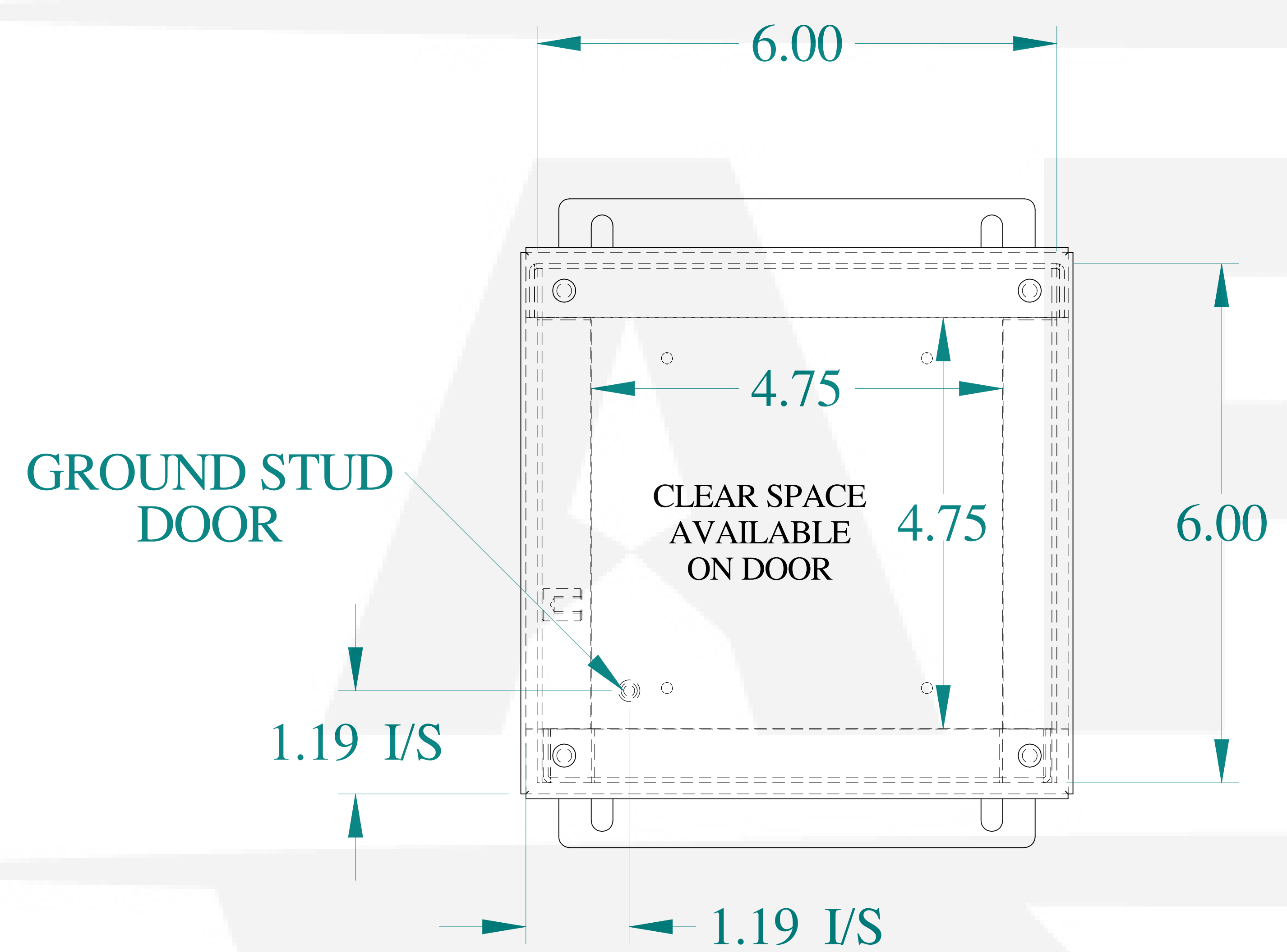
FRONT VIEW
