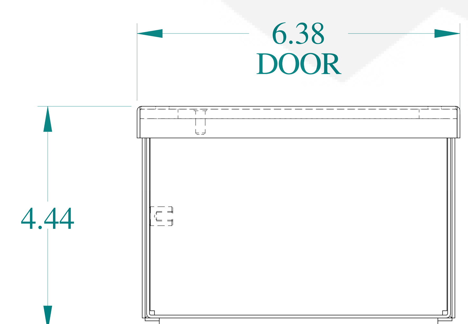
BOTTOM VIEW
