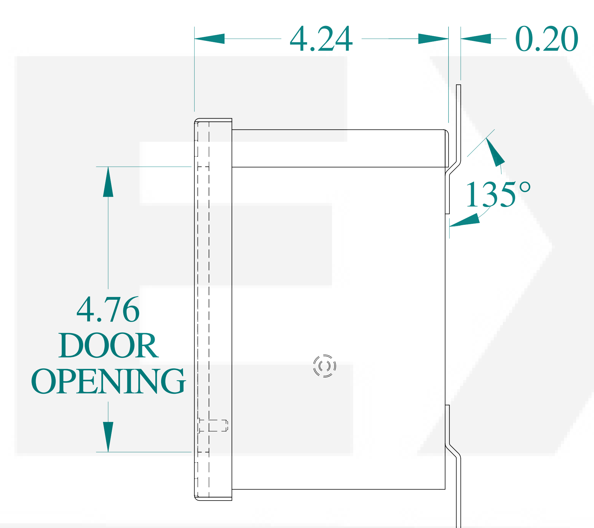
SIDE VIEW
