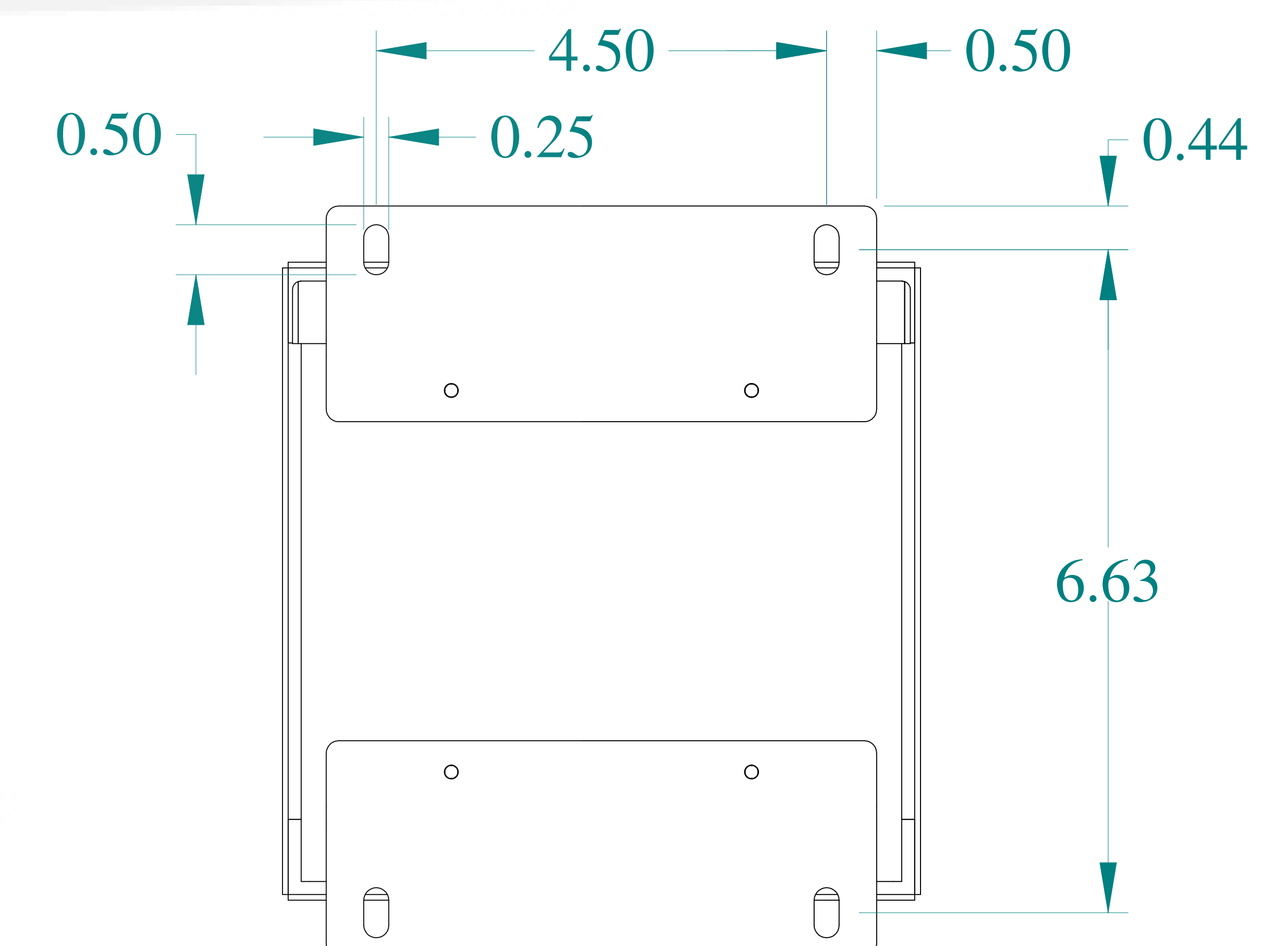
BACK VIEW
