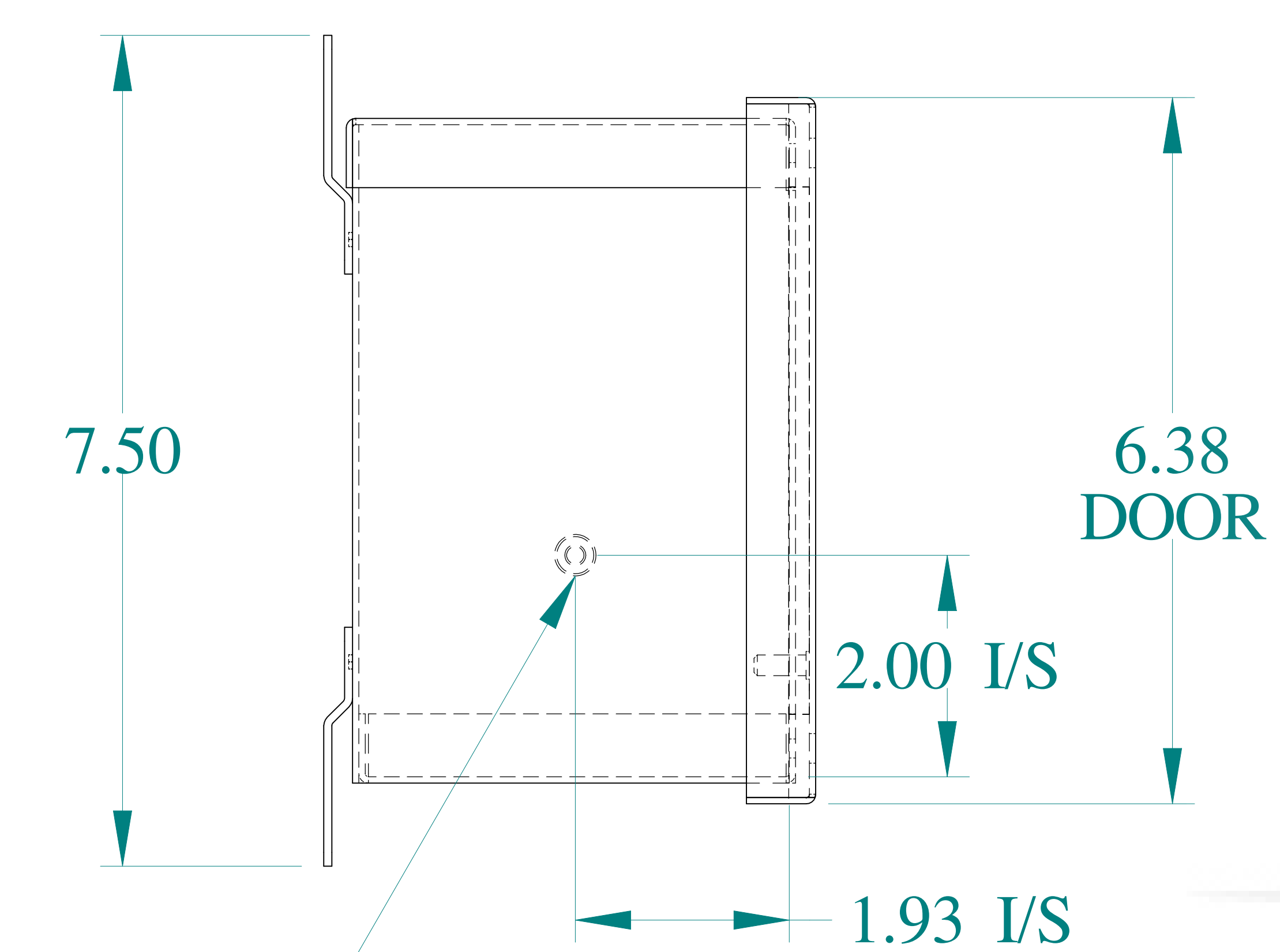
SIDE VIEW
