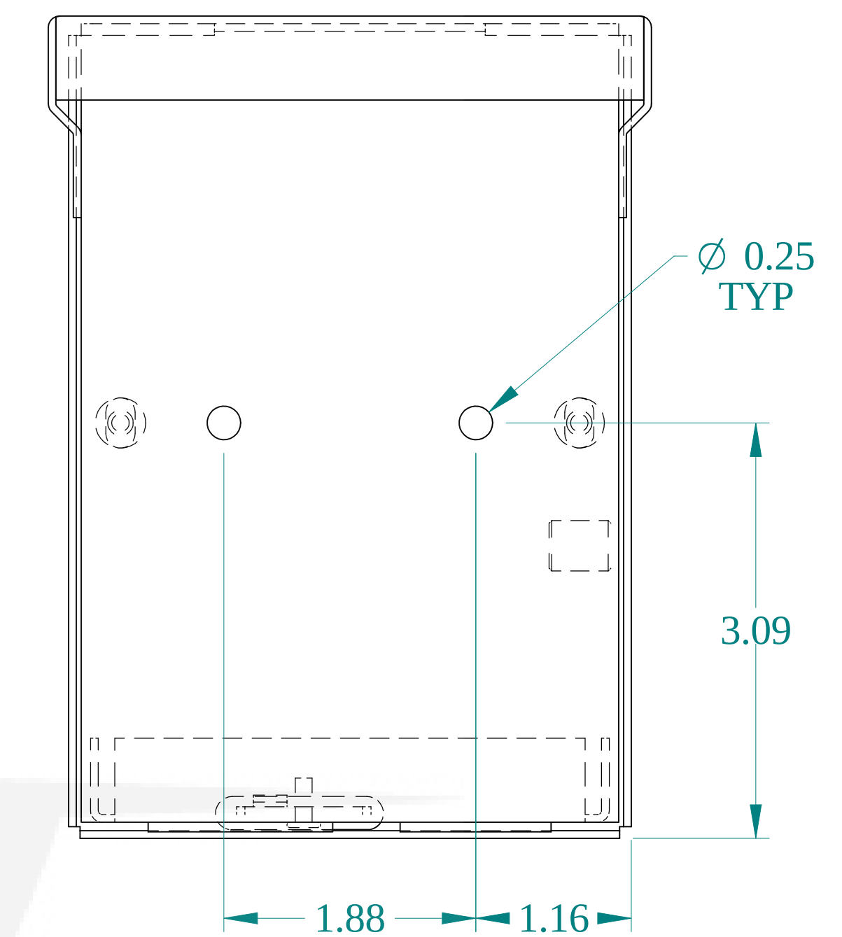
BACK VIEW
