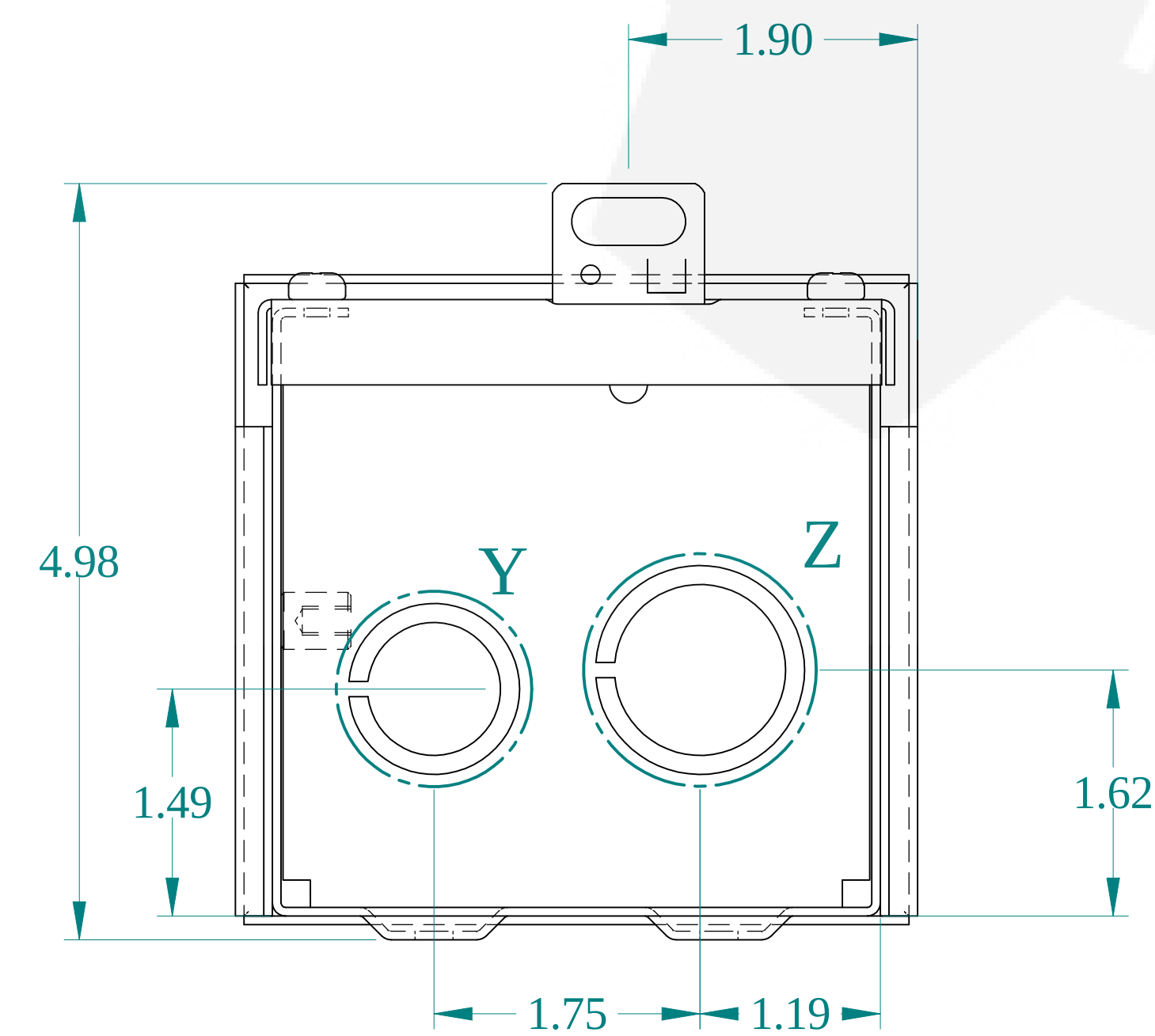
BOTTOM VIEW
