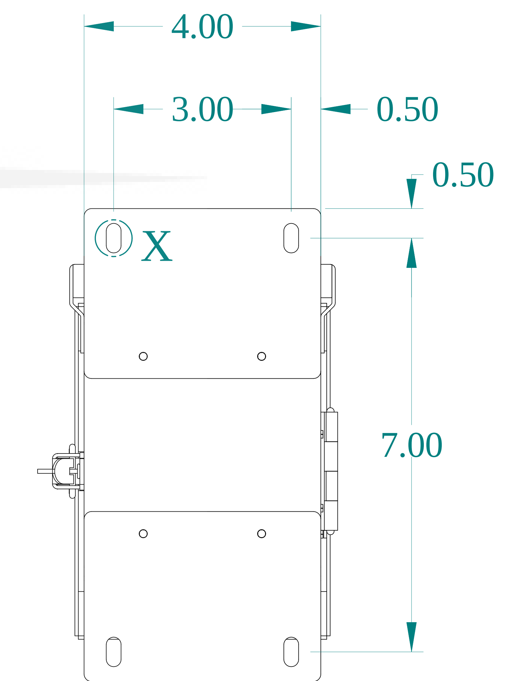
BACK VIEW
