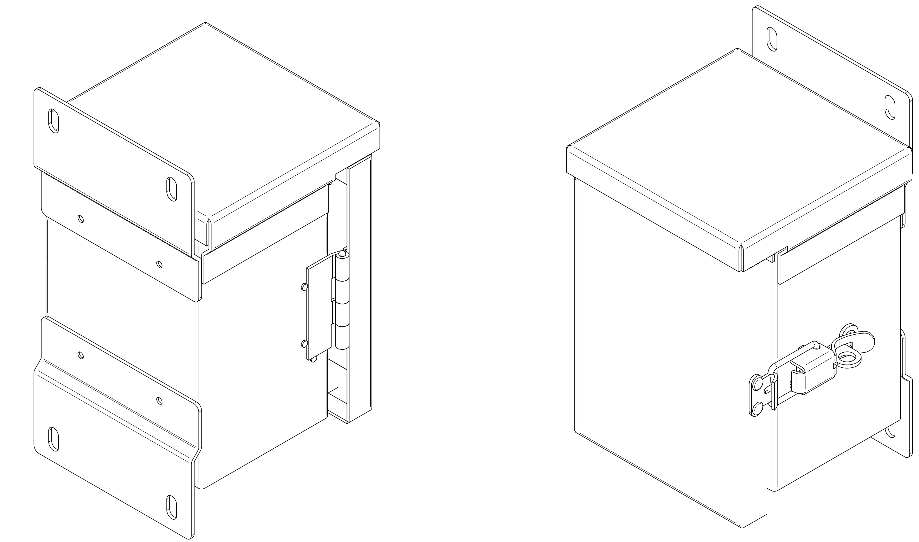
ISOMETRIC VIEWS
