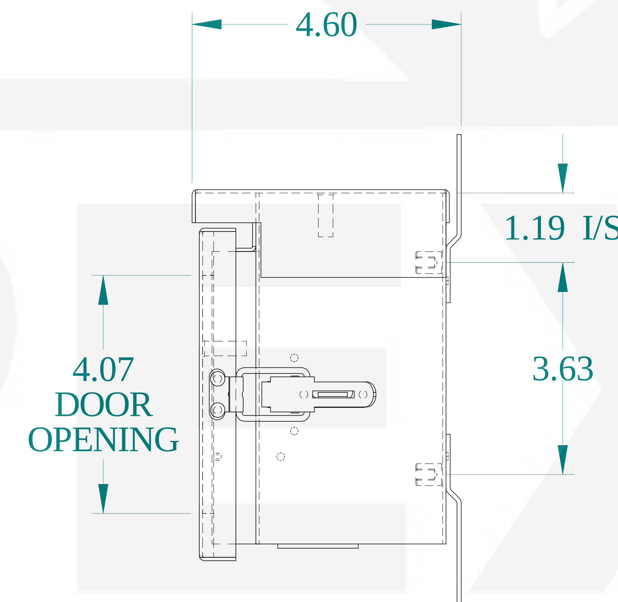
SIDE VIEW
