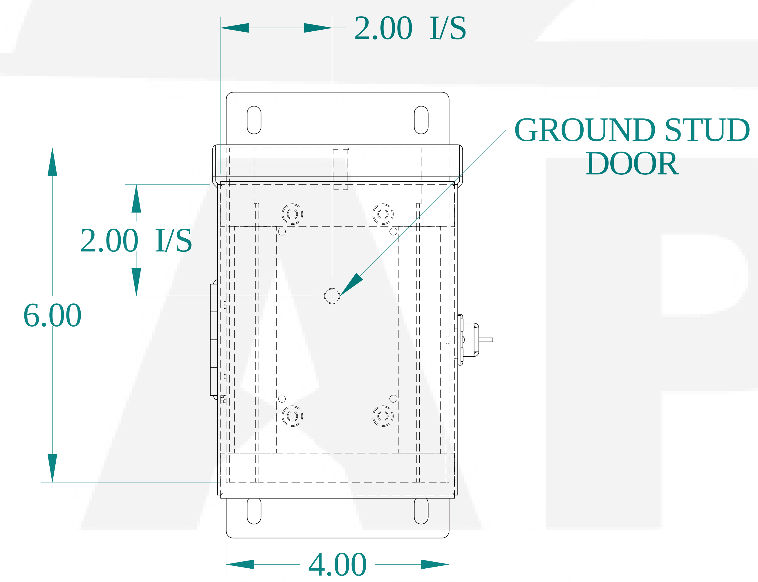
FRONT VIEW
