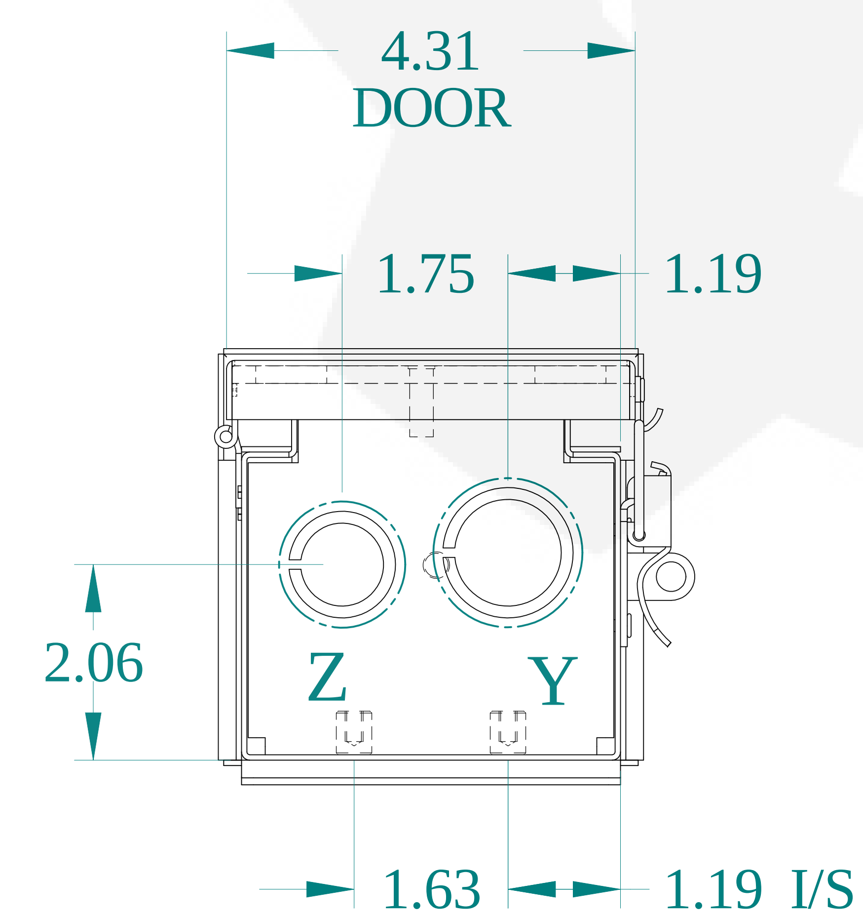
BOTTOM VIEW
