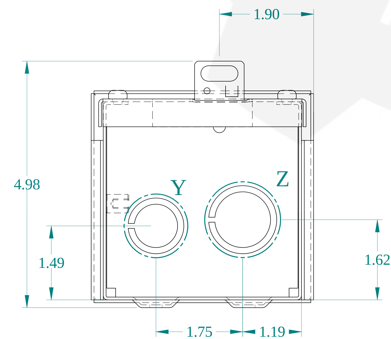
BOTTOM VIEW
