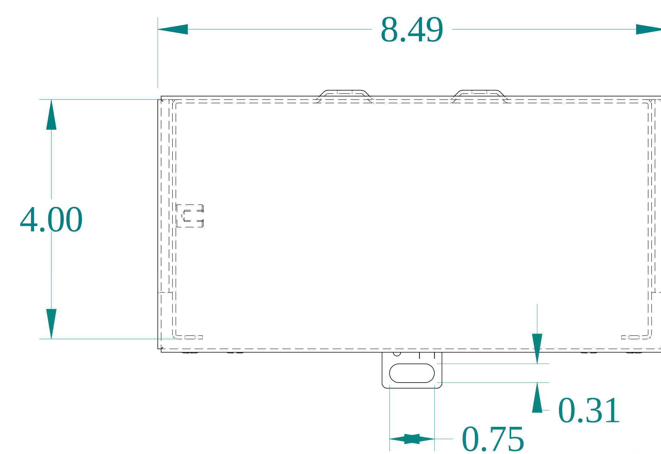
TOP VIEW
