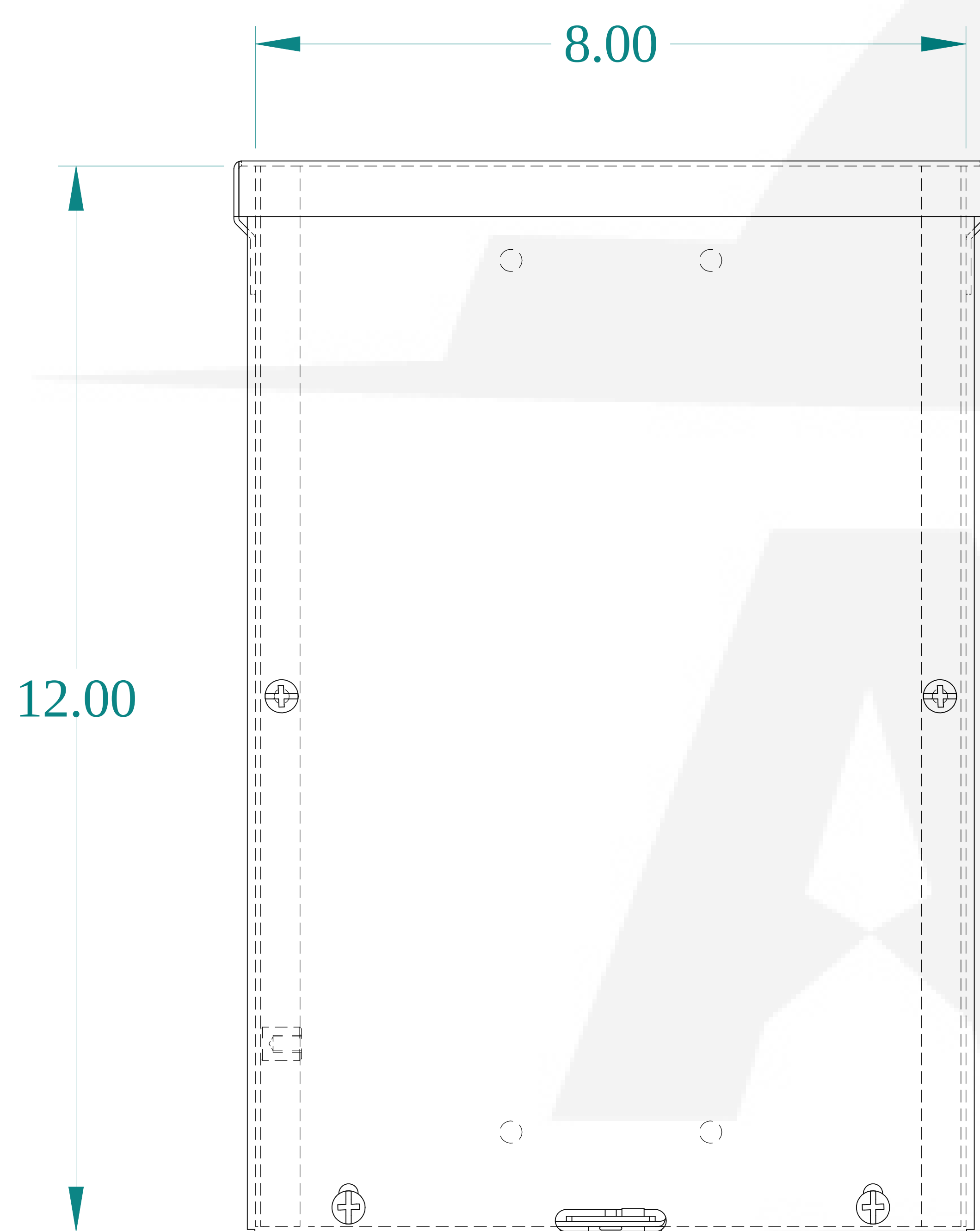
FRONT VIEW
