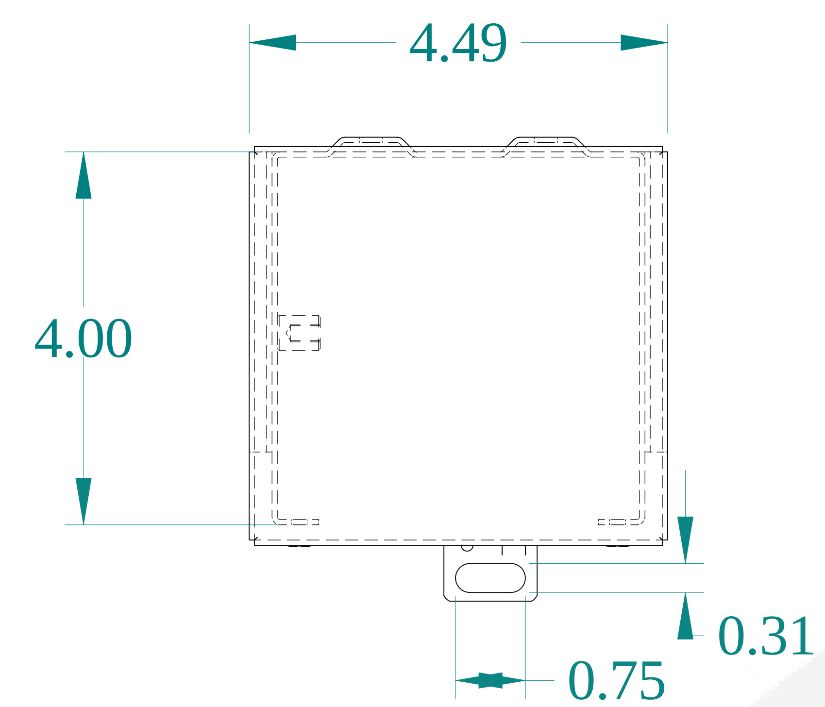
TOP VIEW
