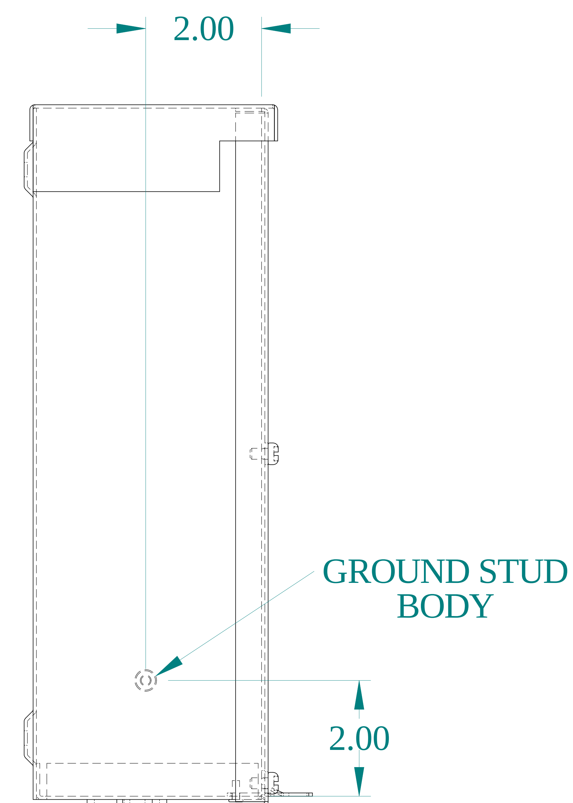
SIDE VIEW
