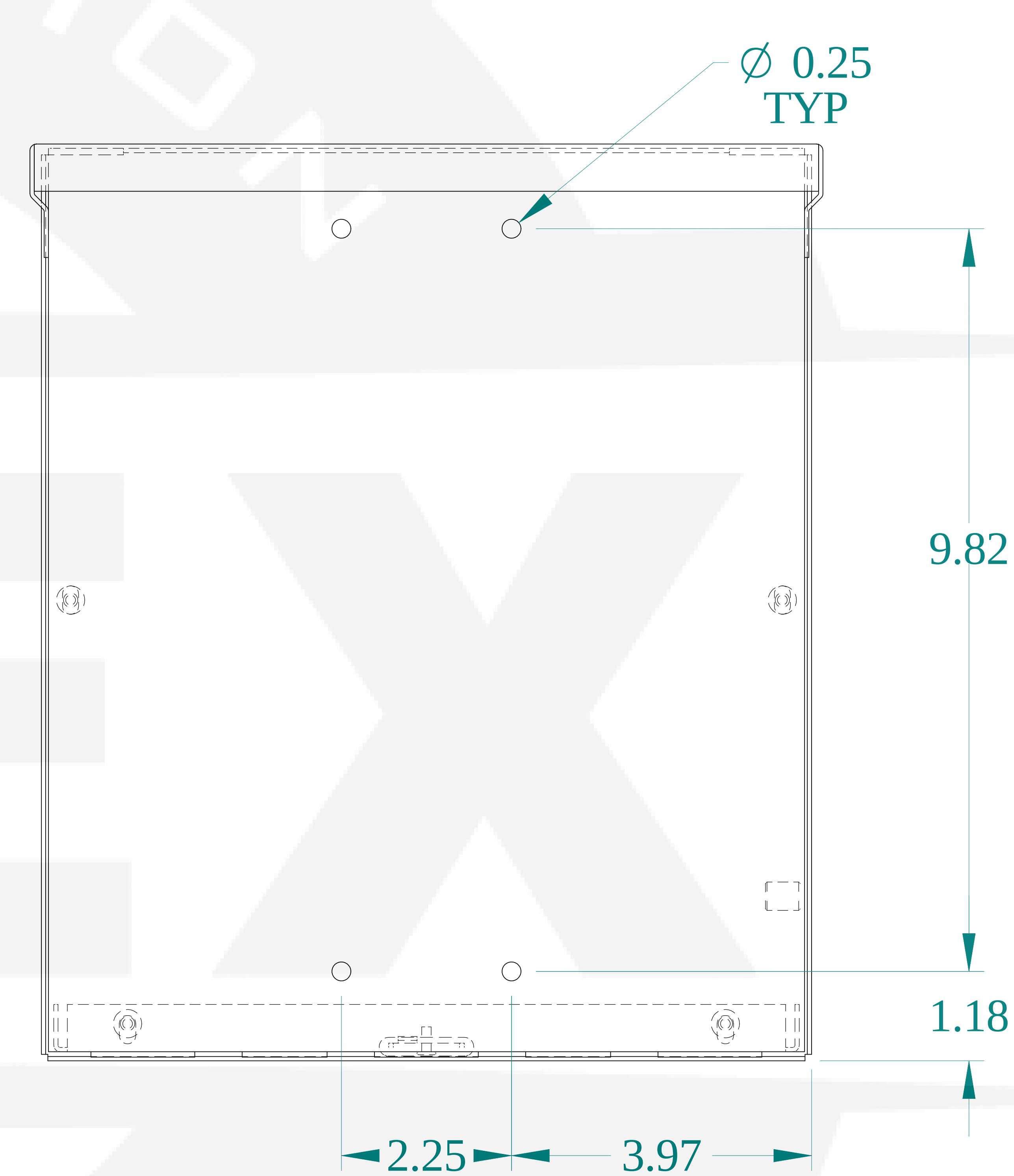
BACK VIEW
