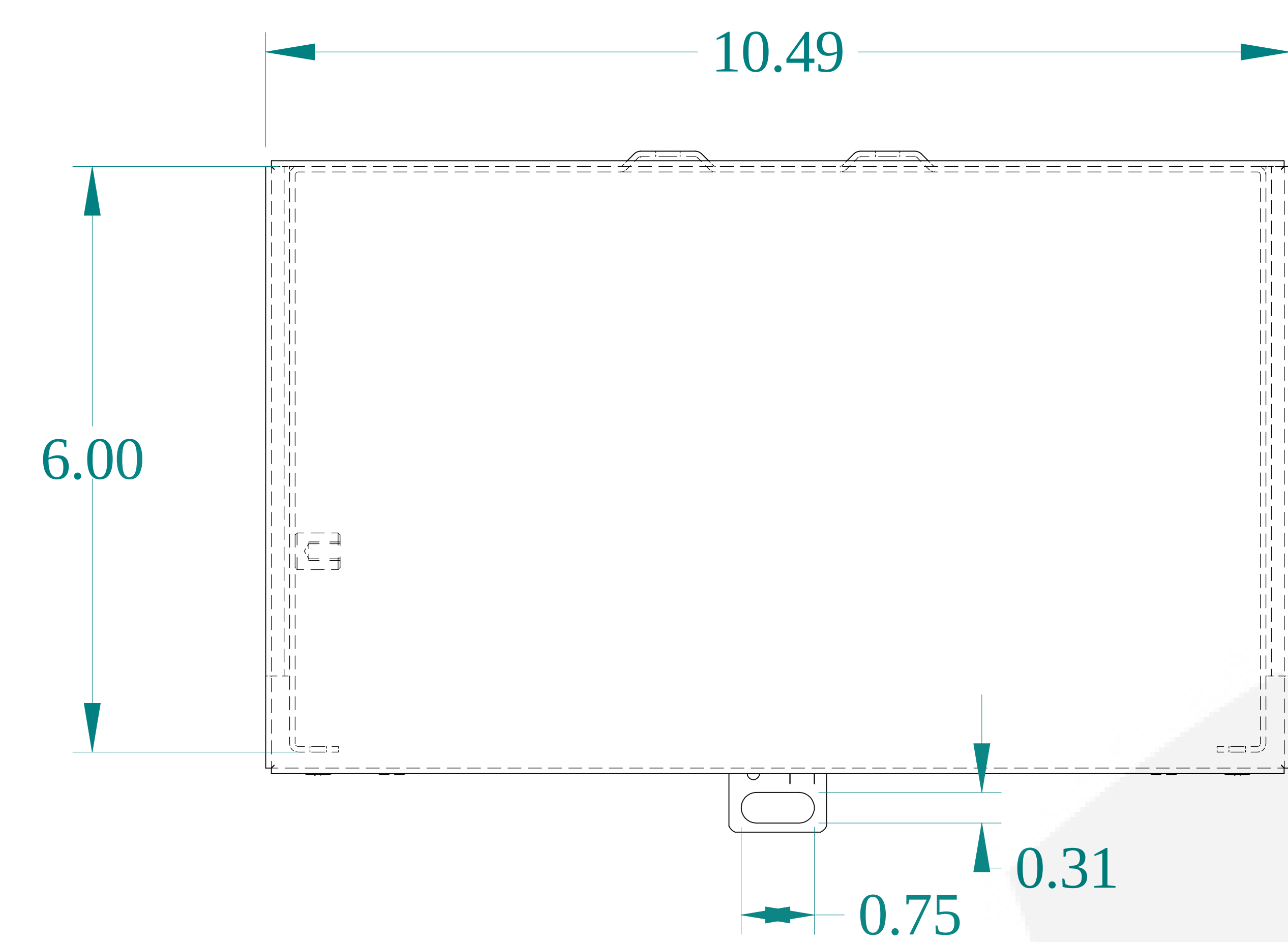
TOP VIEW
