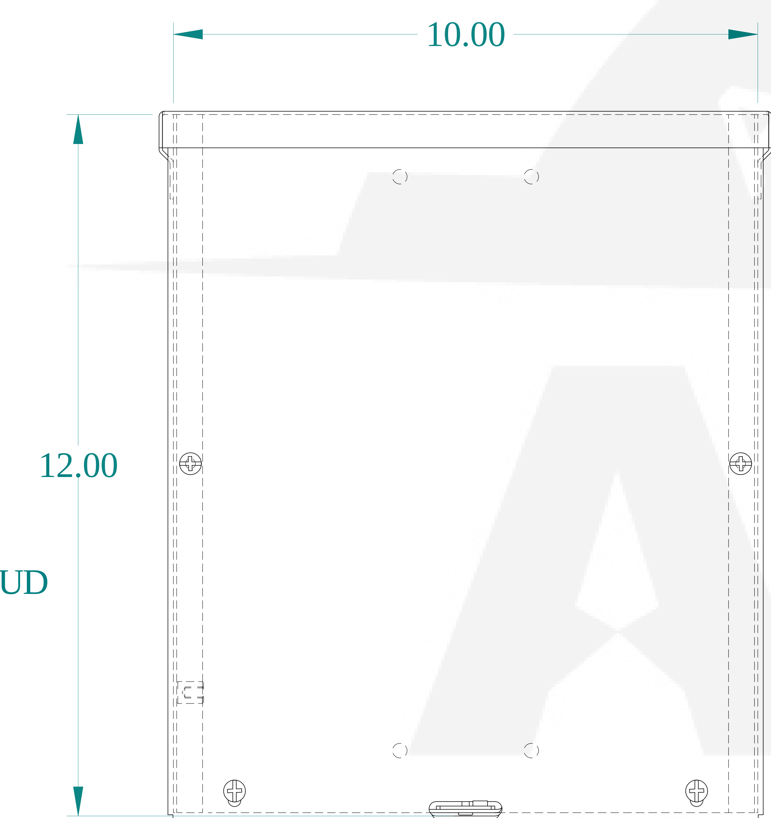
TOP VIEW
