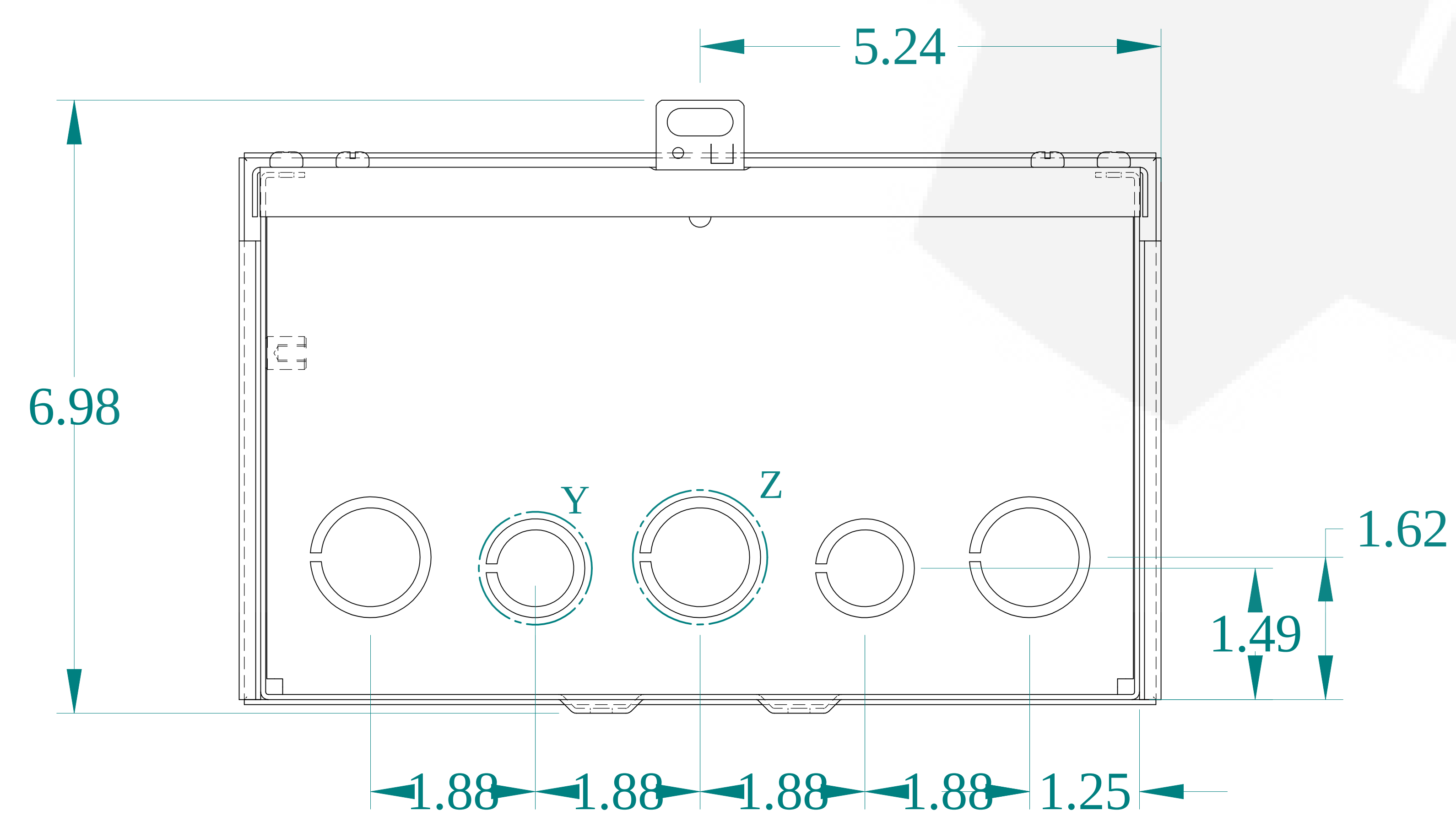
BOTTOM VIEW
