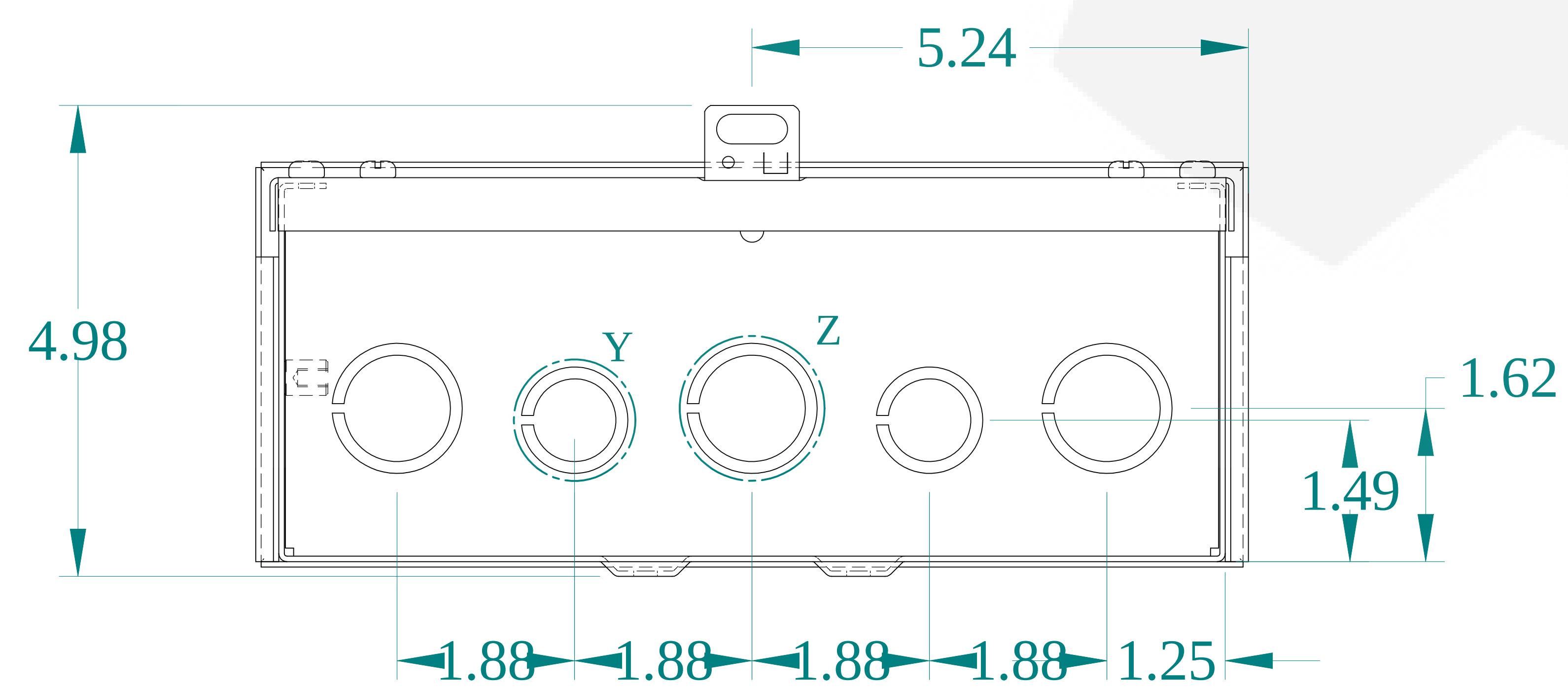
BOTTOM VIEW
