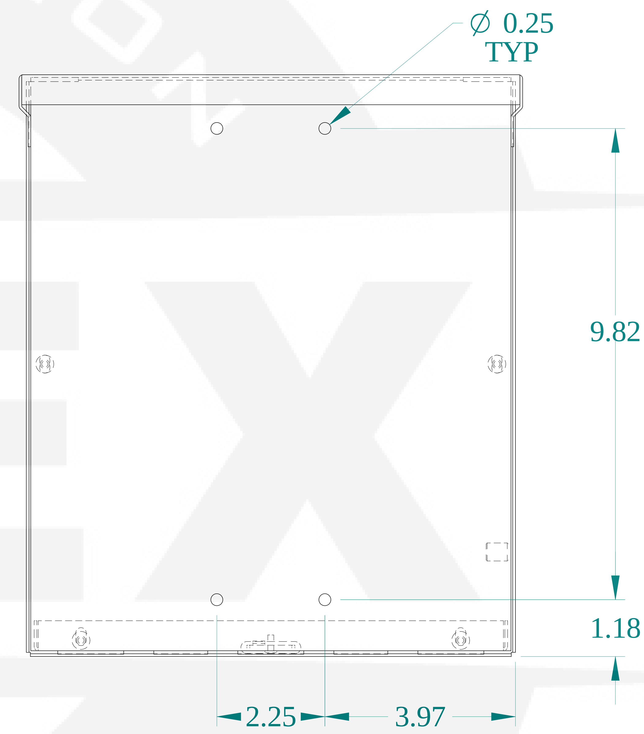
BACK VIEW
