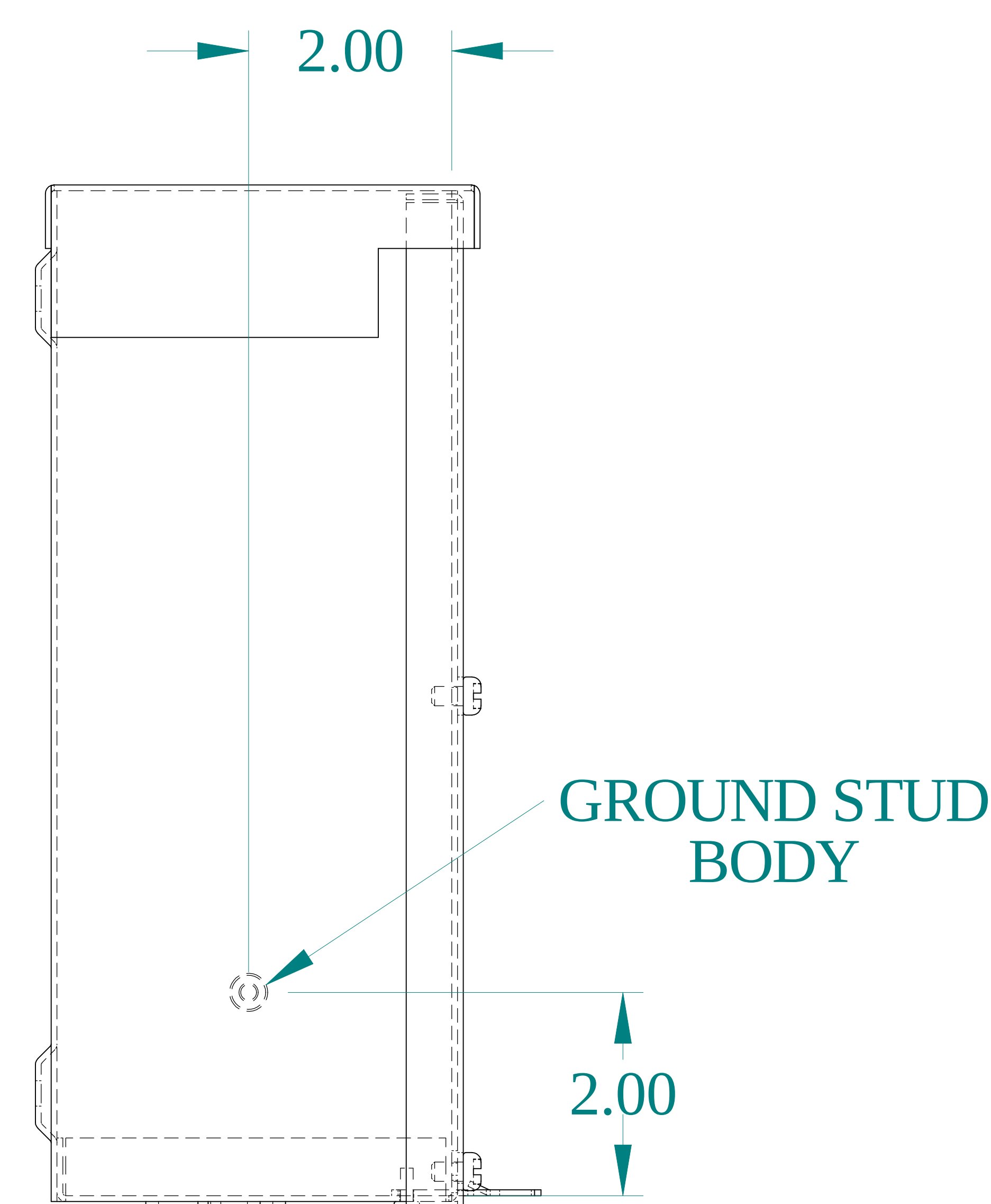
SIDE VIEW
