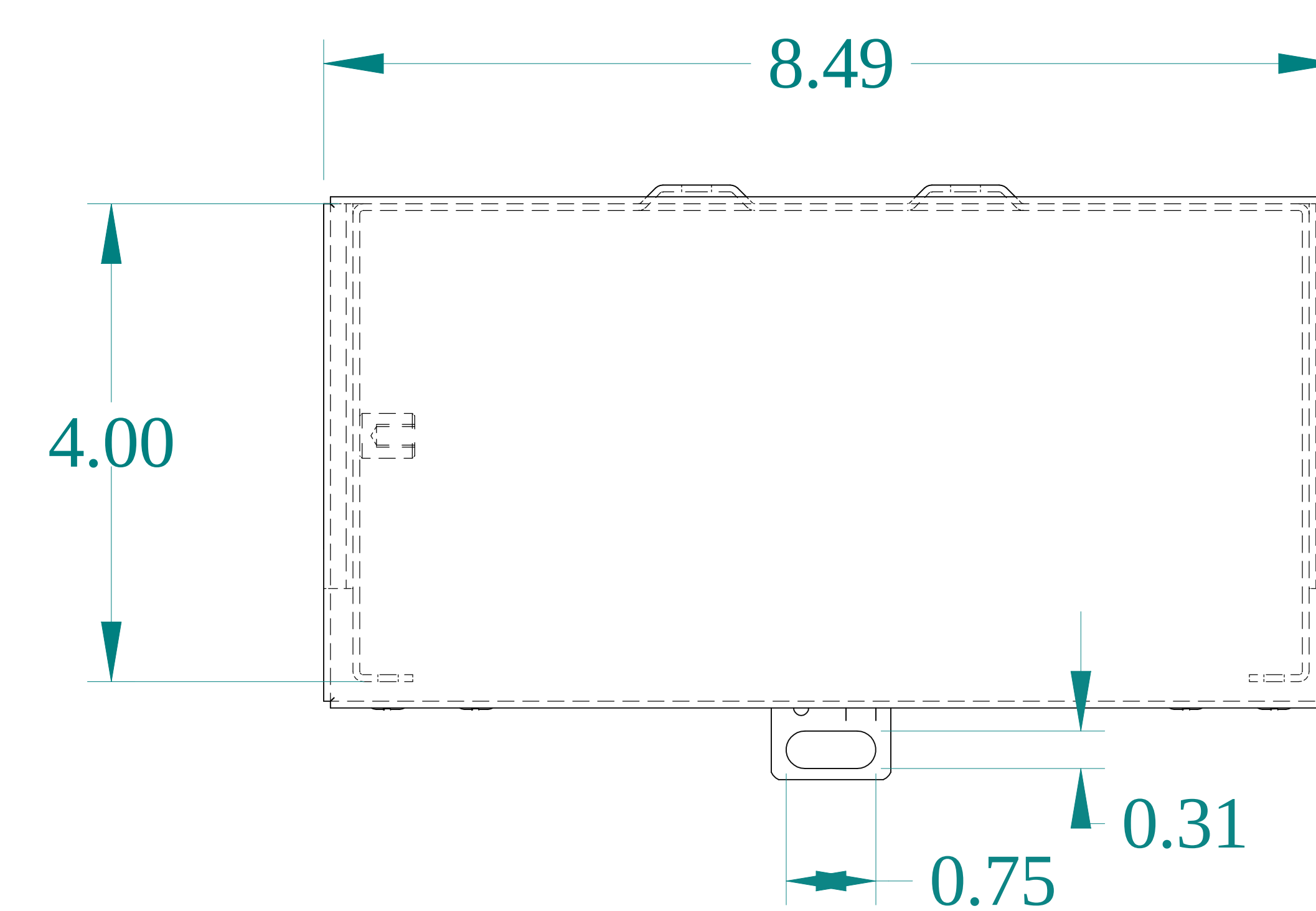
TOP VIEW
