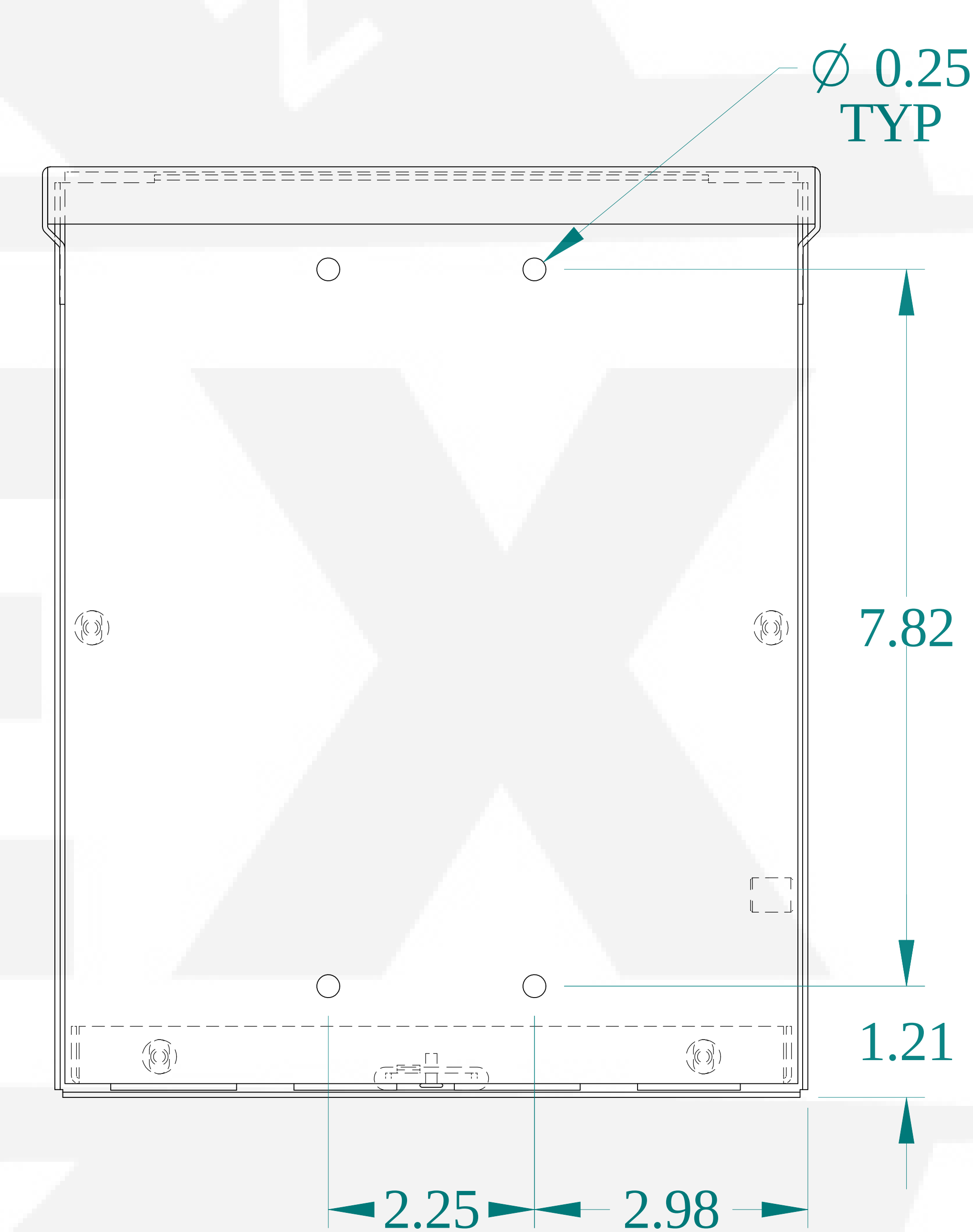
BACK VIEW
