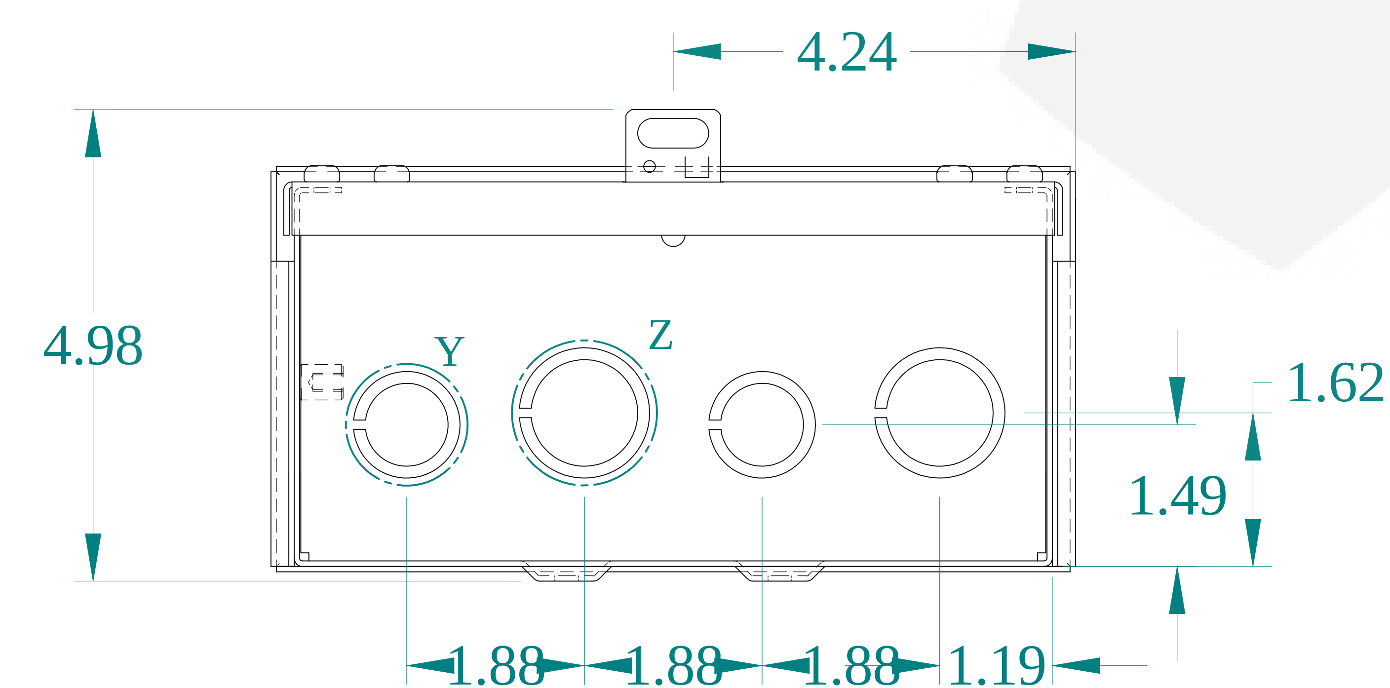
BOTTOM VIEW
