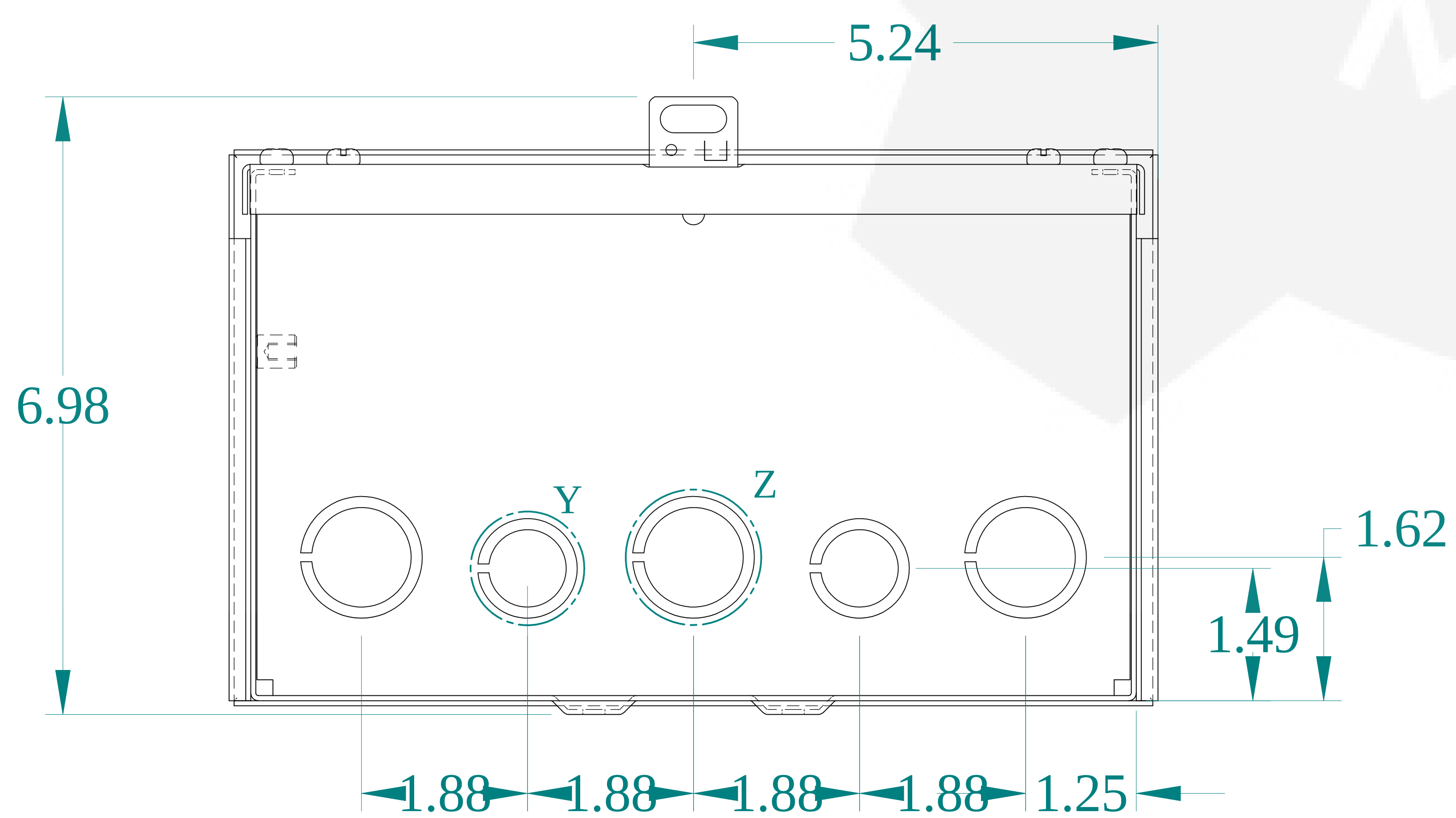
BOTTOM VIEW
