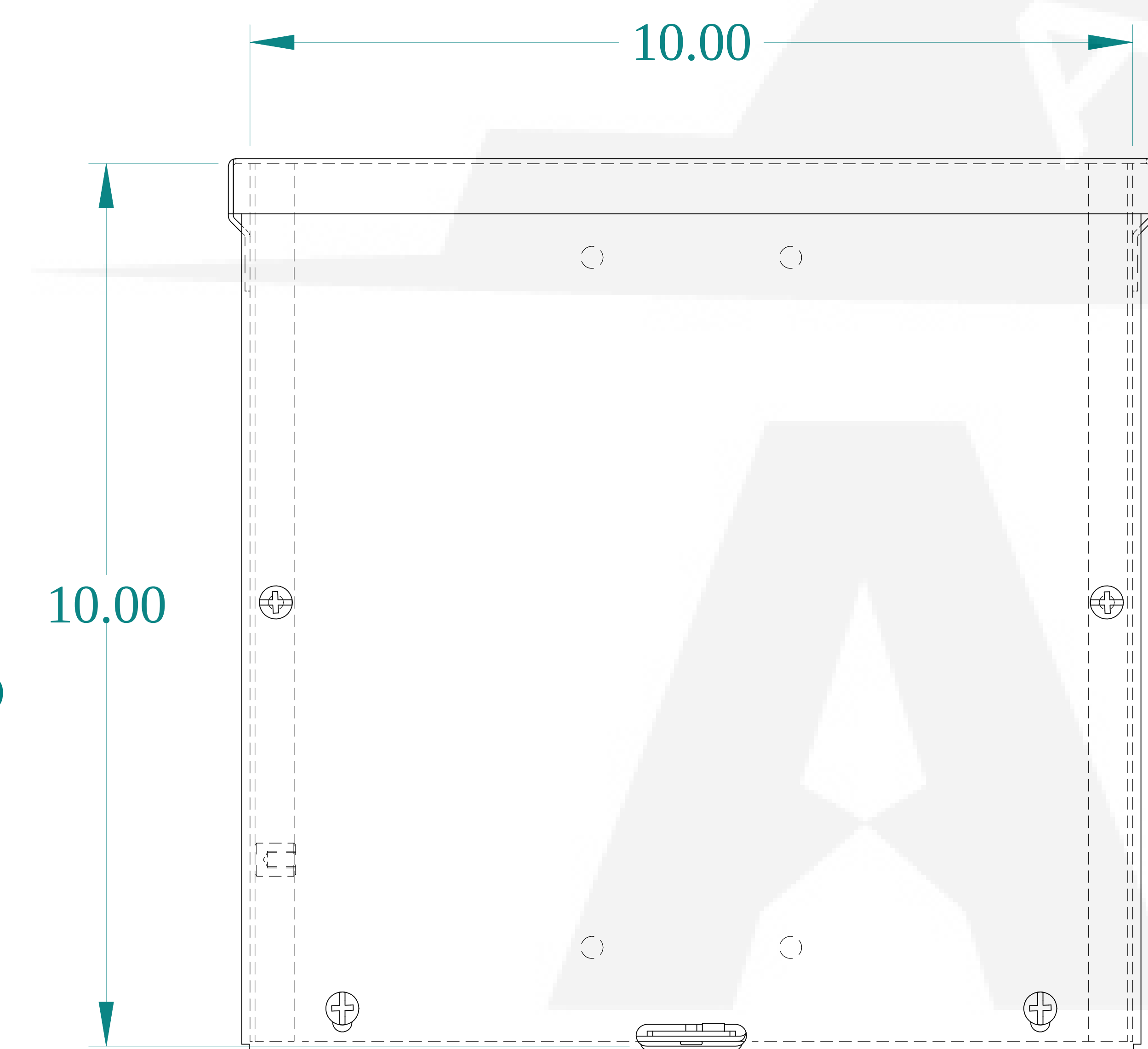
TOP VIEW
