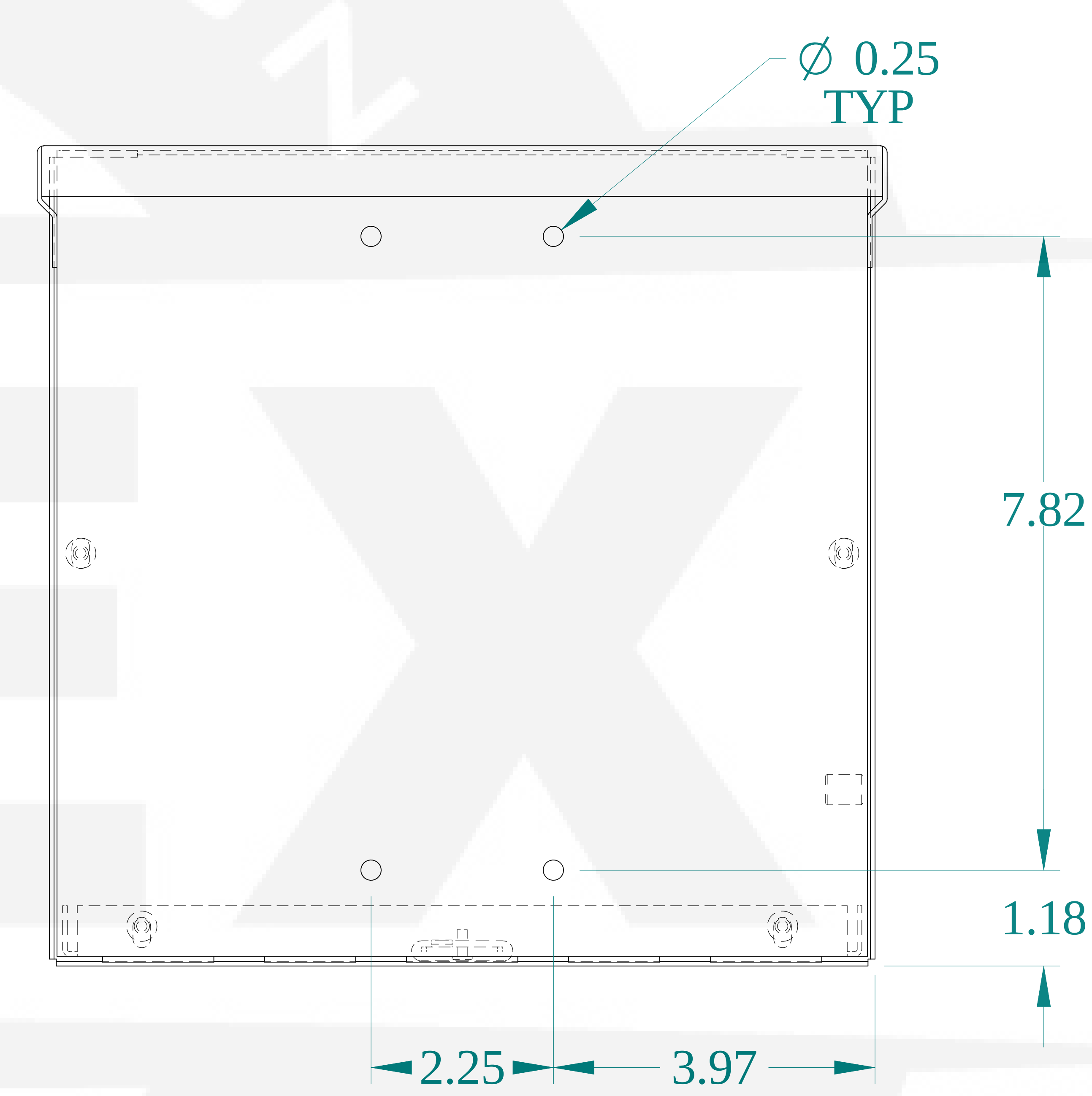
BACK VIEW
