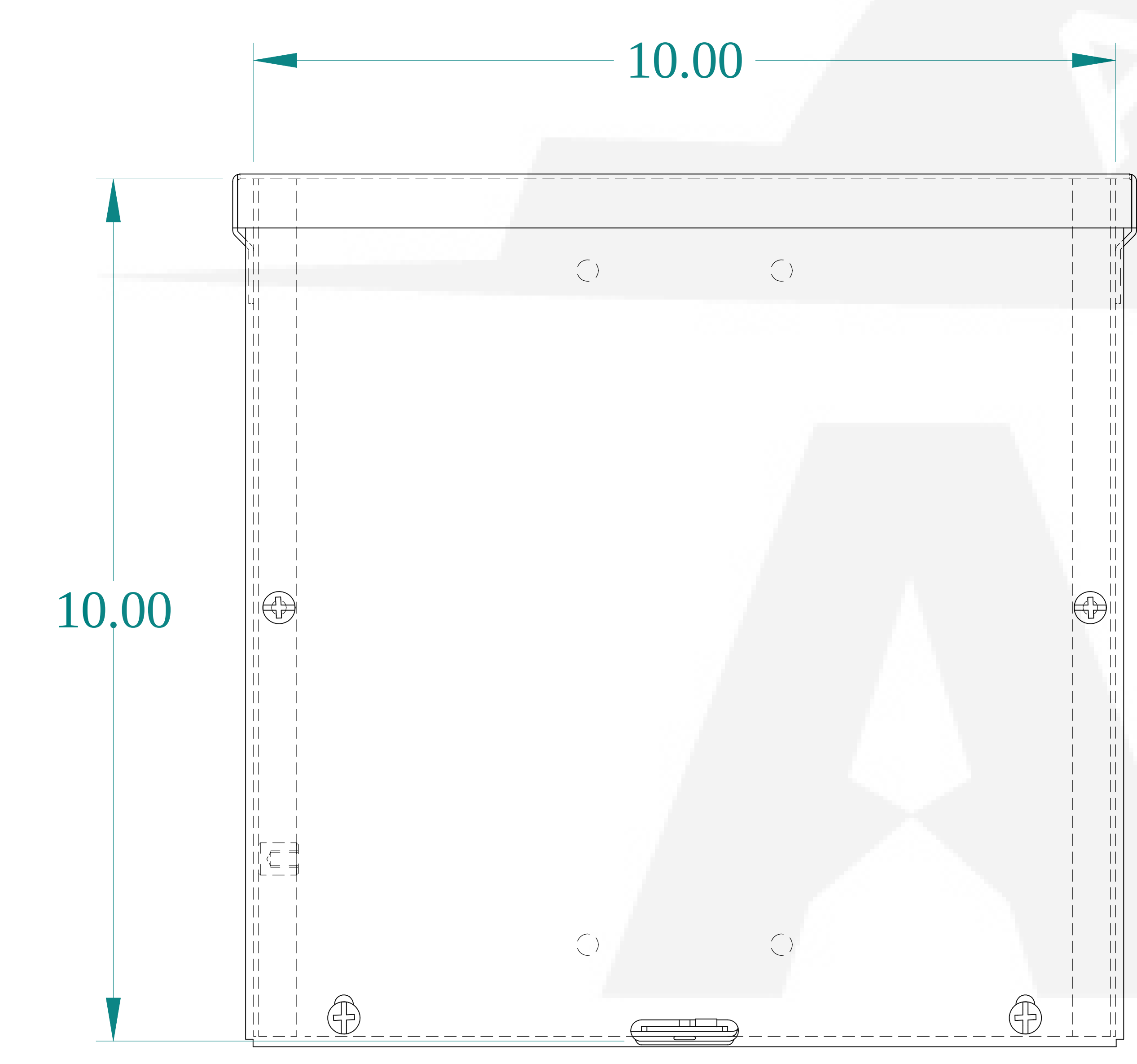
FRONT VIEW
