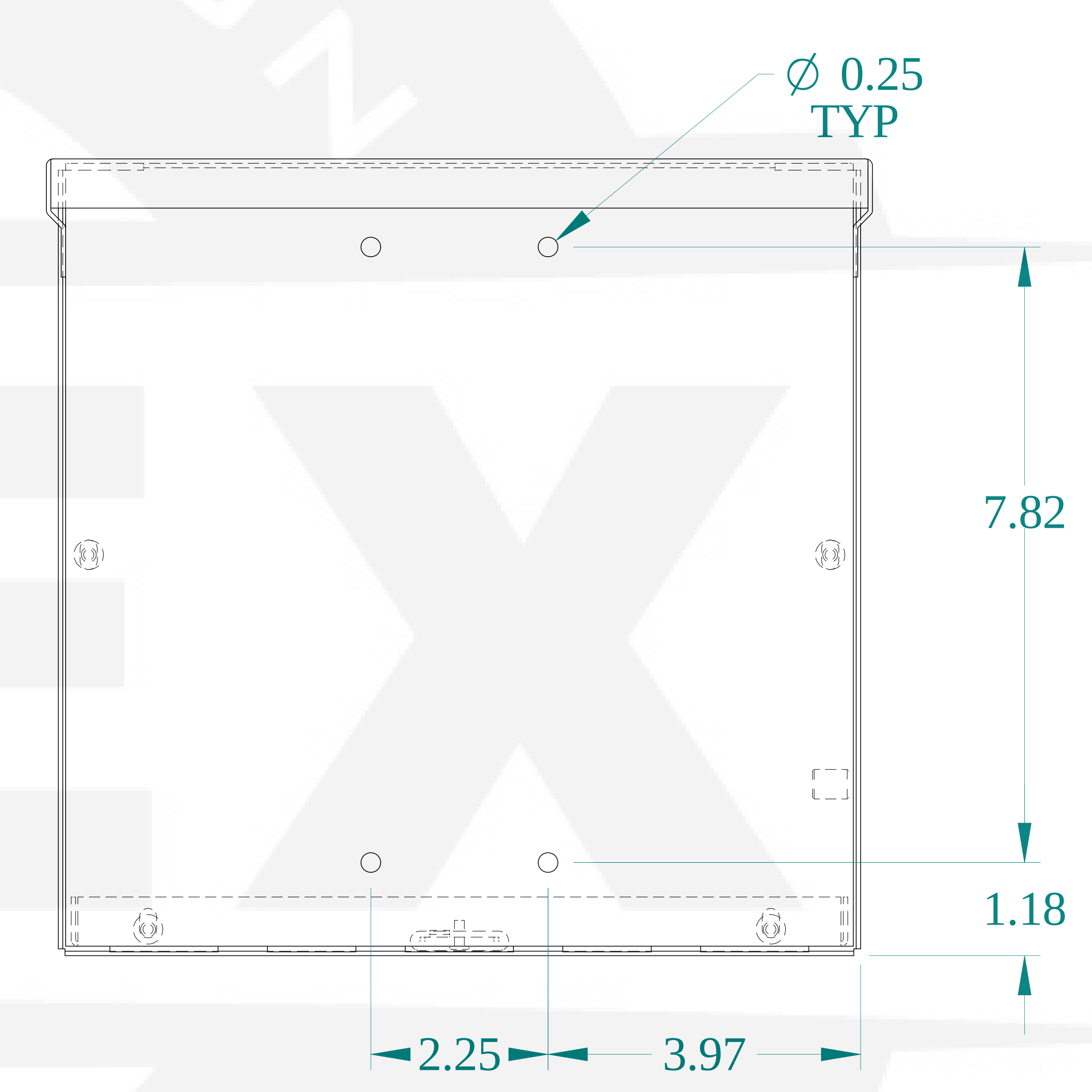
BACK VIEW
