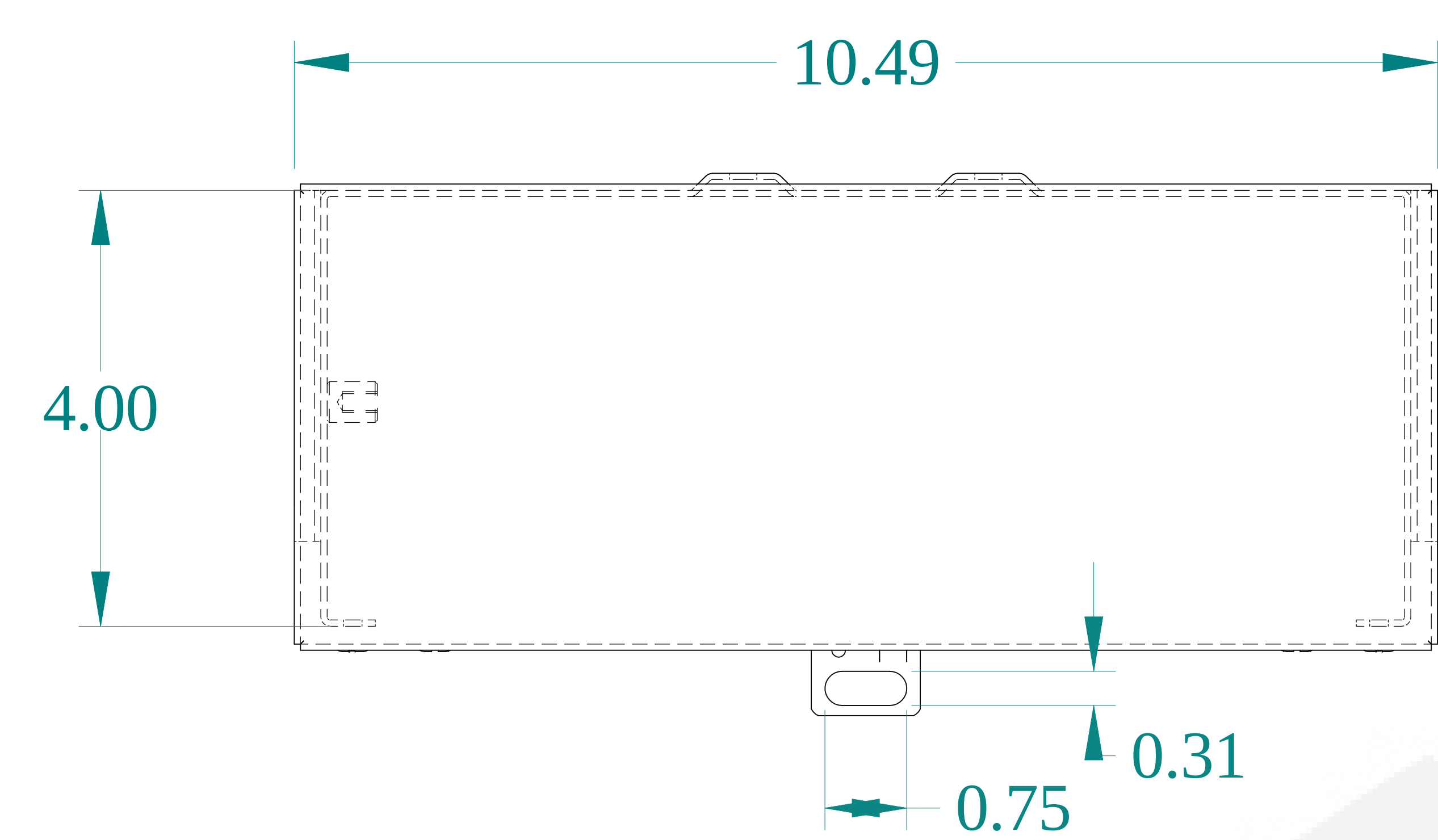
TOP VIEW
