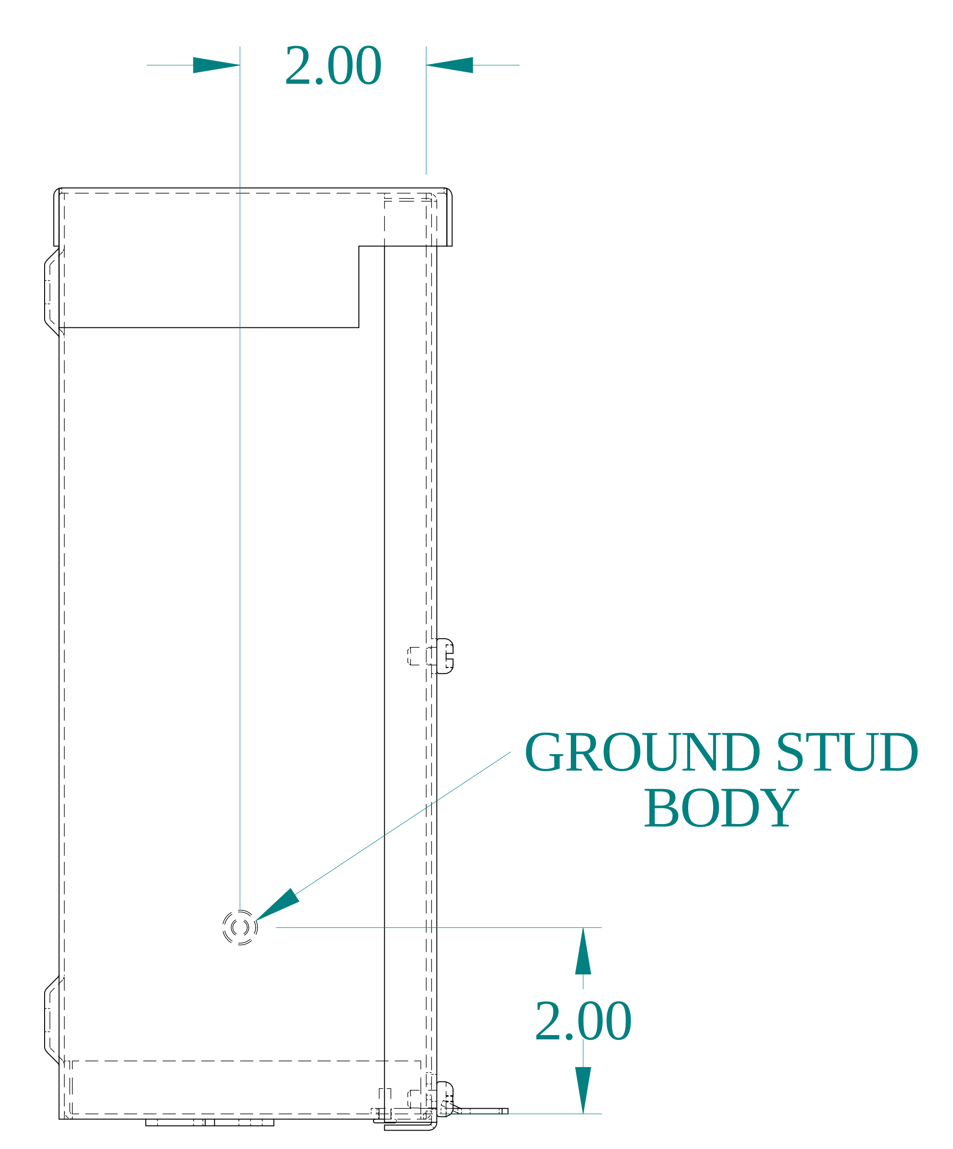
SIDE VIEW
