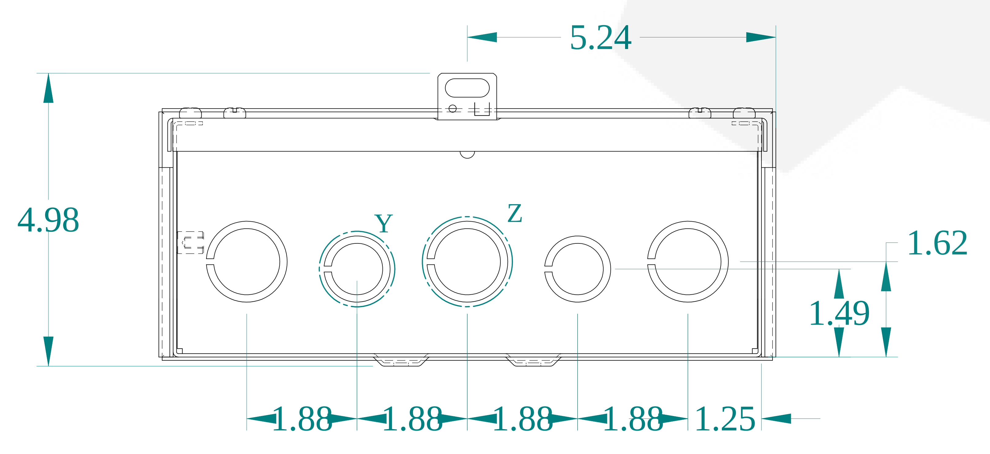
BOTTOM VIEW
