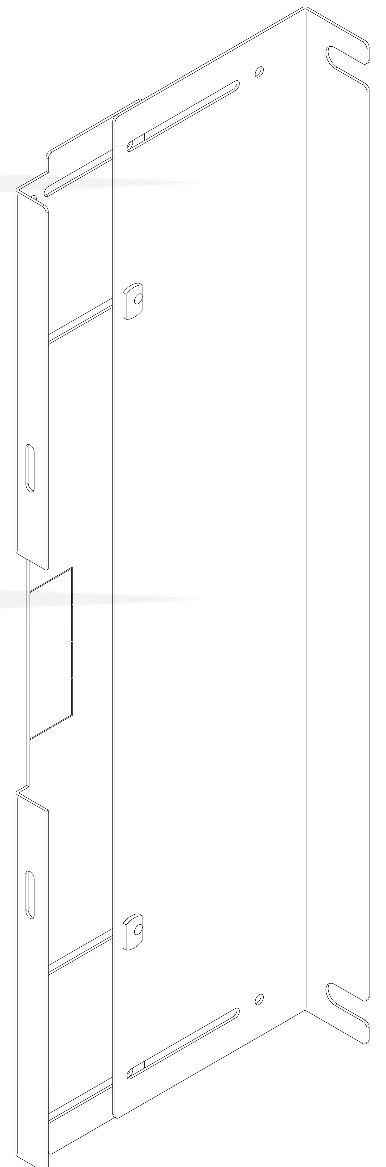
ISOMETRIC VIEW
