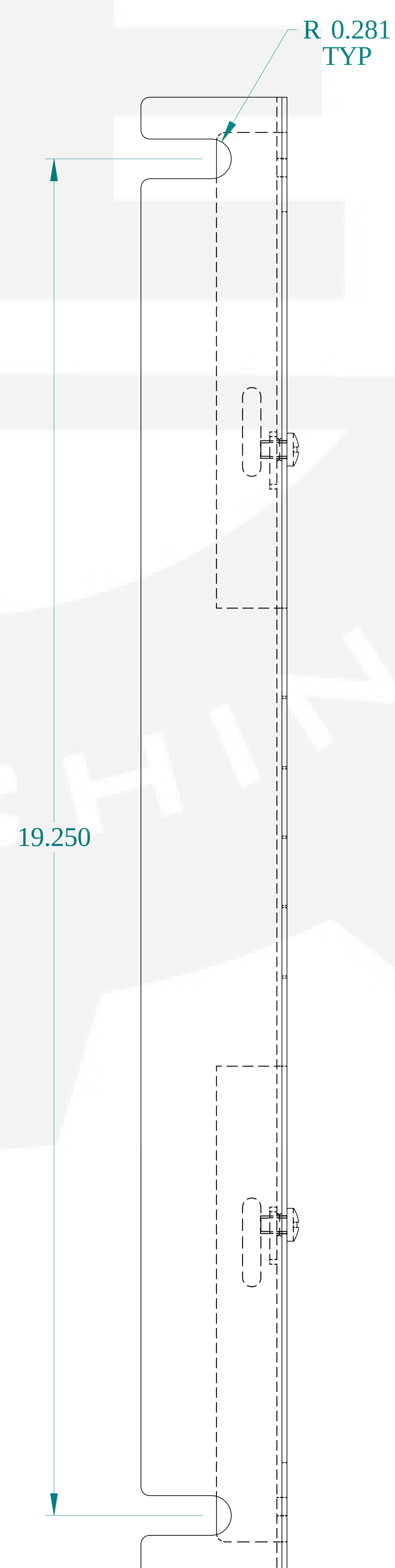
SIDE VIEW
