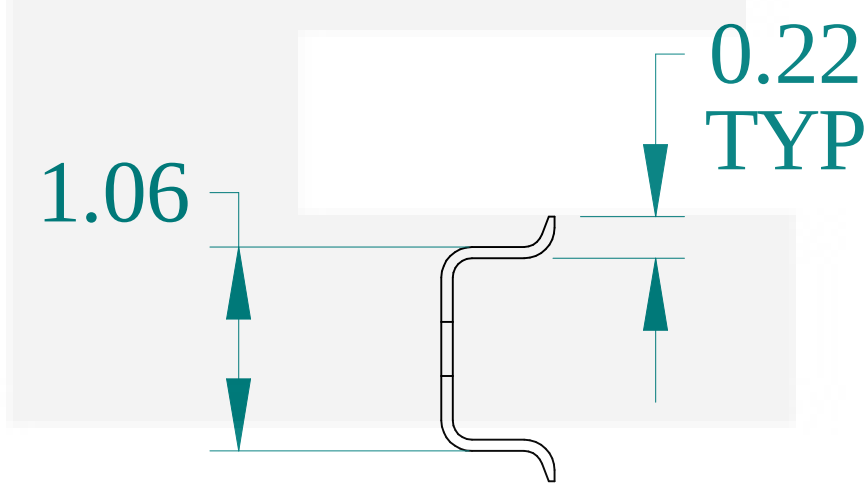
SIDE VIEW
