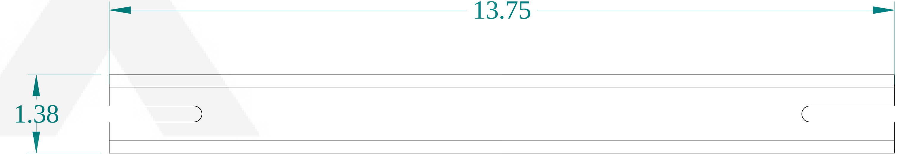
BACK VIEW
