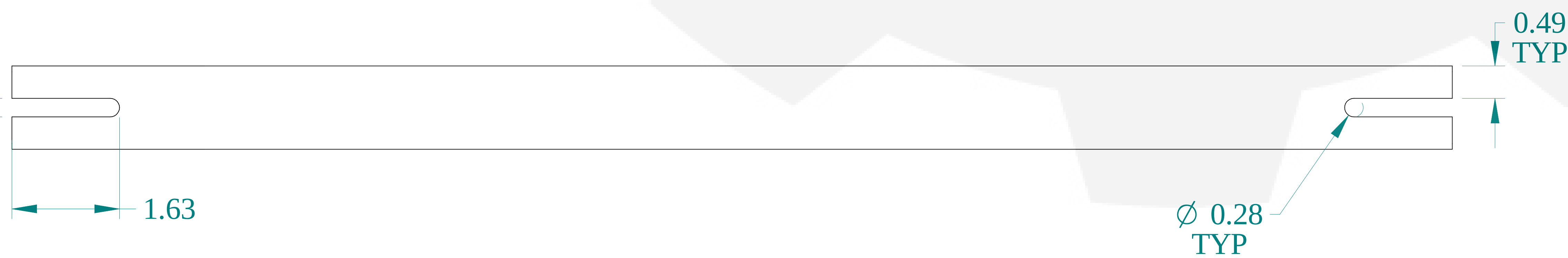
BOTTOM VIEW
