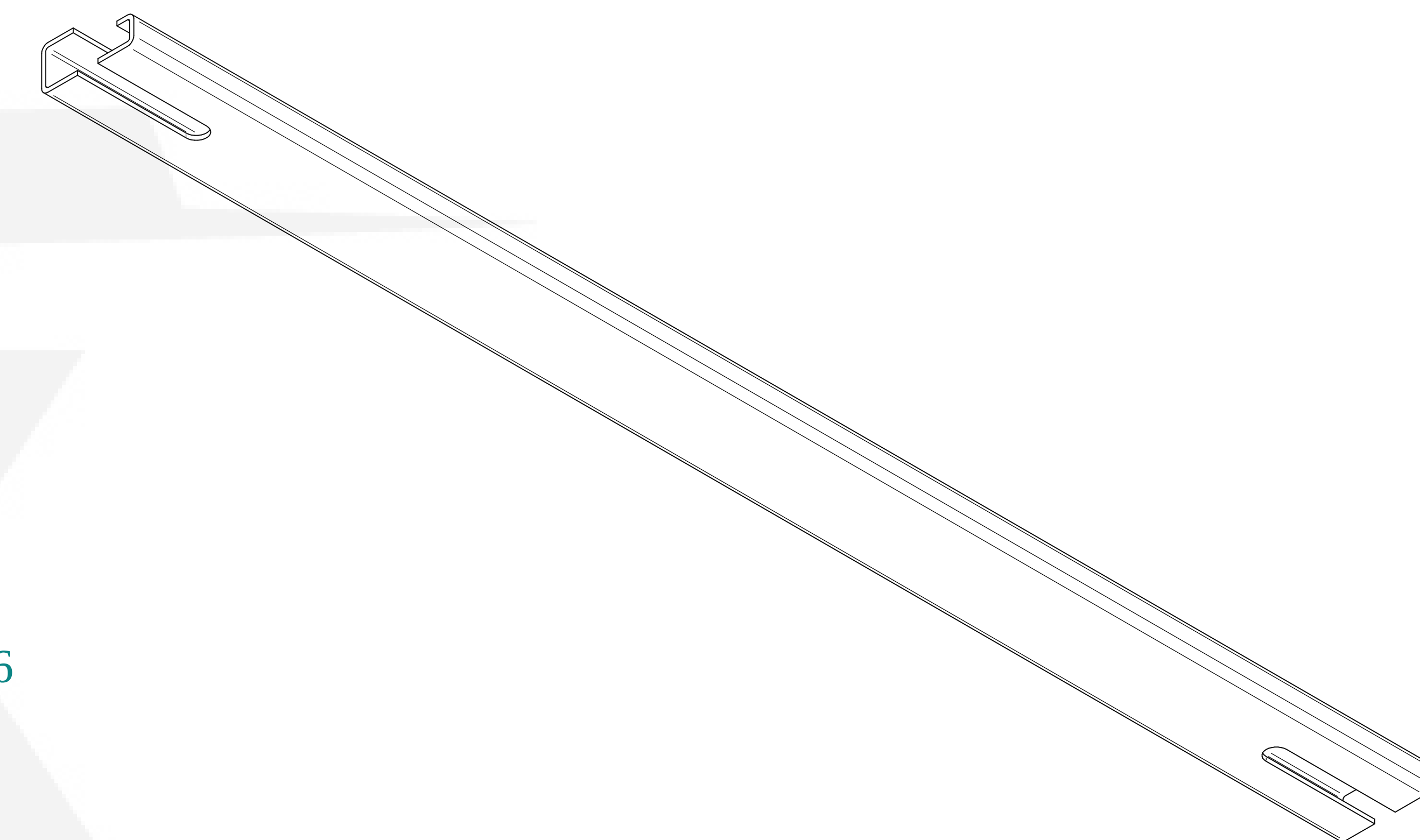
ISOMETRIC VIEWS
