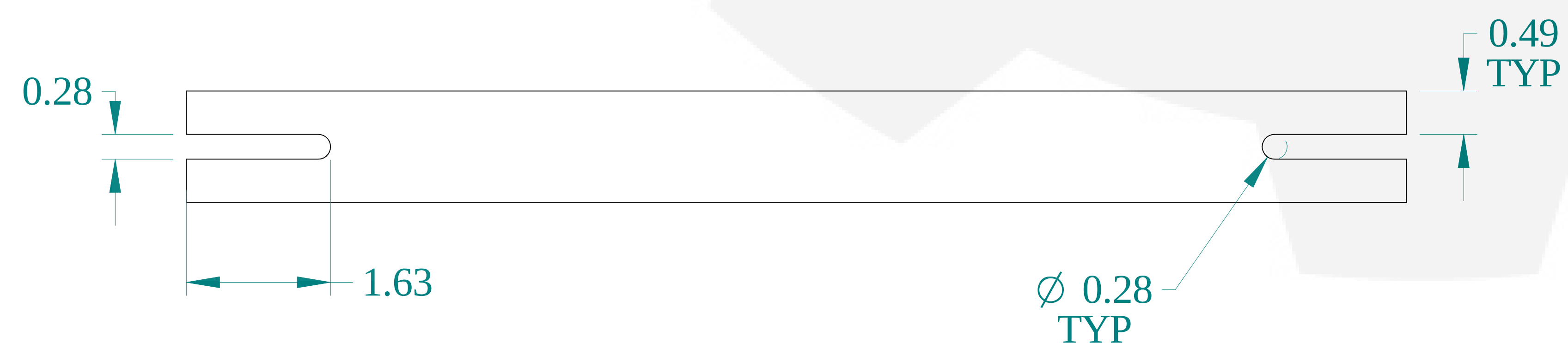
BOTTOM VIEW
