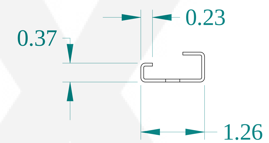
SIDE VIEW
