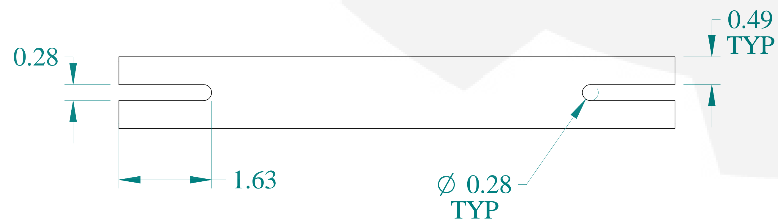
BOTTOM VIEW
