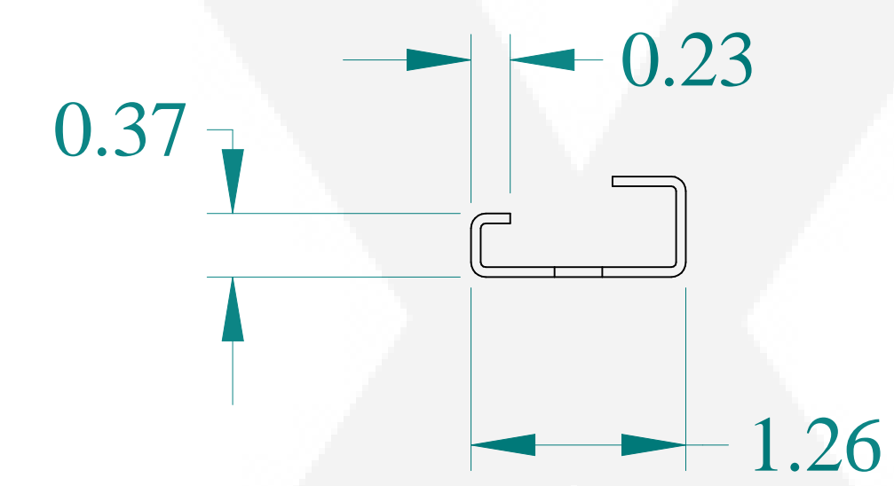
SIDE VIEW
