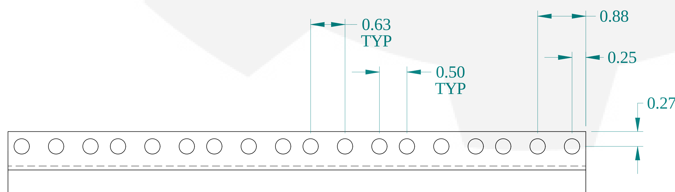
BOTTOM VIEW
