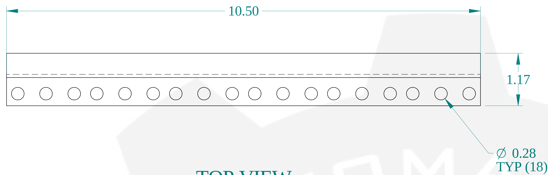
TOP VIEW
