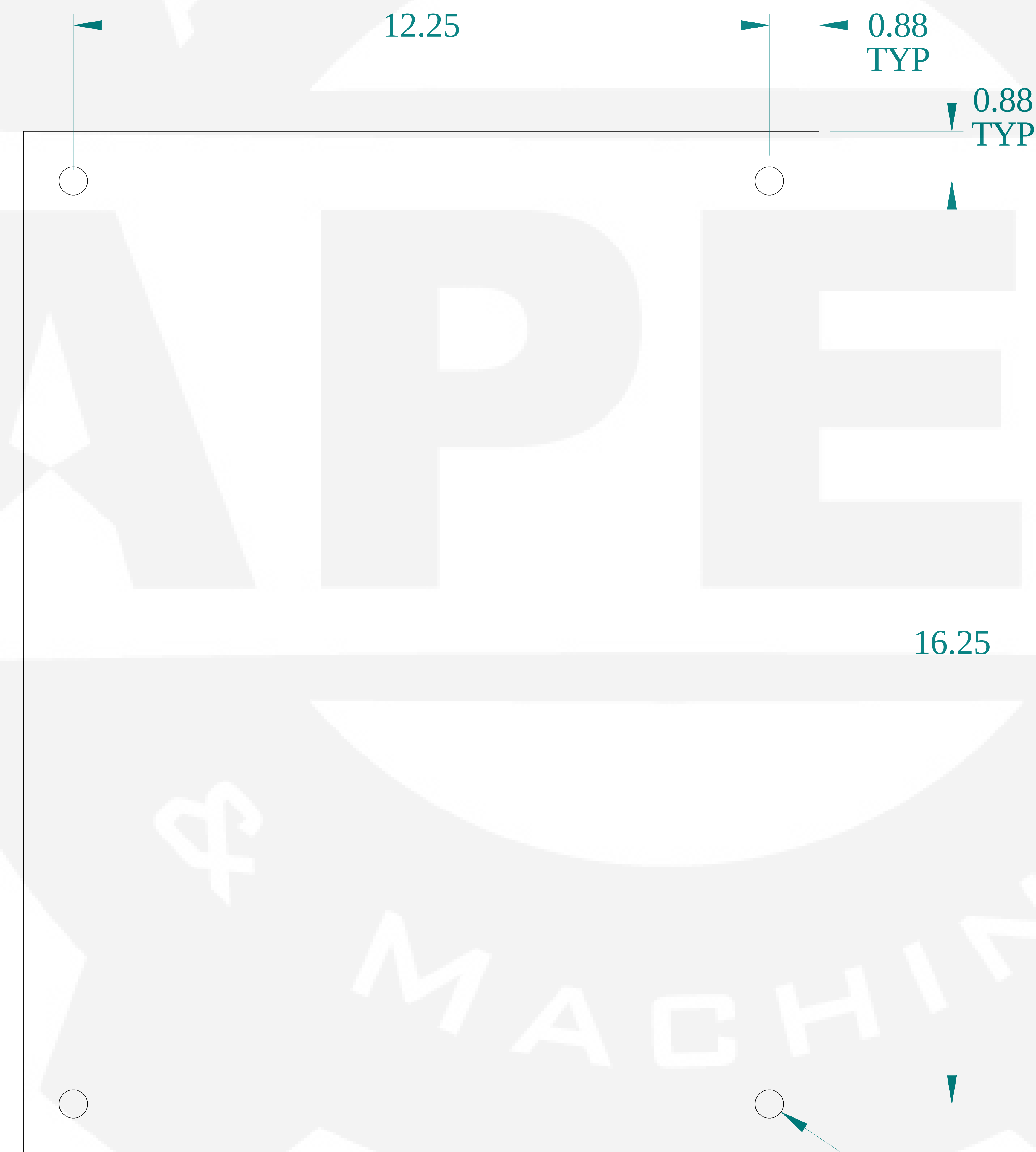
FRONT VIEW
