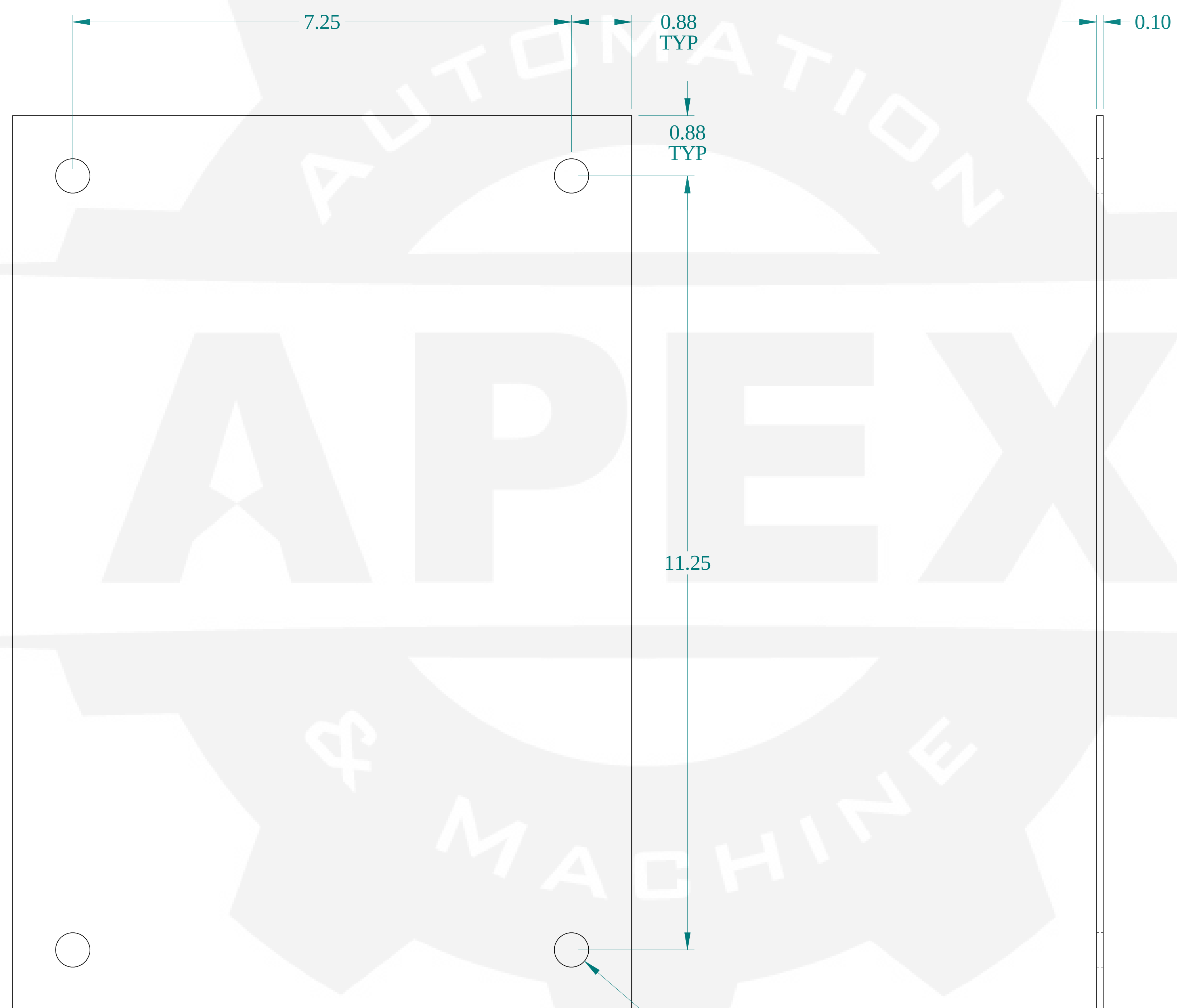
FRONT VIEW
