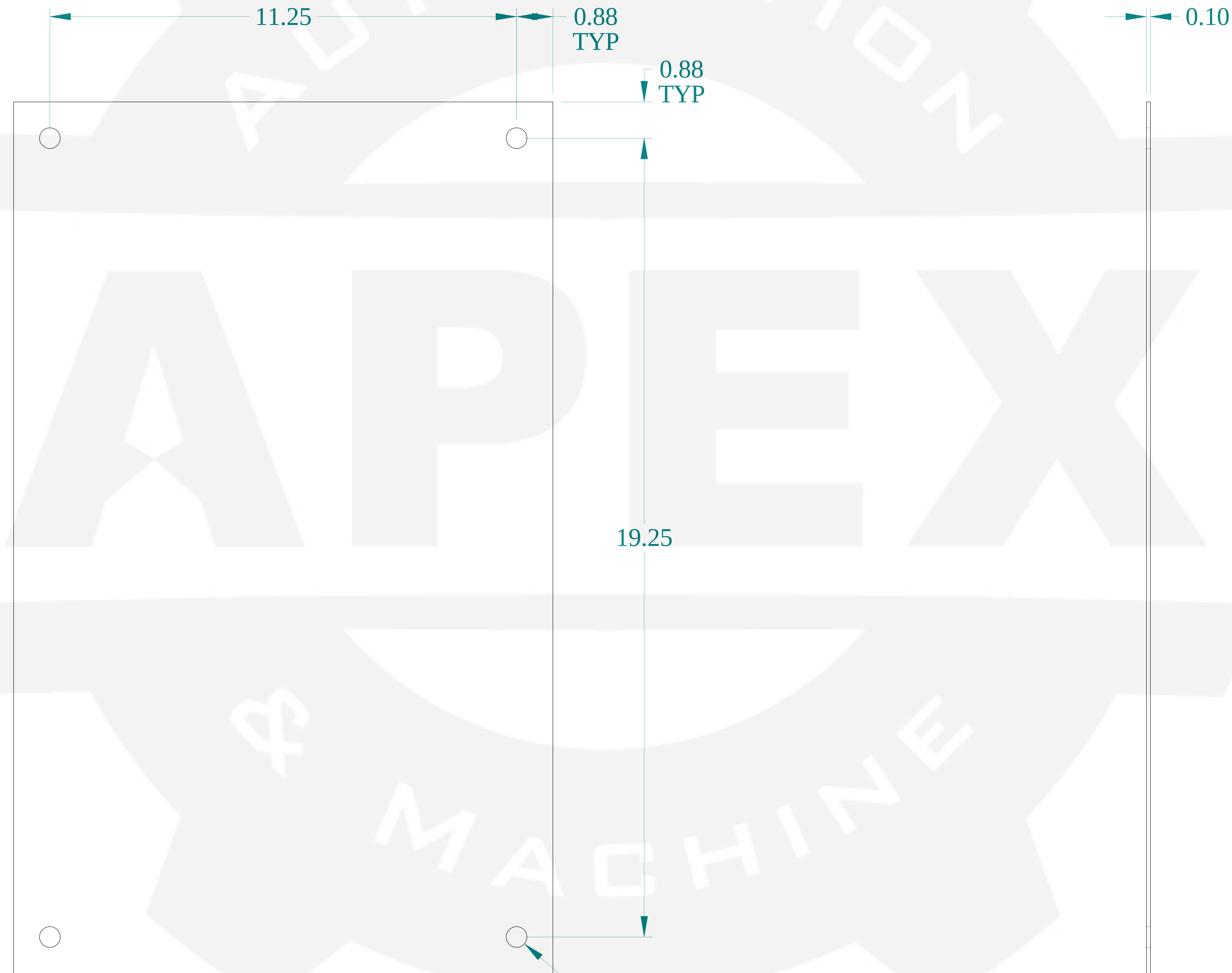
FRONT VIEW
