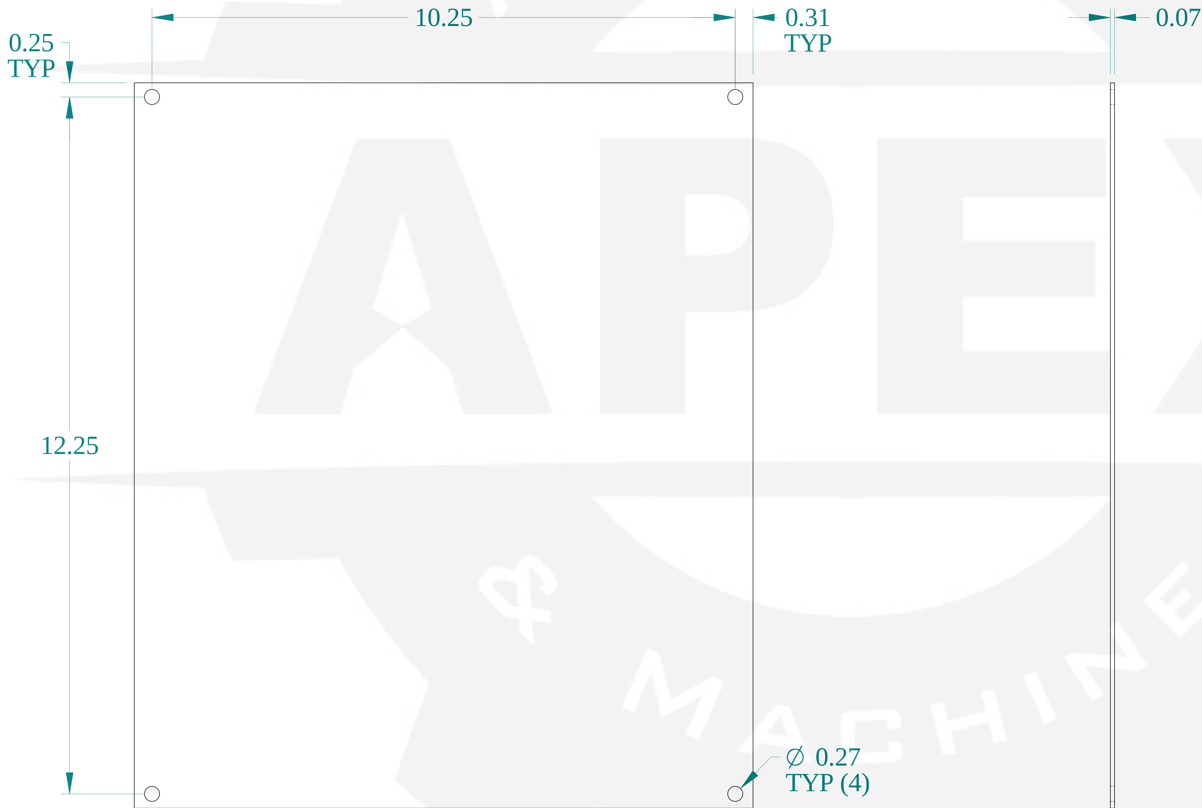
FRONT VIEW
