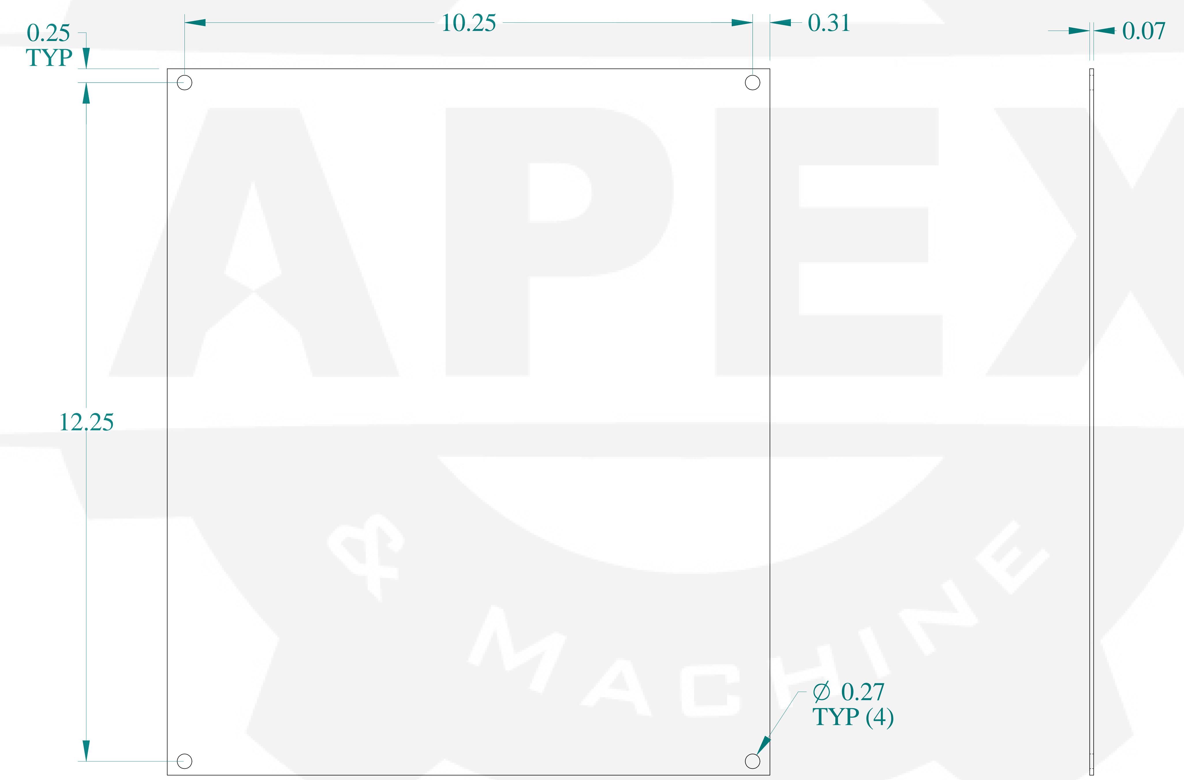
FRONT VIEW
