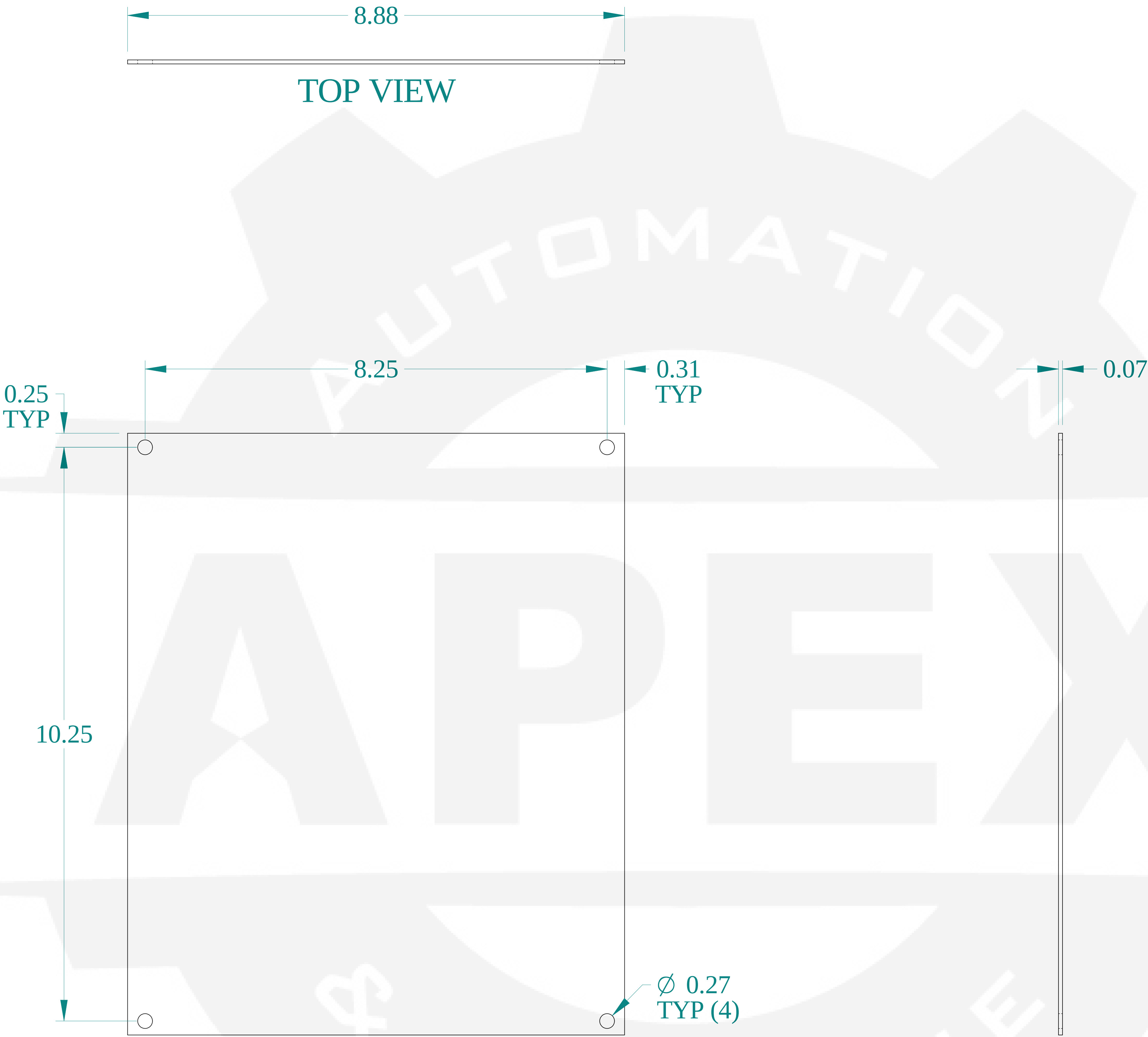
SIDE VIEW
