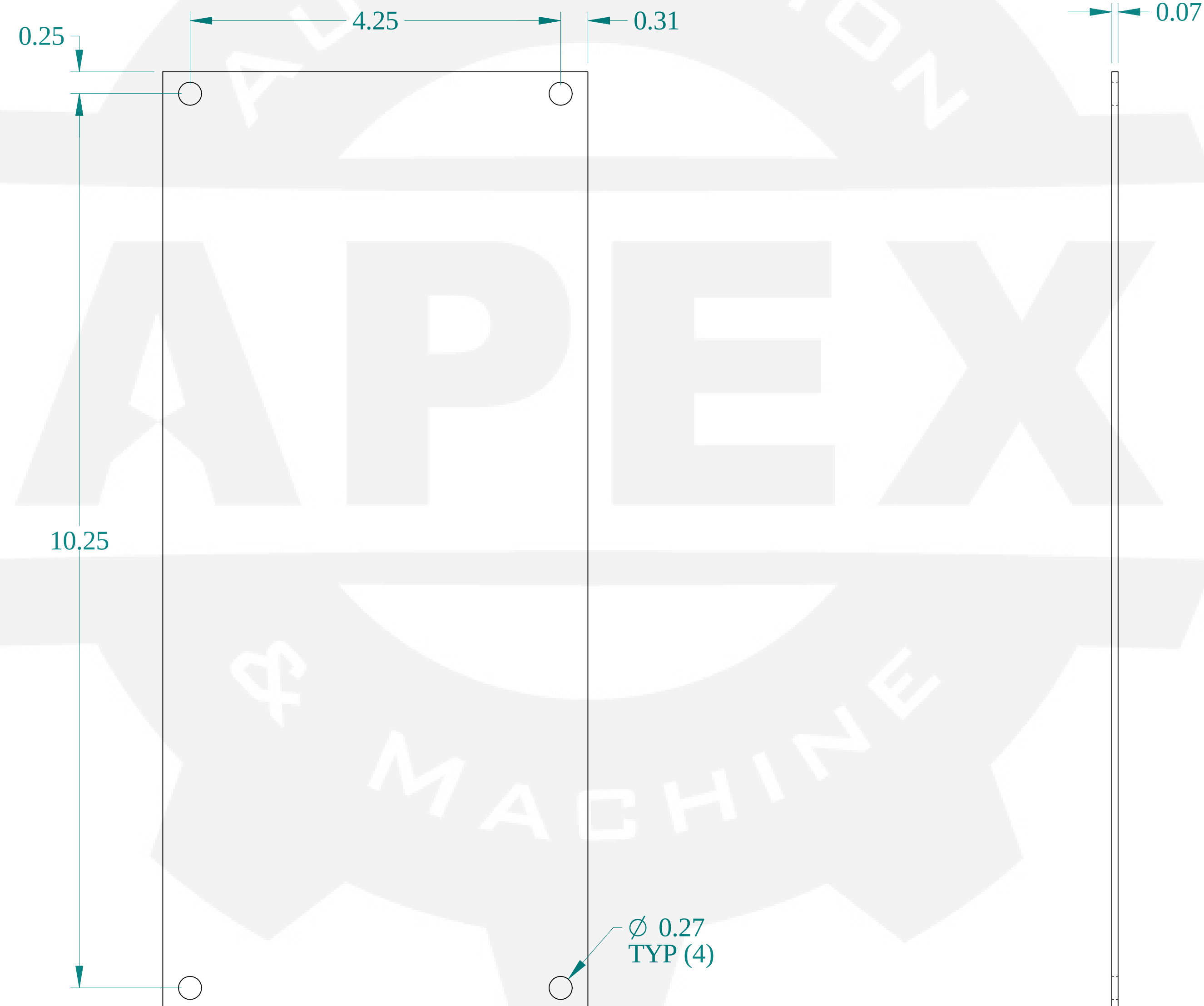
FRONT VIEW
