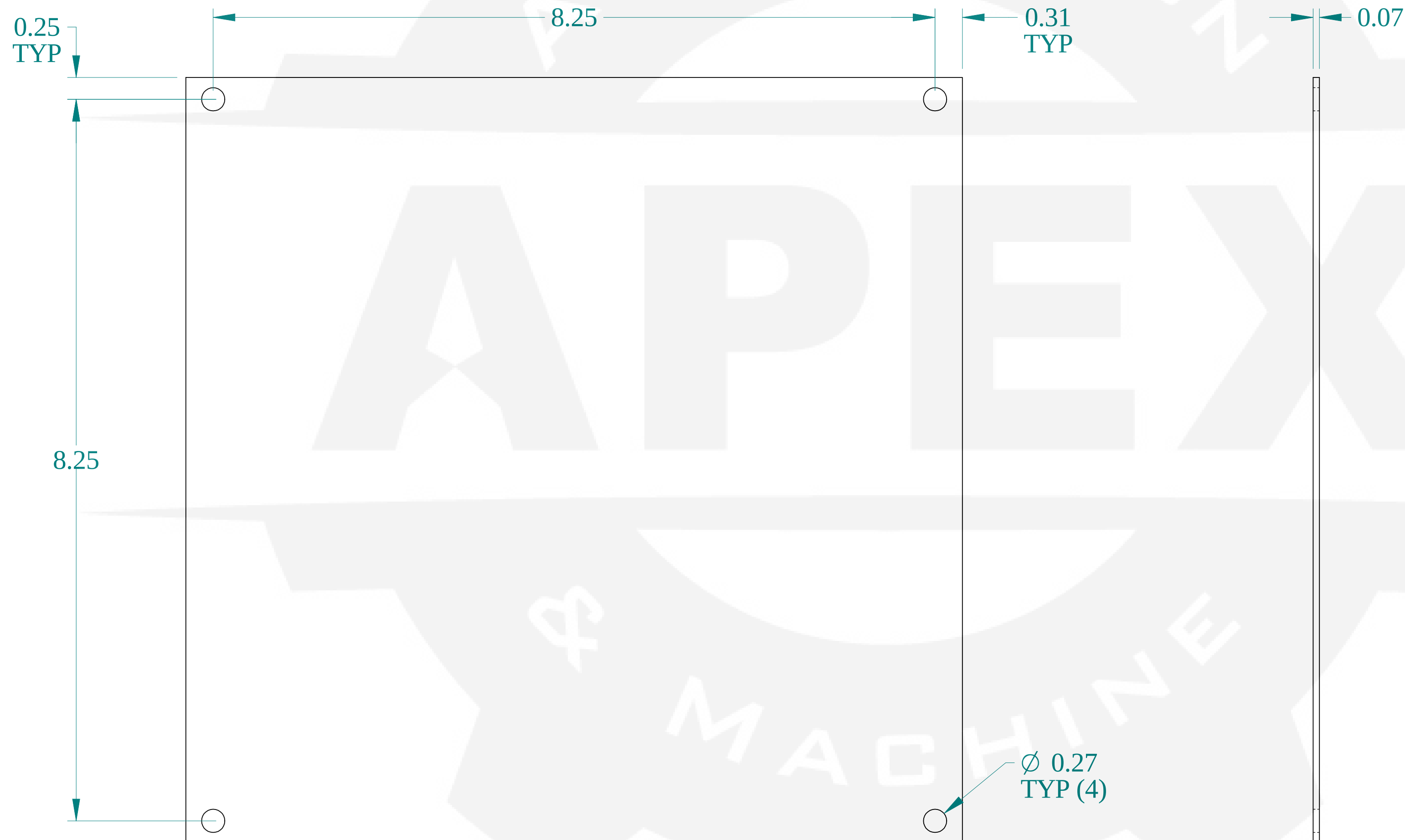
FRONT VIEW
