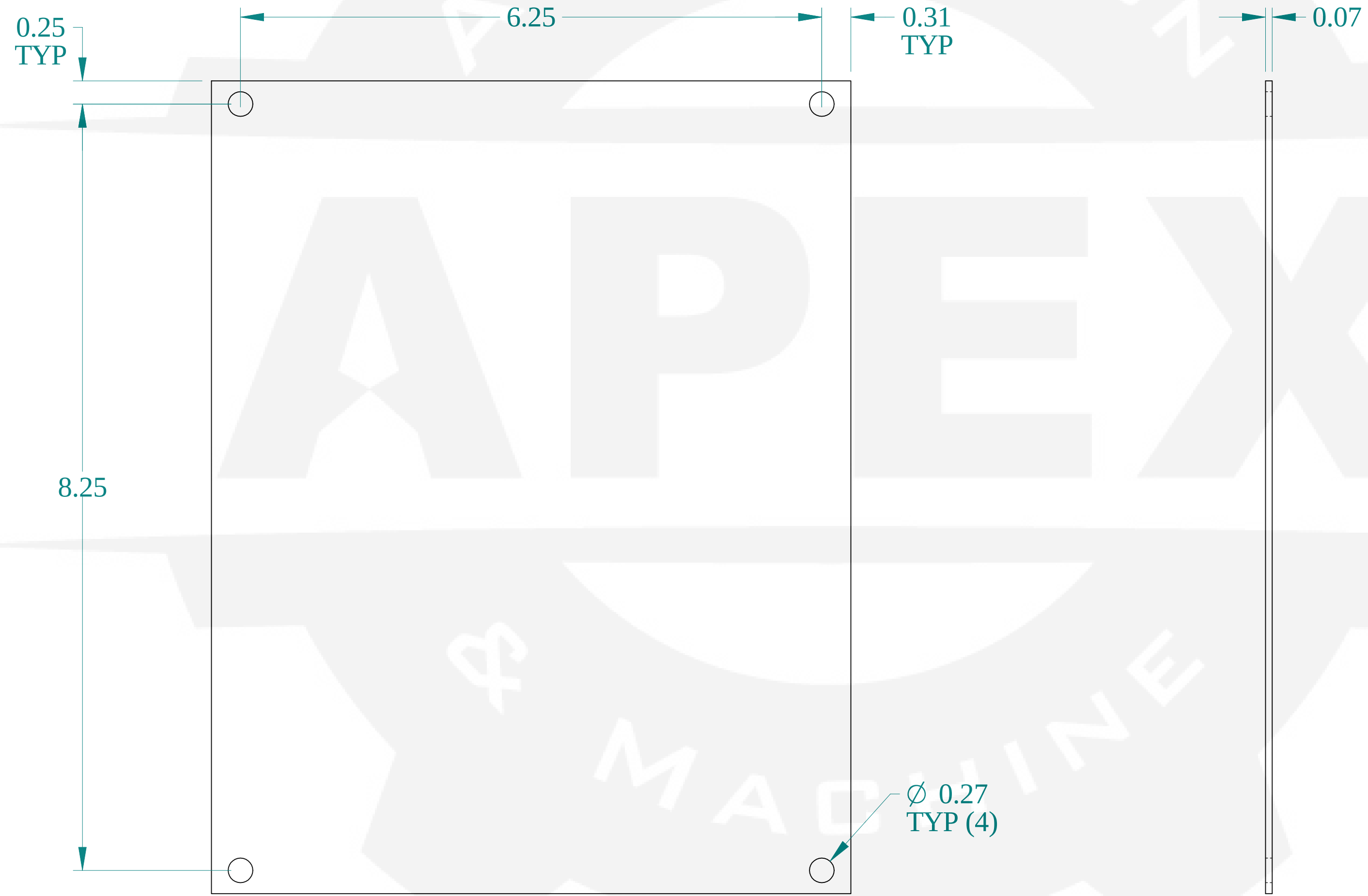
FRONT VIEW
