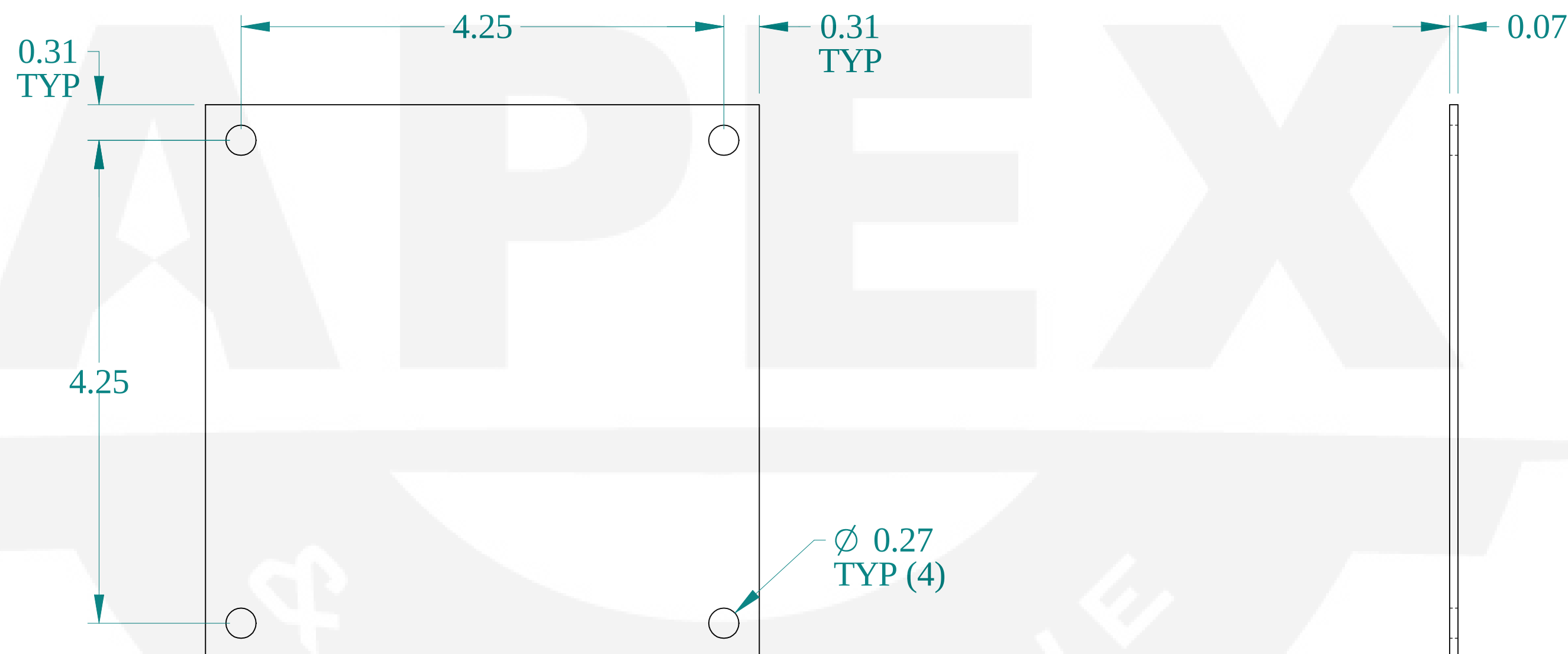
FRONT VIEW
