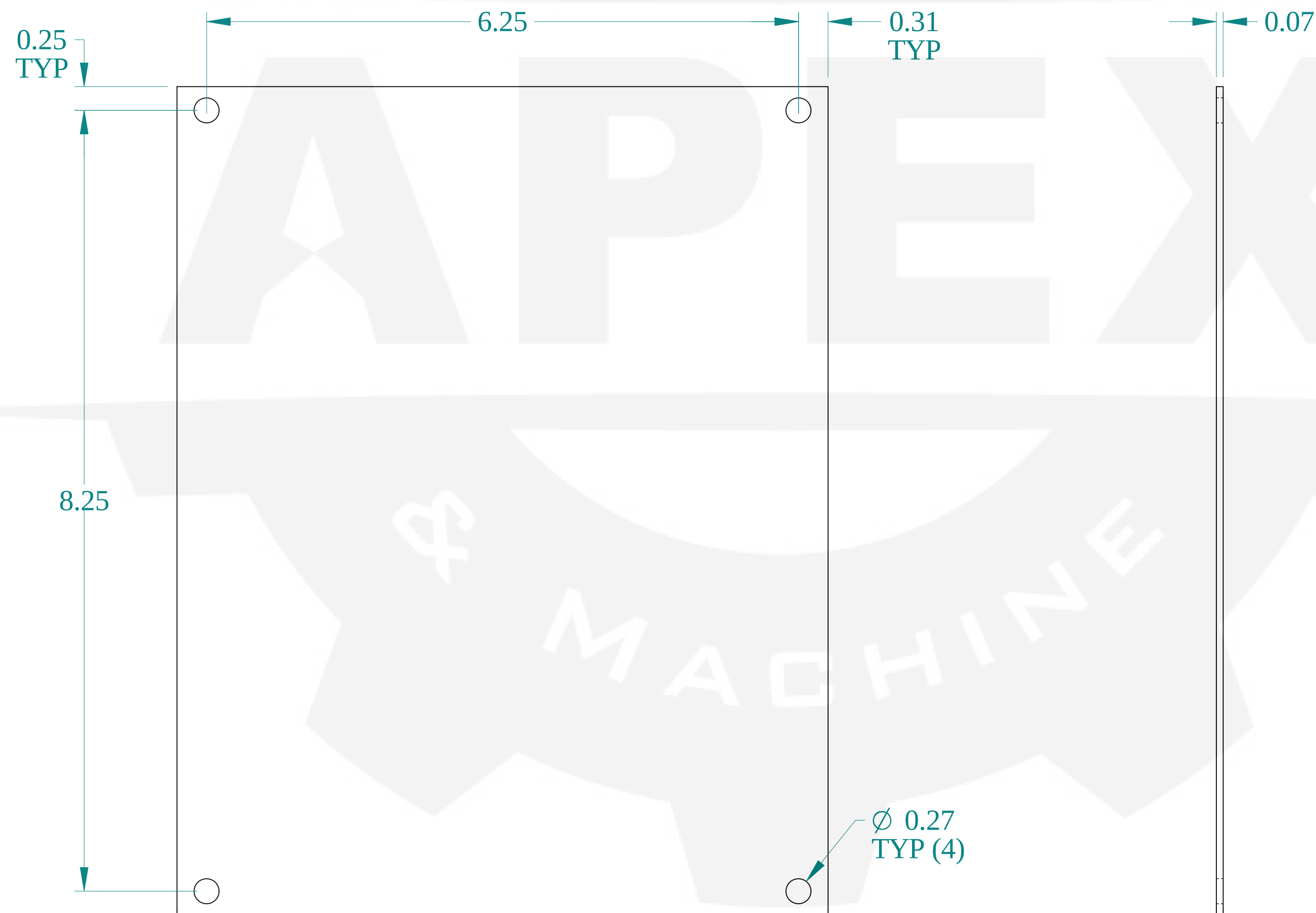
FRONT VIEW
