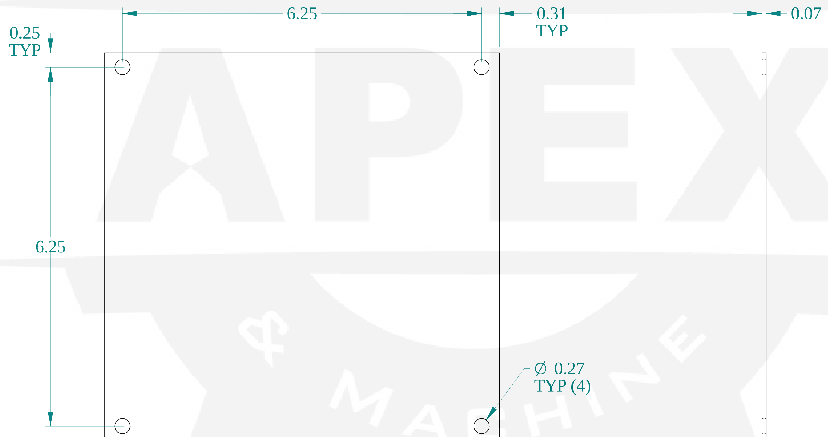
FRONT VIEW
