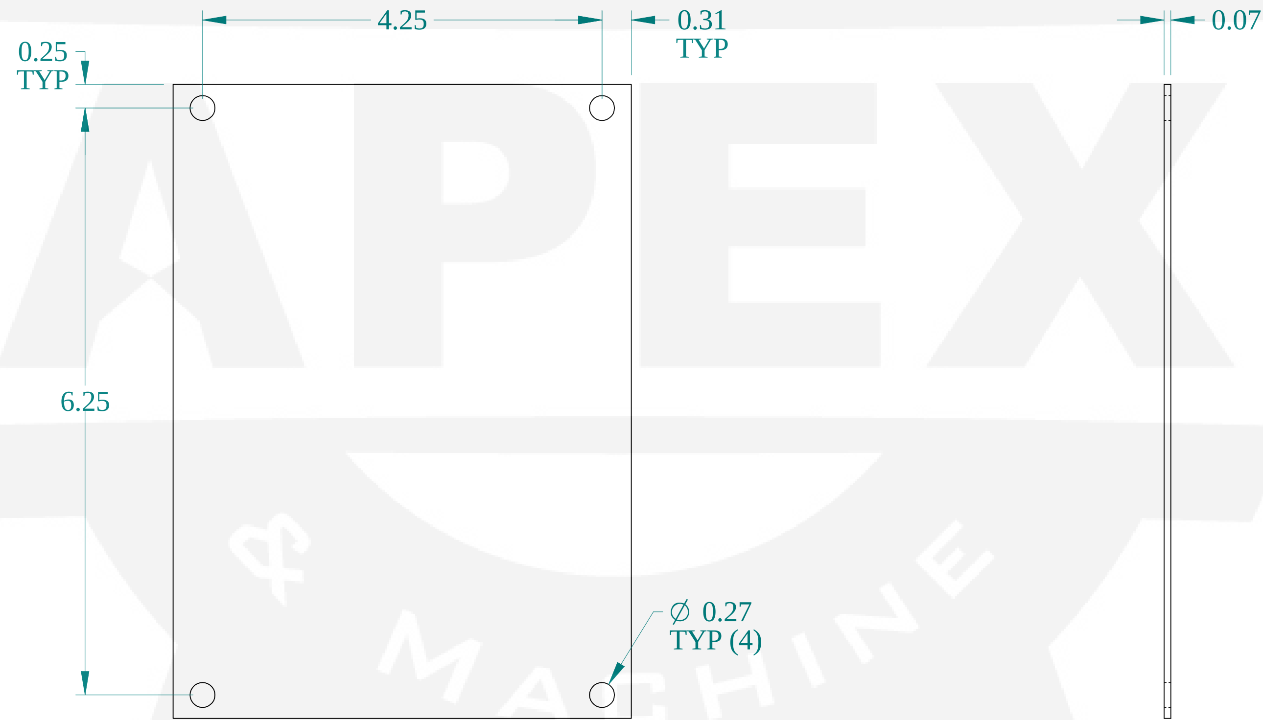
FRONT VIEW
