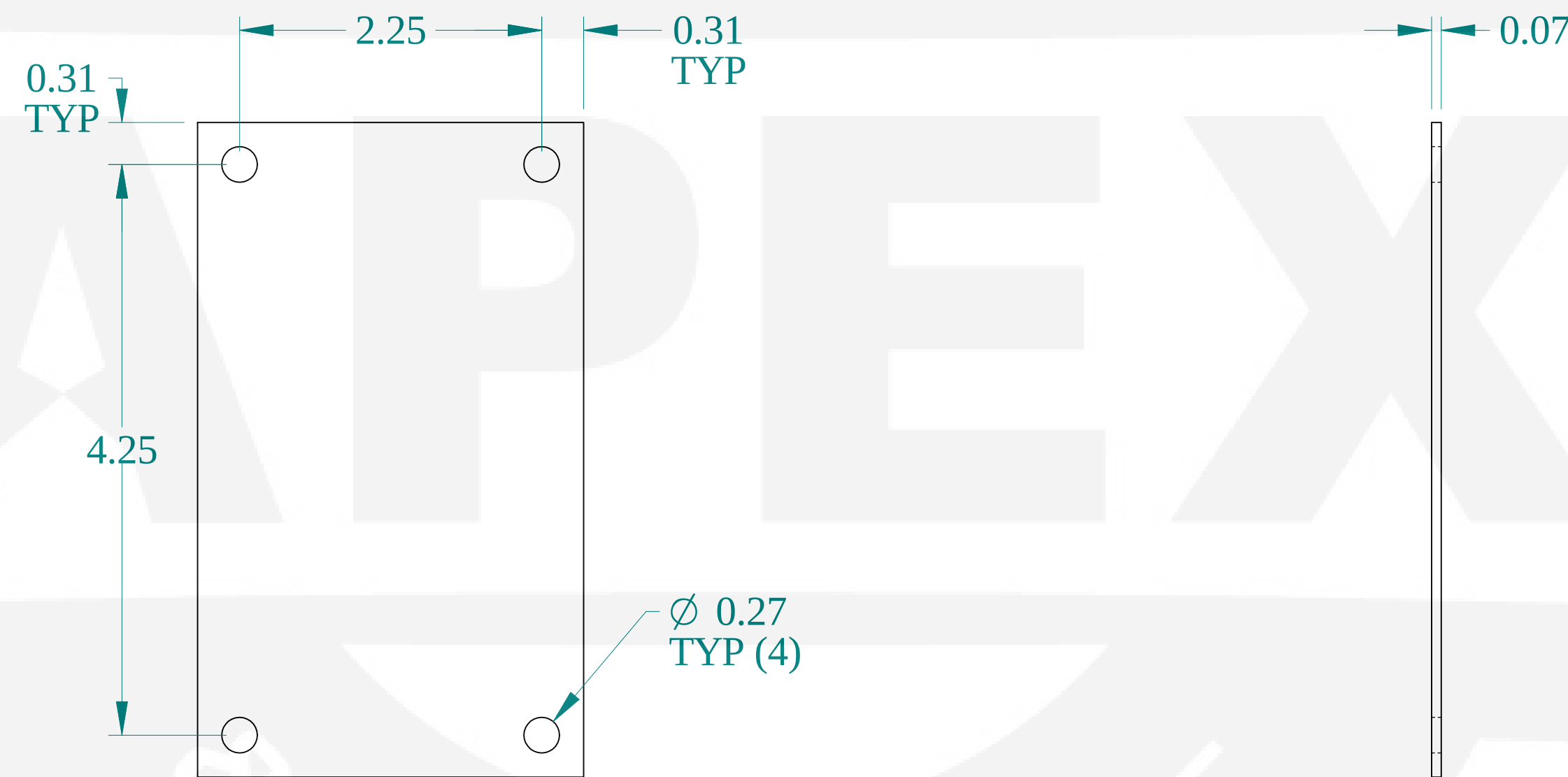
FRONT VIEW
