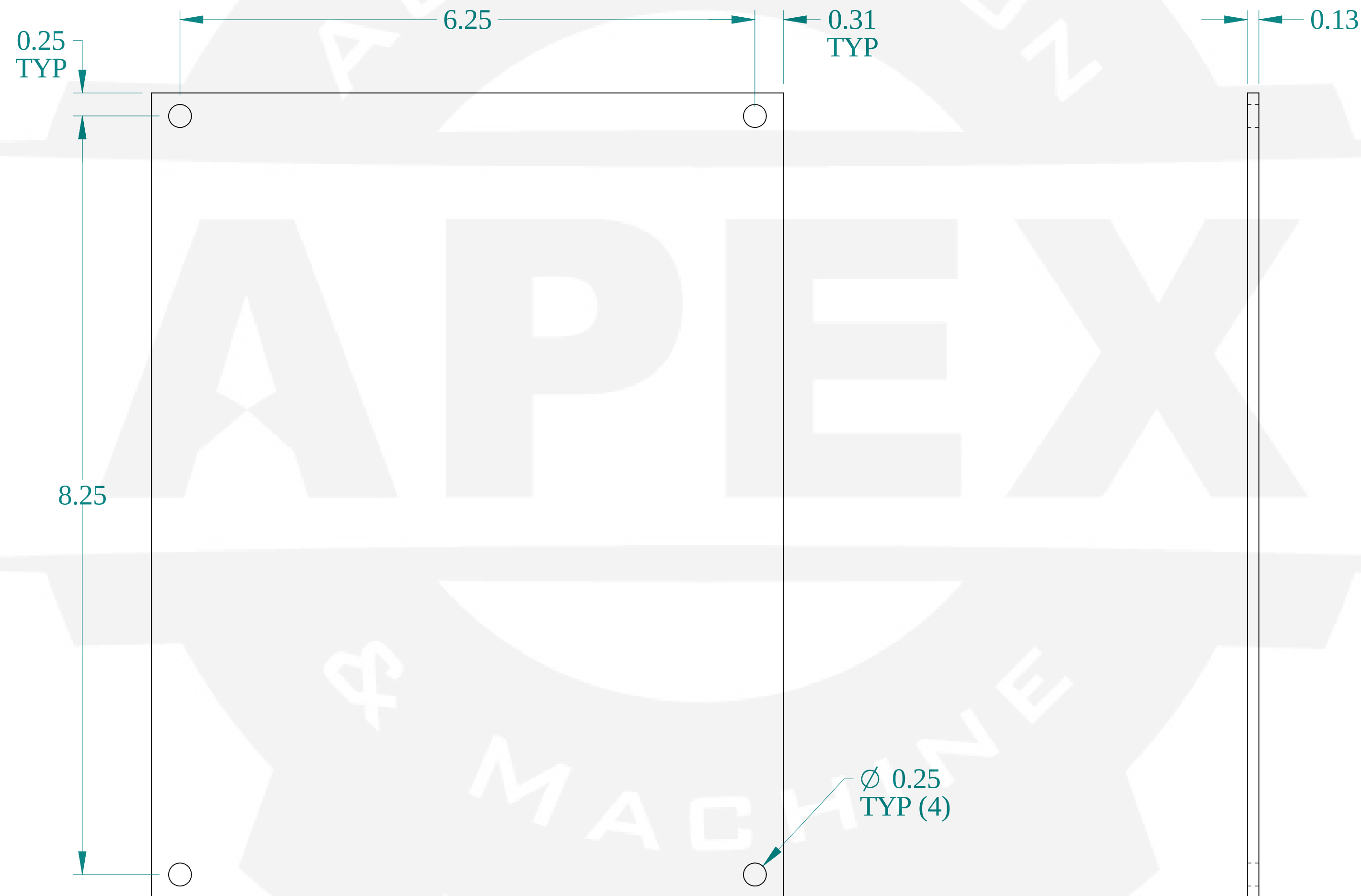
FRONT VIEW
