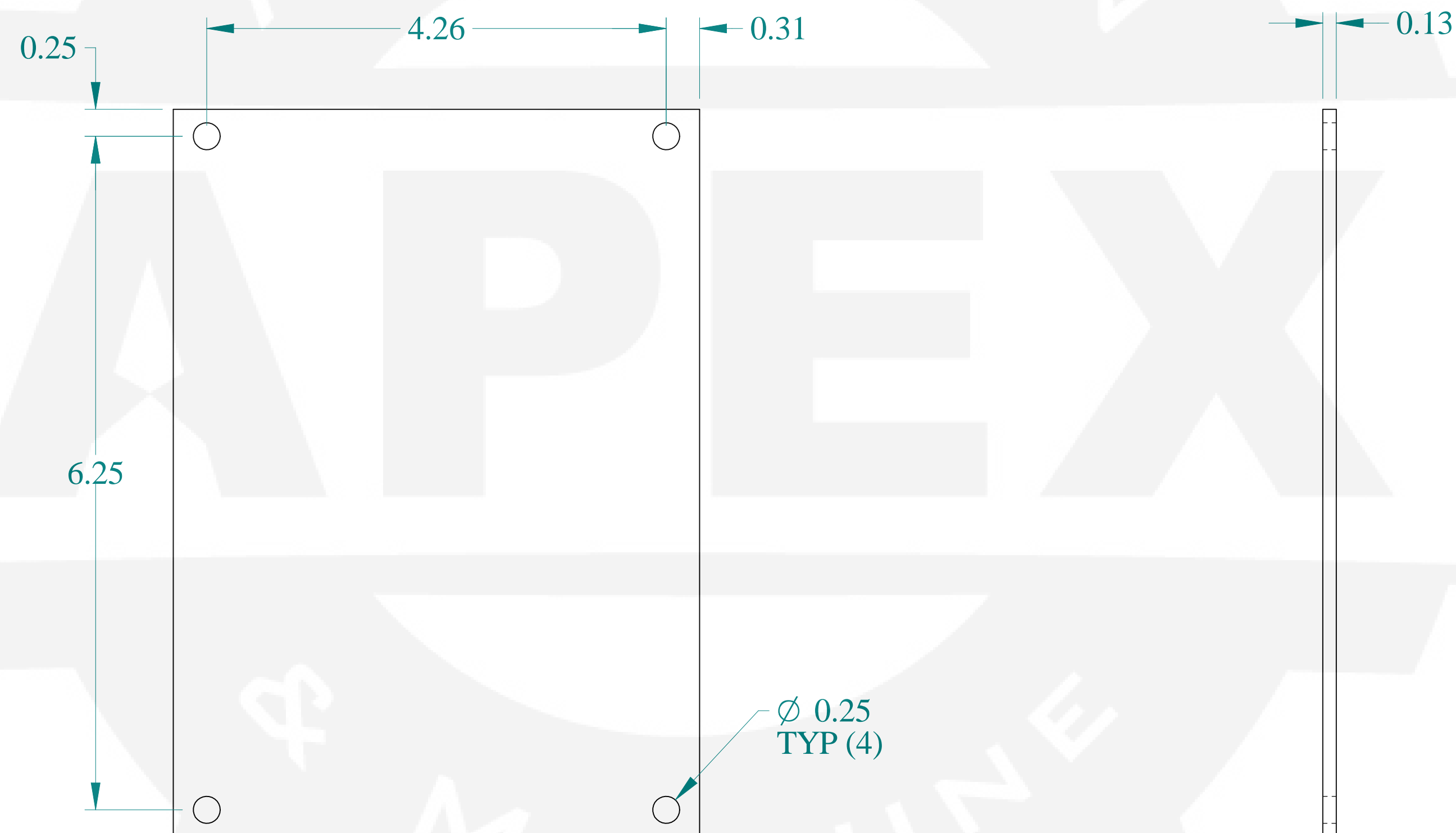
FRONT VIEW
